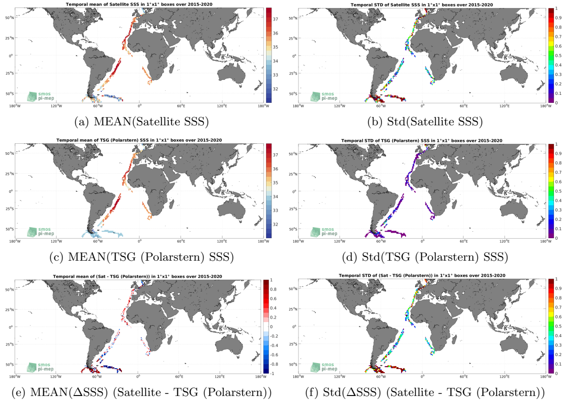
Figure 6: Temporal mean (left) and Std (right) of SSS from SMAP SSS L2 v5.0 (JPL) (top), TSG (Polarstern) (middle), and of \Delta SSS (Satellite - TSG (Polarstern)). Only match-up pairs are used to generate these maps.
