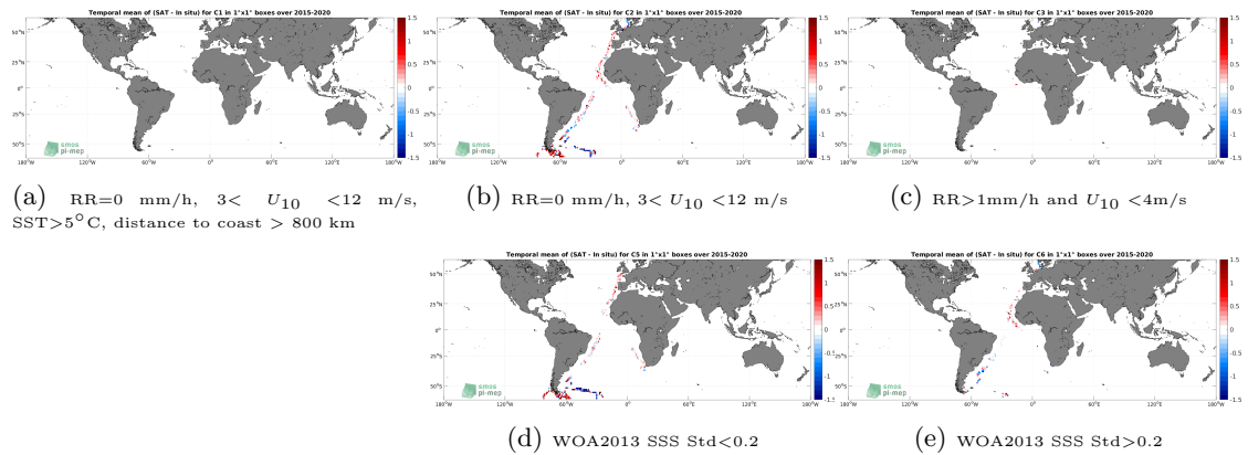
Figure 12: Temporal mean gridded over spatial boxes of size 1^\circ \times 1^\circ of \Delta SSS (SMAP SSS L2 v5.0 (JPL) - TSG (Polarstern)) for 5 different subdatasets corresponding to:RR=0 mm/h, 3 < U_{10} < 12 m/s, SST >5^\circ\text{C} , distance to coast > 800 km (a), RR=0 mm/h, 3 < U_{10} < 12 m/s (b), RR >1 mm/h and U_{10} < 4 m/s (c), WOA2013 SSS Std <0.2 (d), WOA2013 SSS Std >0.2 (e).
