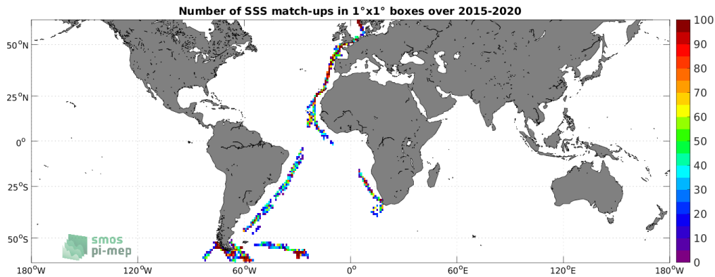
Figure 4: Number of SSS match-ups between TSG (Polarstern) SSS and the SMAP SSS L2 v5.0 (JPL) SSS product for the SMOS coastal zone (<800km) 60N-60S Pi-MEP region over 1^\circ \times 1^\circ boxes and for the full satellite product period.
