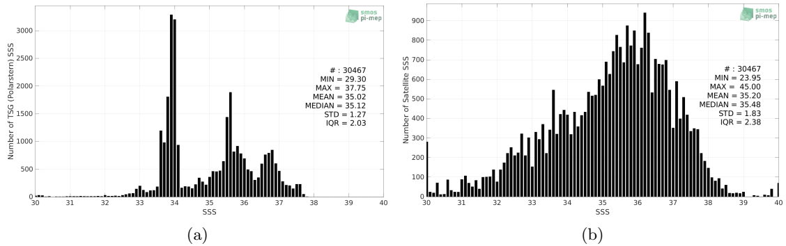
Figure 2: Histograms of SSS from TSG (Polarstern) (a) and SMAP SSS L2 v5.0 (JPL) (b) considering all match-up pairs per bins of 0.1 over the SMOS coastal zone (<800km) 60N-60S Pi-MEP region and for the full satellite product period.
