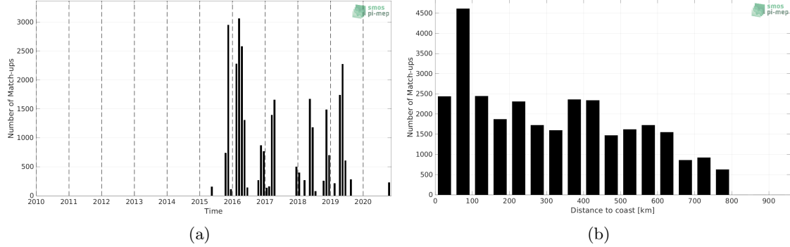
Figure 1: Number of match-ups between TSG (Polarstern) and SMAP SSS L2 v5.0 (JPL) SSS as a function of time (a) and as function of the distance to coast (b) over the SMOS coastal zone (<800km) 60N-60S Pi-MEP region and for the full satellite product period.
