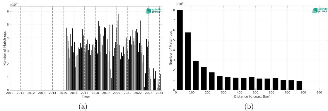
Figure 2: Number of match-ups between TSG (LEGOS-DM) and SMAP SSS L2 v5.0 (JPL) SSS as a function of time (a) and as function of the distance to coast (b) over the SMOS coastal zone (<800km) 60N-60S Pi-MEP region and for the full satellite product period.
