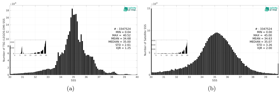
Figure 3: Histograms of SSS from TSG (LEGOS-DM) (a) and SMAP SSS L2 v5.0 (JPL) (b) considering all match-up pairs per bins of 0.1 over the SMOS coastal zone (<800km) 60N-60S Pi-MEP region and for the full satellite product period.
