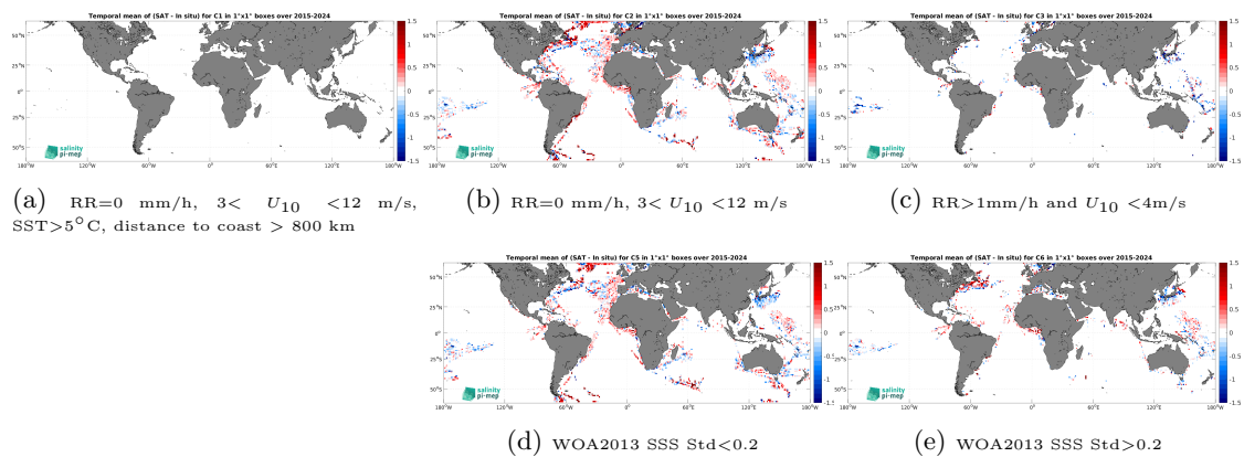
Figure 14: Temporal mean gridded over spatial boxes of size 1^\circ \times 1^\circ of \Delta SSS (SMAP SSS L2 v5.0 (JPL) - TSG (LEGOS-DM)) for 5 different subdatasets corresponding to:RR=0 mm/h, 3 < U_{10} < 12 m/s, SST >5^\circ\text{C} , distance to coast > 800 km (a), RR=0 mm/h, 3 < U_{10} < 12 m/s (b), RR >1 mm/h and U_{10} < 4 m/s (c), WOA2013 SSS Std <0.2 (d), WOA2013 SSS Std >0.2 (e).
