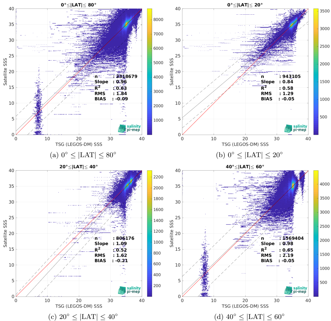
Figure 10: Contour maps of the concentration of SMAP SSS L2 v5.0 (JPL) SSS (y-axis) versus TSG (LEGOS-DM) SSS (x-axis) at match-up pairs for different latitude bands. For each plot, the red line shows x=y . The black thin and dashed lines indicate a linear fit through the data cloud and the \pm 95\% confidence levels, respectively. The number match-up pairs n , the slope and R^2 coefficient of the linear fit, the root mean square (RMS) and the mean bias between satellite and in situ data are indicated for each latitude band in each plots.
