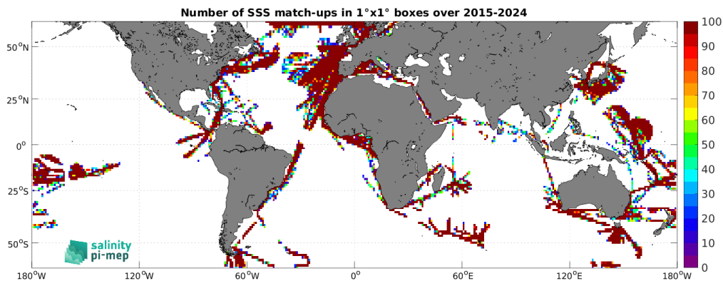
Figure 5: Number of SSS match-ups between TSG (LEGOS-DM) SSS and the SMAP SSS L2 v5.0 (JPL) SSS product for the SMOS coastal zone (<800km) 60N-60S Pi-MEP region over 1^\circ \times 1^\circ boxes and for the full satellite product period.
