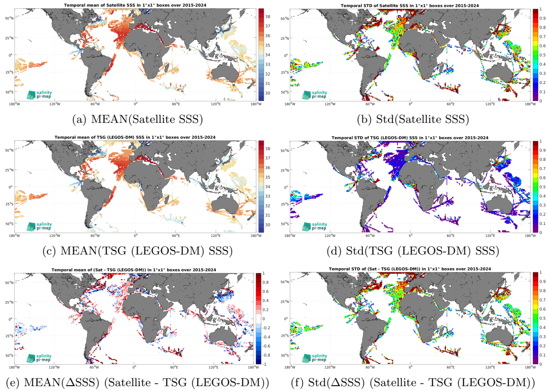
Figure 7: Temporal mean (left) and Std (right) of SSS from SMAP SSS L2 v5.0 (JPL) (top), TSG (LEGOS-DM) (middle), and of \Delta SSS (Satellite - TSG (LEGOS-DM)). Only match-up pairs are used to generate these maps.
