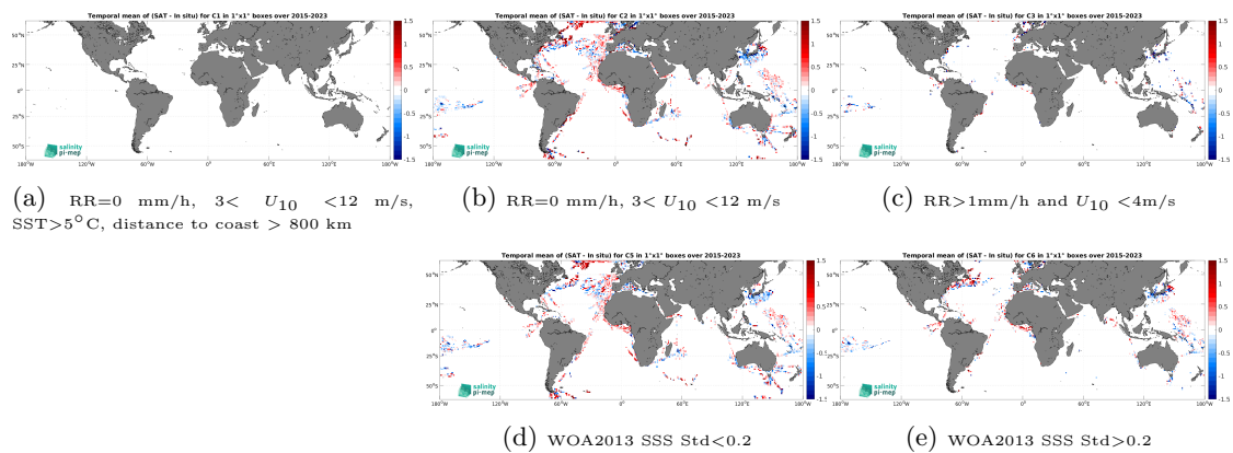
Figure 14: Temporal mean gridded over spatial boxes of size 1^\circ \times 1^\circ of \Delta\text{SSS} (SMAP SSS L2 v5.0 (JPL) - TSG (LEGOS-DM)) for 5 different subdatasets corresponding to: RR=0 mm/h, 3 < U_{10} < 12 m/s, SST > 5^\circ\text{C} , distance to coast > 800 km (a), RR=0 mm/h, 3 < U_{10} < 12 m/s (b), RR > 1 mm/h and U_{10} < 4 m/s (c), WOA2013 SSS Std < 0.2 (d), WOA2013 SSS Std > 0.2 (e).
