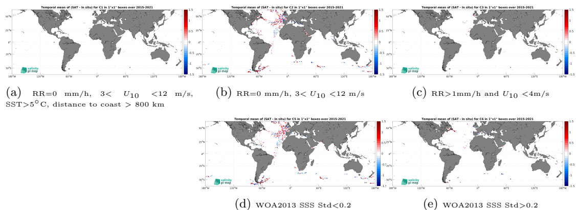
Figure 14: Temporal mean gridded over spatial boxes of size 1^\circ \times 1^\circ of \Delta\text{SSS} (SMAP SSS L2 v5.0 (JPL) - TSG (GOSUD-Sailing-ship)) for 5 different subdatasets corresponding to: RR=0 mm/h, 3 < U_{10} < 12 m/s, SST > 5°C, distance to coast > 800 km (a), RR=0 mm/h, 3 < U_{10} < 12 m/s (b), RR > 1mm/h and U_{10} < 4 m/s (c), WOA2013 SSS Std < 0.2 (d), WOA2013 SSS Std > 0.2 (e).
