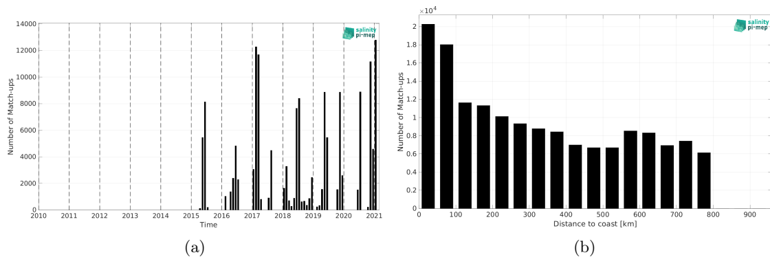
Figure 2: Number of match-ups between TSG (GOSUD-Sailing-ship) and SMAP SSS L2 v5.0 (JPL) SSS as a function of time (a) and as function of the distance to coast (b) over the SMOS coastal zone (<800km) 60N-60S Pi-MEP region and for the full satellite product period.
