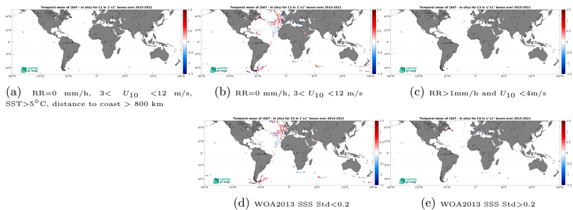
Figure 12: Temporal mean gridded over spatial boxes of size 1^\circ \times 1^\circ of \Delta\text{SSS} (SMAP SSS L2 v5.0 (JPL) - TSG (GOSUD-Sailing-ship)) for 5 different subdatasets corresponding to:RR=0 mm/h, 3 < U_{10} < 12 m/s, SST >5^\circ\text{C} , distance to coast > 800 km (a), RR=0 mm/h, 3 < U_{10} < 12 m/s (b), RR >1 mm/h and U_{10} < 4 m/s (c), WOA2013 SSS Std <0.2 (d), WOA2013 SSS Std >0.2 (e).
