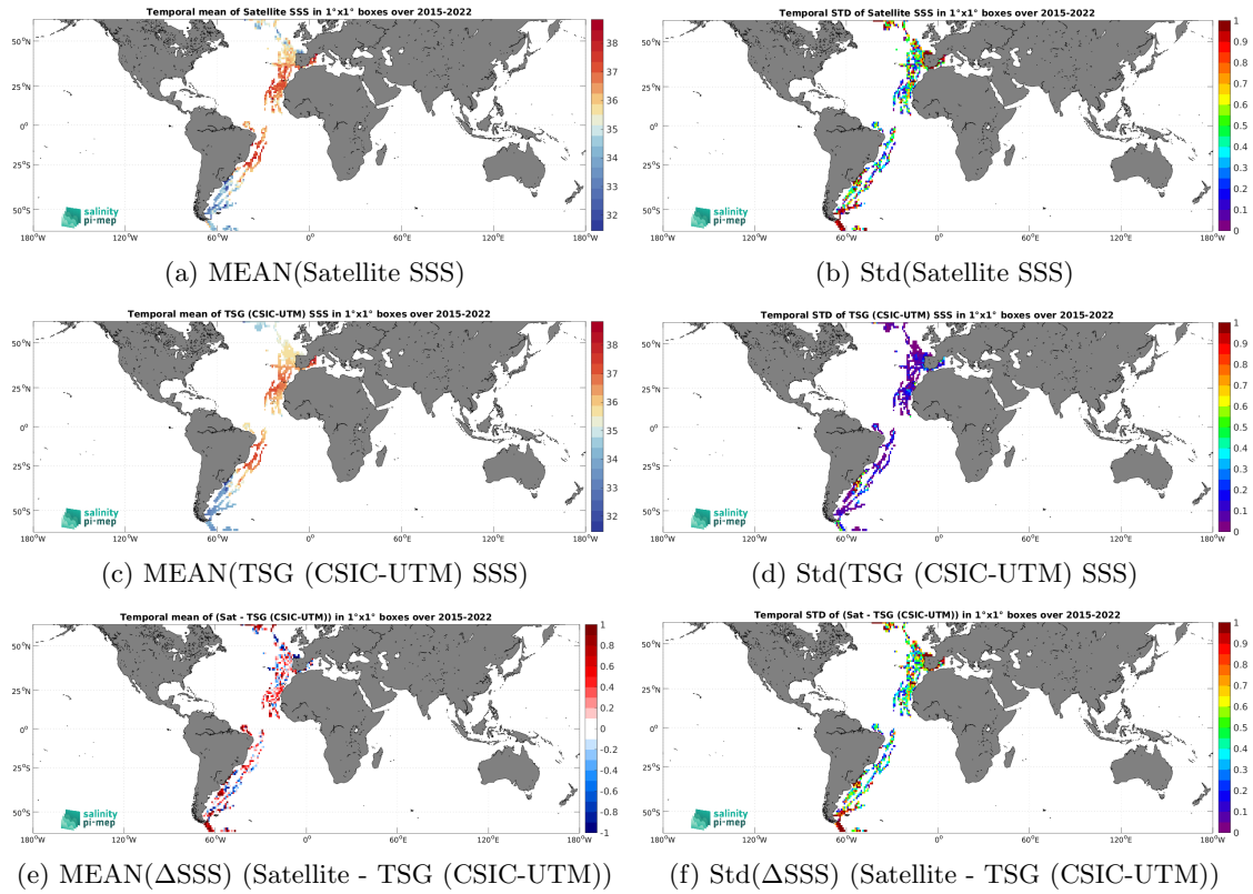
Figure 6: Temporal mean (left) and Std (right) of SSS from SMAP SSS L2 v5.0 (JPL) (top), TSG (CSIC-UTM) (middle), and of \Delta SSS (Satellite - TSG (CSIC-UTM)). Only match-up pairs are used to generate these maps.
