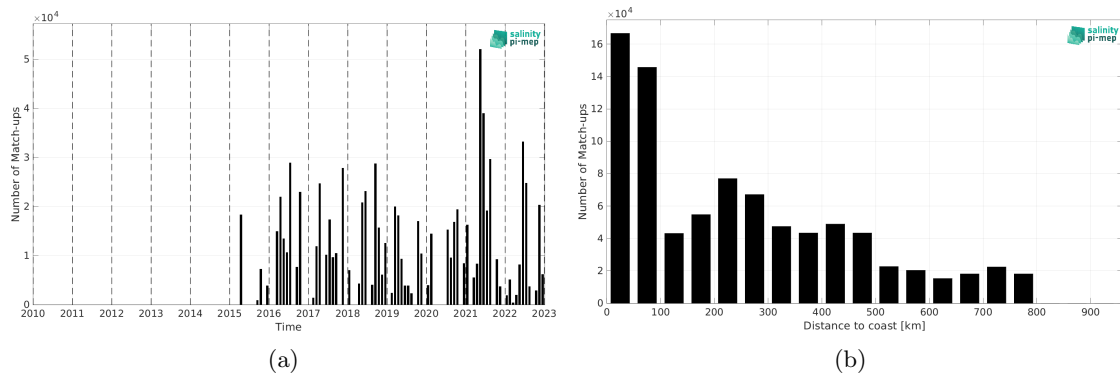
Figure 1: Number of match-ups between TSG (CSIC-UTM) and SMAP SSS L2 v5.0 (JPL) SSS as a function of time (a) and as function of the distance to coast (b) over the SMOS coastal zone (<800km) 60N-60S Pi-MEP region and for the full satellite product period.
