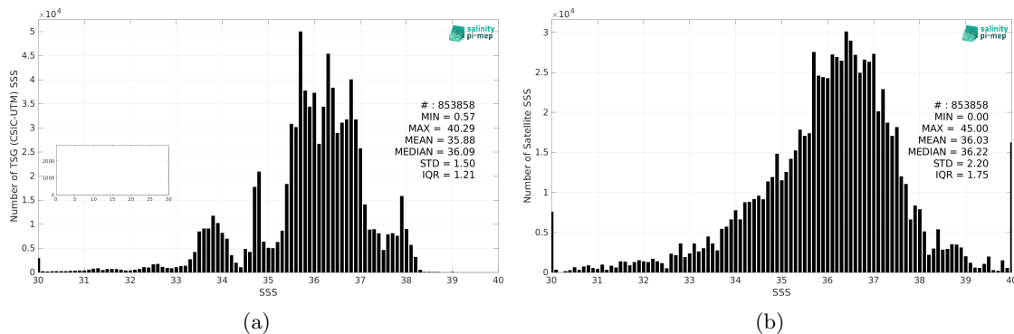
Figure 2: Histograms of SSS from TSG (CSIC-UTM) (a) and SMAP SSS L2 v5.0 (JPL) (b) considering all match-up pairs per bins of 0.1 over the SMOS coastal zone (<800km) 60N-60S Pi-MEP region and for the full satellite product period.
