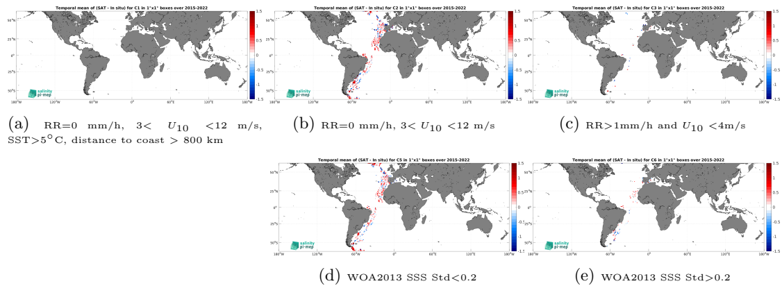
Figure 12: Temporal mean gridded over spatial boxes of size 1^\circ \times 1^\circ of \Delta\text{SSS} (SMAP SSS L2 v5.0 (JPL) - TSG (CSIC-UTM)) for 5 different subdatasets corresponding to:RR=0 mm/h, 3 < U_{10} < 12 m/s, SST >5^\circ\text{C} , distance to coast > 800 km (a), RR=0 mm/h, 3 < U_{10} < 12 m/s (b), RR >1 mm/h and U_{10} < 4 m/s (c), WOA2013 SSS Std <0.2 (d), WOA2013 SSS Std >0.2 (e).
