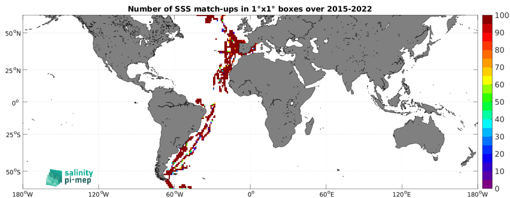
Figure 4: Number of SSS match-ups between TSG (CSIC-UTM) SSS and the SMAP SSS L2 v5.0 (JPL) SSS product for the SMOS coastal zone (<800km) 60N-60S Pi-MEP region over 1^\circ \times 1^\circ boxes and for the full satellite product period.
