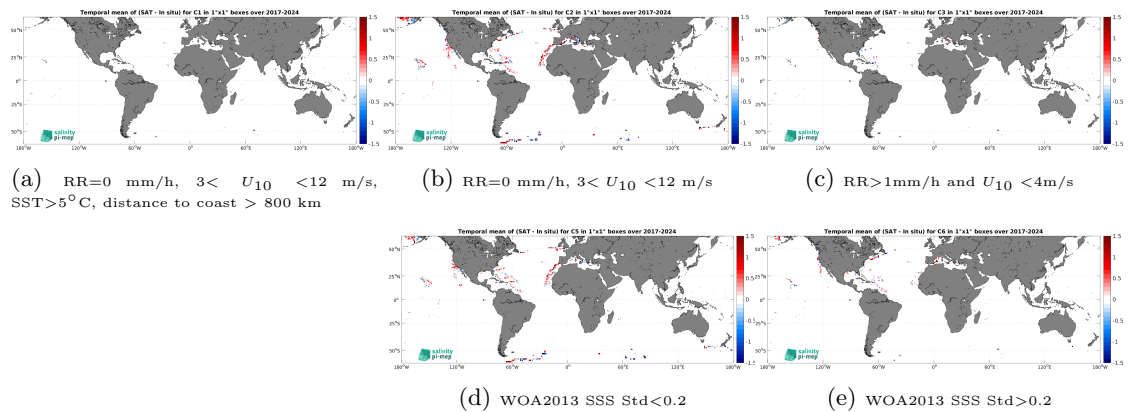
Figure 14: Temporal mean gridded over spatial boxes of size 1^\circ \times 1^\circ of \Delta SSS (SMAP SSS L2 v5.0 (JPL) - Saildrone) for 5 different subdatasets corresponding to:RR=0 mm/h, 3 < U_{10} < 12 m/s, SST >5^\circ\text{C} , distance to coast > 800 km (a), RR=0 mm/h, 3 < U_{10} < 12 m/s (b), RR >1 mm/h and U_{10} < 4 m/s (c), WOA2013 SSS Std <0.2 (d), WOA2013 SSS Std >0.2 (e).
