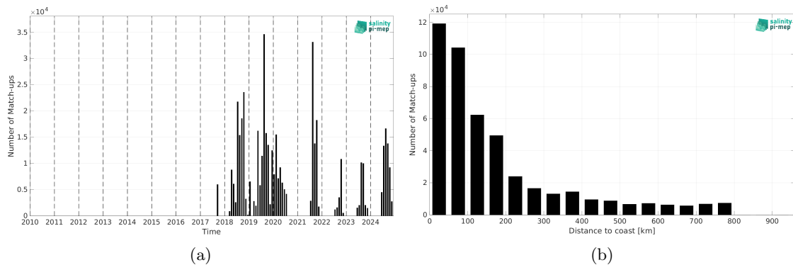
Figure 2: Number of match-ups between Saildrone and SMAP SSS L2 v5.0 (JPL) SSS as a function of time (a) and as function of the distance to coast (b) over the SMOS coastal zone (<800km) 60N-60S Pi-MEP region and for the full satellite product period.
