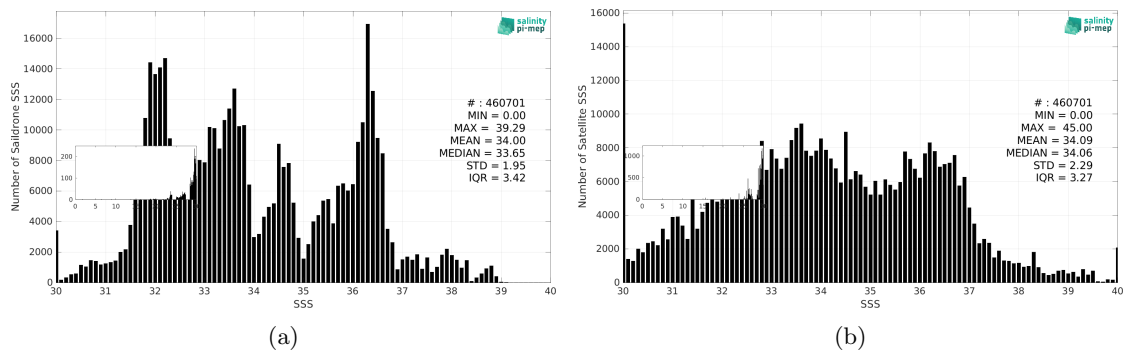
Figure 3: Histograms of SSS from Saildrone (a) and SMAP SSS L2 v5.0 (JPL) (b) considering all match-up pairs per bins of 0.1 over the SMOS coastal zone (<800km) 60N-60S Pi-MEP region and for the full satellite product period.
