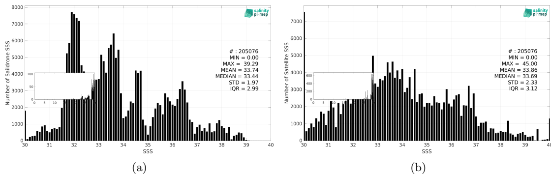
Figure 3: Histograms of SSS from Sairdrone (a) and SMAP SSS L2 v5.0 (JPL) (b) considering all match-up pairs per bins of 0.1 over the SMOS coastal zone (<800km) 60N-60S Pi-MEP region and for the full satellite product period.
