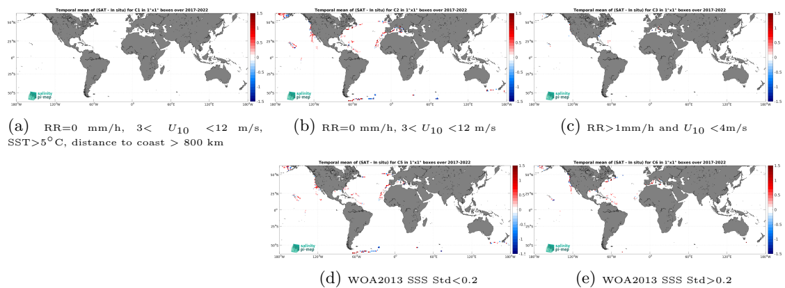
Figure 14: Temporal mean gridded over spatial boxes of size 1^\circ \times 1^\circ of \Delta SSS (SMAP SSS L2 v5.0 (JPL) - Saldrone) for 5 different subdatasets corresponding to:RR=0 mm/h, 3 < U_{10} < 12 m/s, SST >5^\circ\text{C} , distance to coast > 800 km (a), RR=0 mm/h, 3 < U_{10} < 12 m/s (b), RR >1 mm/h and U_{10} < 4 m/s (c), WOA2013 SSS Std <0.2 (d), WOA2013 SSS Std >0.2 (e).
