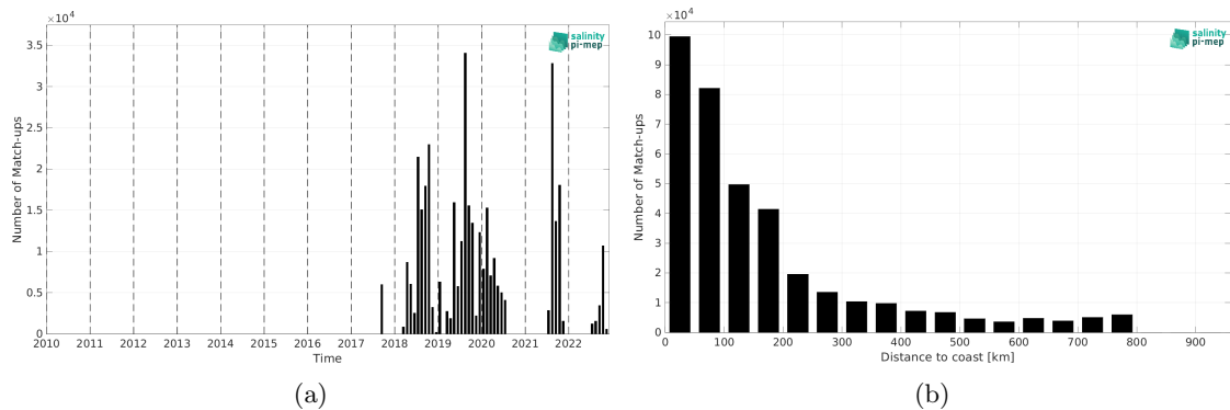
Figure 1: Number of match-ups between Sairdrone and SMAP SSS L2 v5.0 (JPL) SSS as a function of time (a) and as function of the distance to coast (b) over the SMOS coastal zone (<800km) 60N-60S Pi-MEP region and for the full satellite product period.
