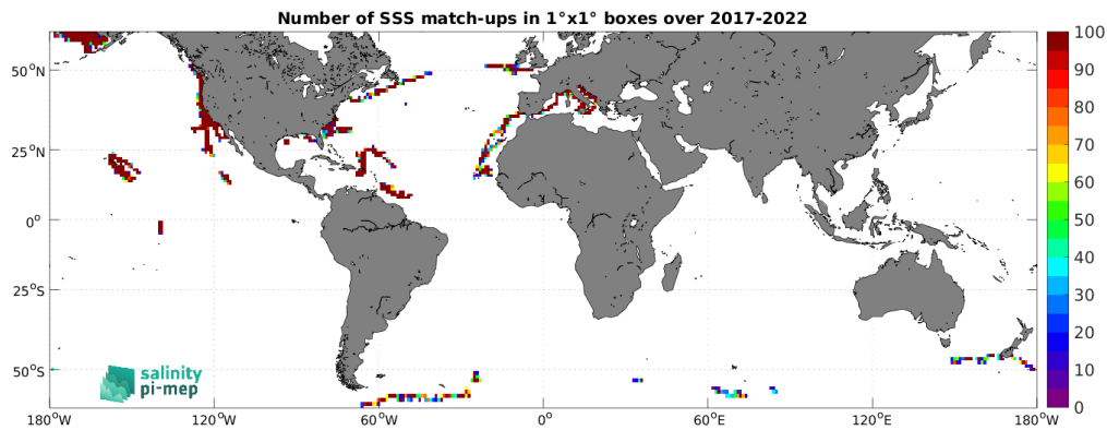
Figure 4: Number of SSS match-ups between Saildrone SSS and the SMAP SSS L2 v5.0 (JPL) SSS product for the SMOS coastal zone (<800km) 60N-60S Pi-MEP region over 1^\circ \times 1^\circ boxes and for the full satellite product period.
