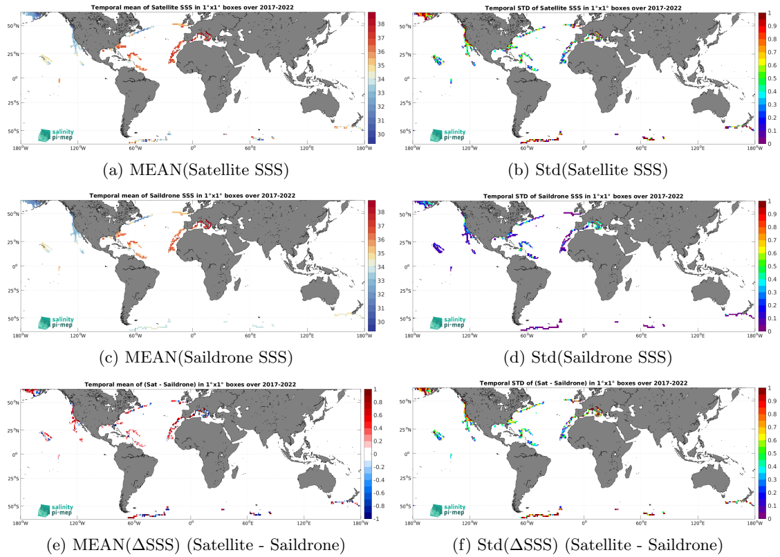
Figure 6: Temporal mean (left) and Std (right) of SSS from SMAP SSS L2 v5.0 (JPL) (top), Saildrone (middle), and of \Delta SSS (Satellite - Saildrone). Only match-up pairs are used to generate these maps.
