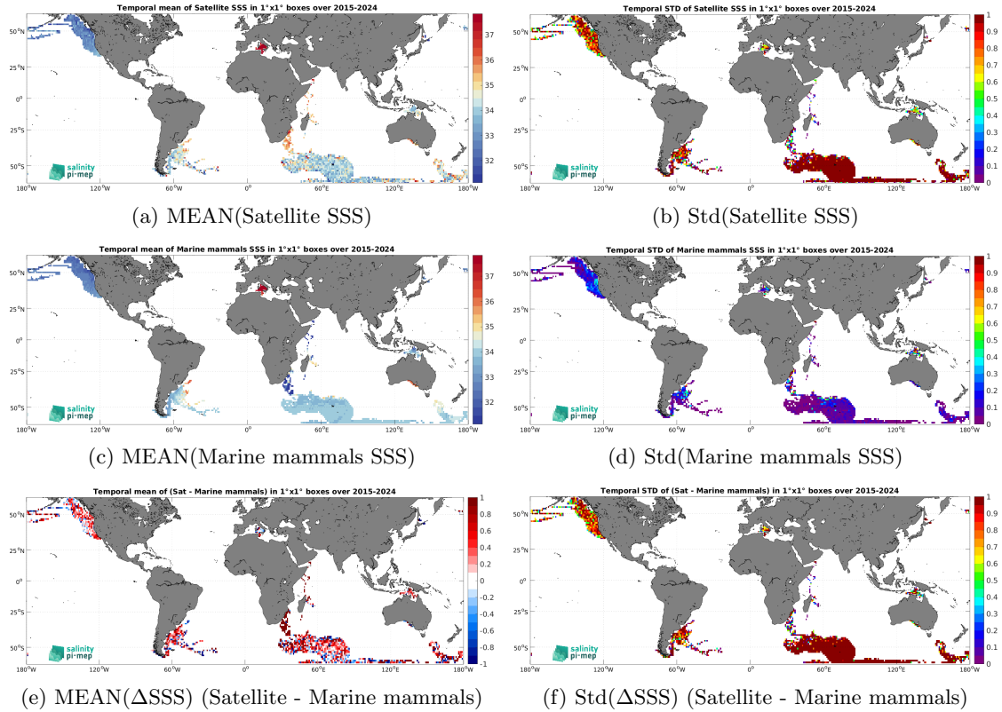
Figure 7: Temporal mean (left) and Std (right) of SSS from SMAP SSS L2 v5.0 (JPL) (top), Marine mammals (middle), and of \Delta SSS (Satellite - Marine mammals). Only match-up pairs are used to generate these maps.
