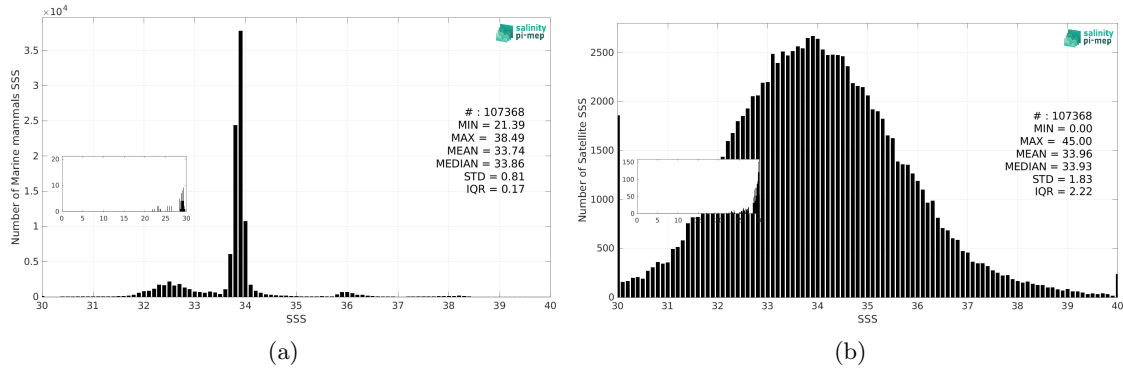
Figure 3: Histograms of SSS from Marine mammals (a) and SMAP SSS L2 v5.0 (JPL) (b) considering all match-up pairs per bins of 0.1 over the SMOS coastal zone (<800km) 60N-60S Pi-MEP region and for the full satellite product period.
