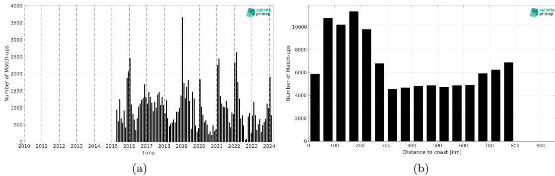
Figure 2: Number of match-ups between Marine mammals and SMAP SSS L2 v5.0 (JPL) SSS as a function of time (a) and as function of the distance to coast (b) over the SMOS coastal zone (<800km) 60N-60S Pi-MEP region and for the full satellite product period.
