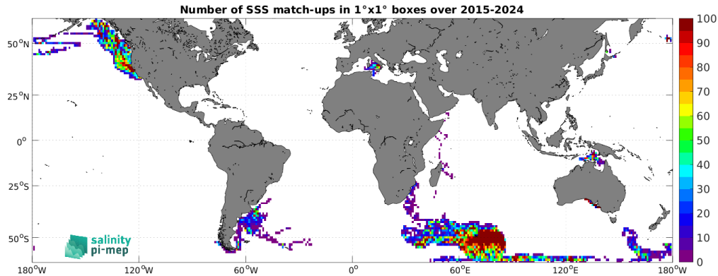
Figure 5: Number of SSS match-ups between Marine mammals SSS and the SMAP SSS L2 v5.0 (JPL) SSS product for the SMOS coastal zone (<800km) 60N-60S Pi-MEP region over 1^\circ \times 1^\circ boxes and for the full satellite product period.
