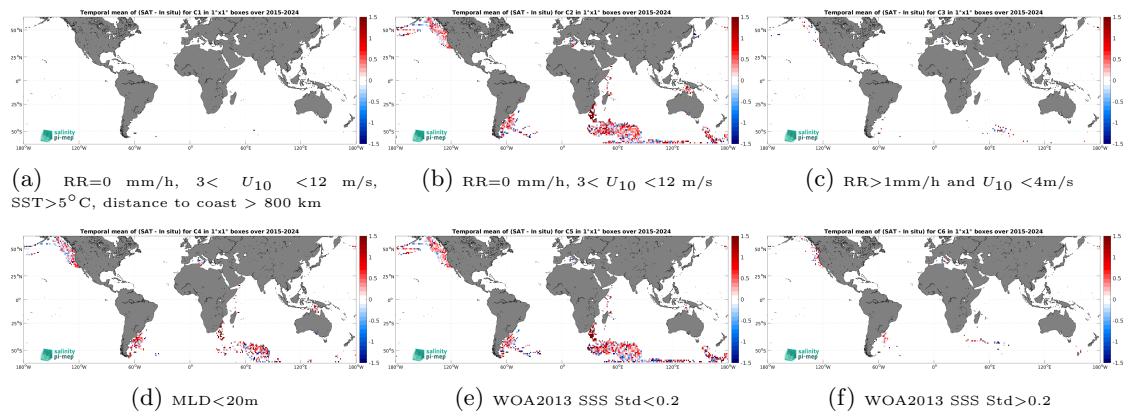
Figure 14: Temporal mean gridded over spatial boxes of size 1^\circ \times 1^\circ of \Delta\text{SSS} (SMAP SSS L2 v5.0 (JPL) - Marine mammals) for 6 different subdatasets corresponding to:RR=0 mm/h, 3 < U_{10} < 12 m/s, SST>5°C, distance to coast > 800 km (a), RR=0 mm/h, 3 < U_{10} < 12 m/s (b), RR>1mm/h and U_{10} < 4 m/s (c),MLD<20m (d),WOA2013 SSS Std<0.2 (e),WOA2013 SSS Std>0.2 (f).
