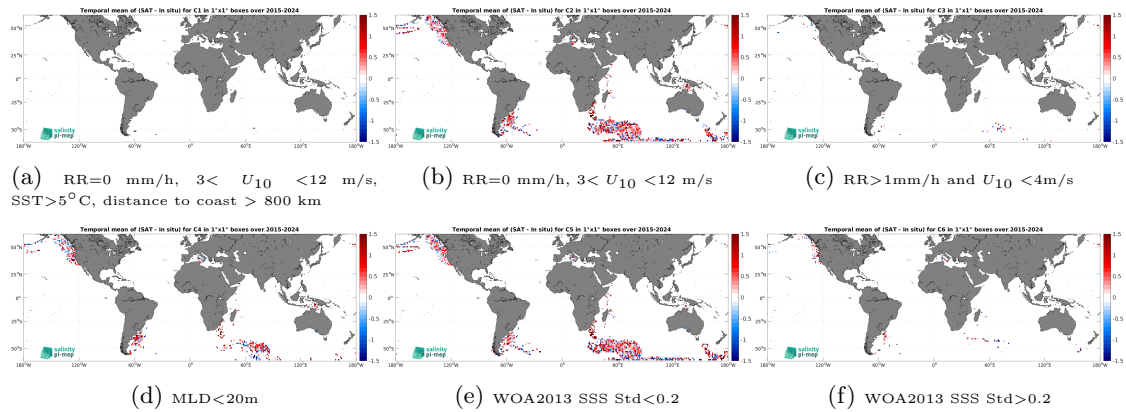
Figure 14: Temporal mean gridded over spatial boxes of size 1^\circ \times 1^\circ of \Delta SSS (SMAP SSS L2 v5.0 (JPL) - Marine mammals) for 6 different subdatasets corresponding to:RR=0 mm/h, 3 < U_{10} < 12 m/s, SST >5^\circ C, distance to coast > 800 km (a), RR=0 mm/h, 3 < U_{10} < 12 m/s (b), RR >1 mm/h and U_{10} < 4 m/s (c),MLD <20 m (d),WOA2013 SSS Std <0.2 (e),WOA2013 SSS Std >0.2 (f).
