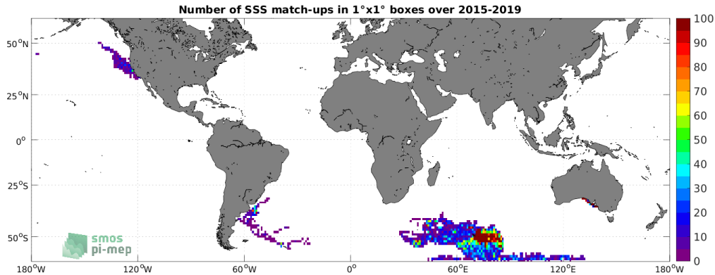
Figure 4: Number of SSS match-ups between Marine mammals SSS and the SMAP SSS L2 v5.0 (JPL) SSS product for the SMOS coastal zone (<800km) 60N-60S Pi-MEP region over 1^\circ \times 1^\circ boxes and for the full satellite product period.
