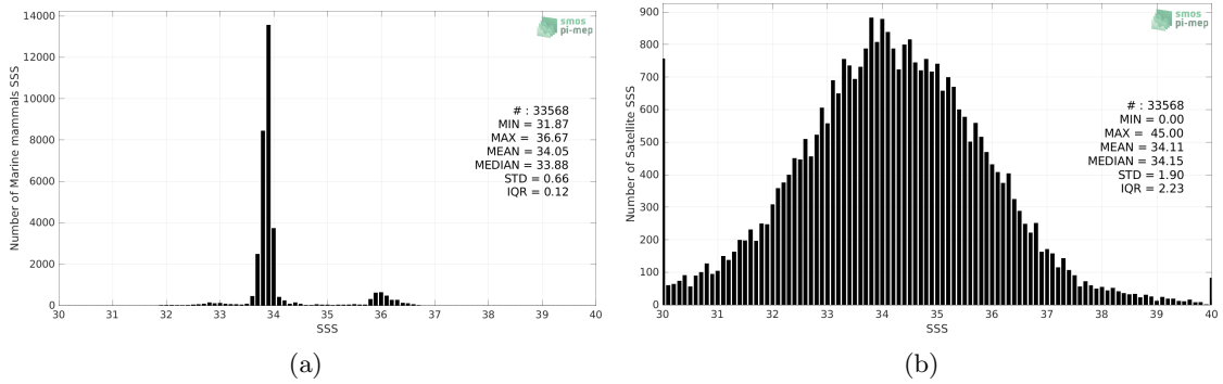
Figure 2: Histograms of SSS from Marine mammals (a) and SMAP SSS L2 v5.0 (JPL) (b) considering all match-up pairs per bins of 0.1 over the SMOS coastal zone (<800km) 60N-60S Pi-MEP region and for the full satellite product period.
