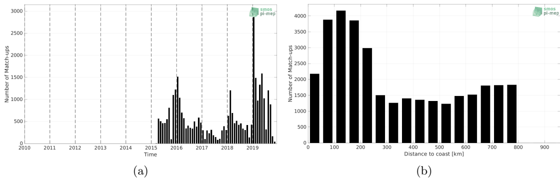
Figure 1: Number of match-ups between Marine mammals and SMAP SSS L2 v5.0 (JPL) SSS as a function of time (a) and as function of the distance to coast (b) over the SMOS coastal zone (<800km) 60N-60S Pi-MEP region and for the full satellite product period.
