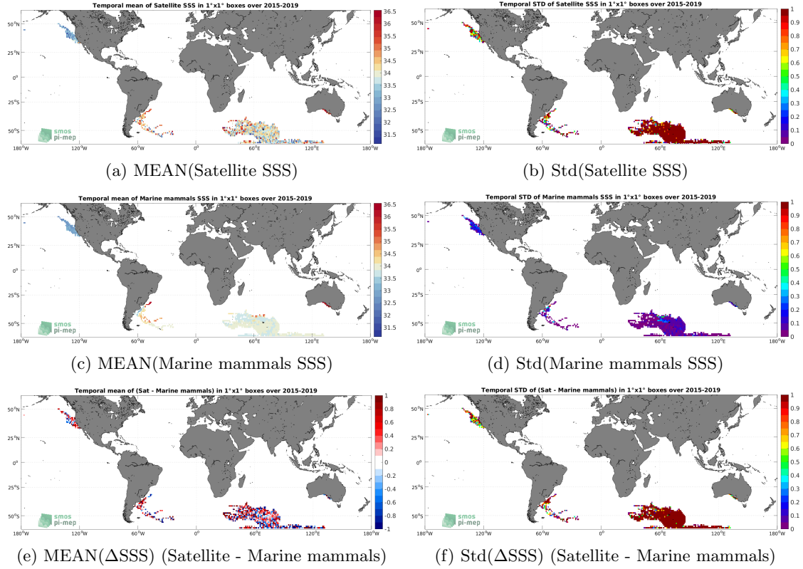
Figure 6: Temporal mean (left) and Std (right) of SSS from SMAP SSS L2 v5.0 (JPL) (top), Marine mammals (middle), and of \Delta SSS (Satellite - Marine mammals). Only match-up pairs are used to generate these maps.
