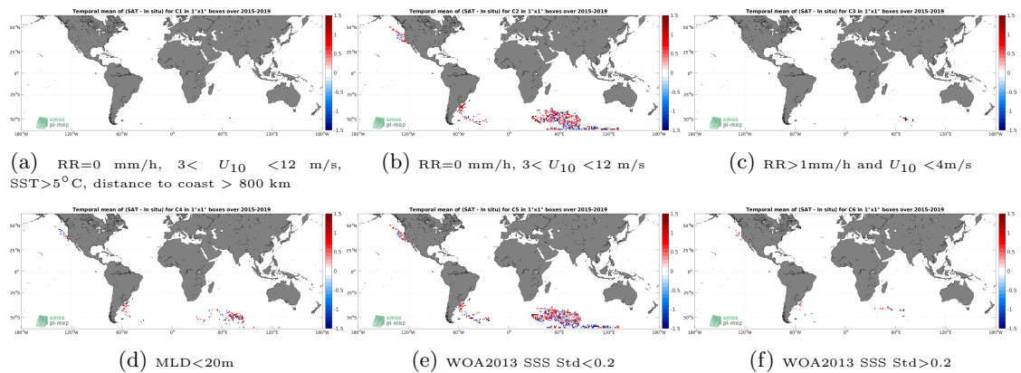
Figure 12: Temporal mean gridded over spatial boxes of size 1^\circ \times 1^\circ of \Delta SSS (SMAP SSS L2 v5.0 (JPL) - Marine mammals) for 6 different subdatasets corresponding to:RR=0 mm/h, 3 < U_{10} < 12 m/s, SST >5^\circ C, distance to coast > 800 km (a), RR=0 mm/h, 3 < U_{10} < 12 m/s (b), RR >1 mm/h and U_{10} < 4 m/s (c),MLD <20 m (d),WOA2013 SSS Std <0.2 (e),WOA2013 SSS Std >0.2 (f).
