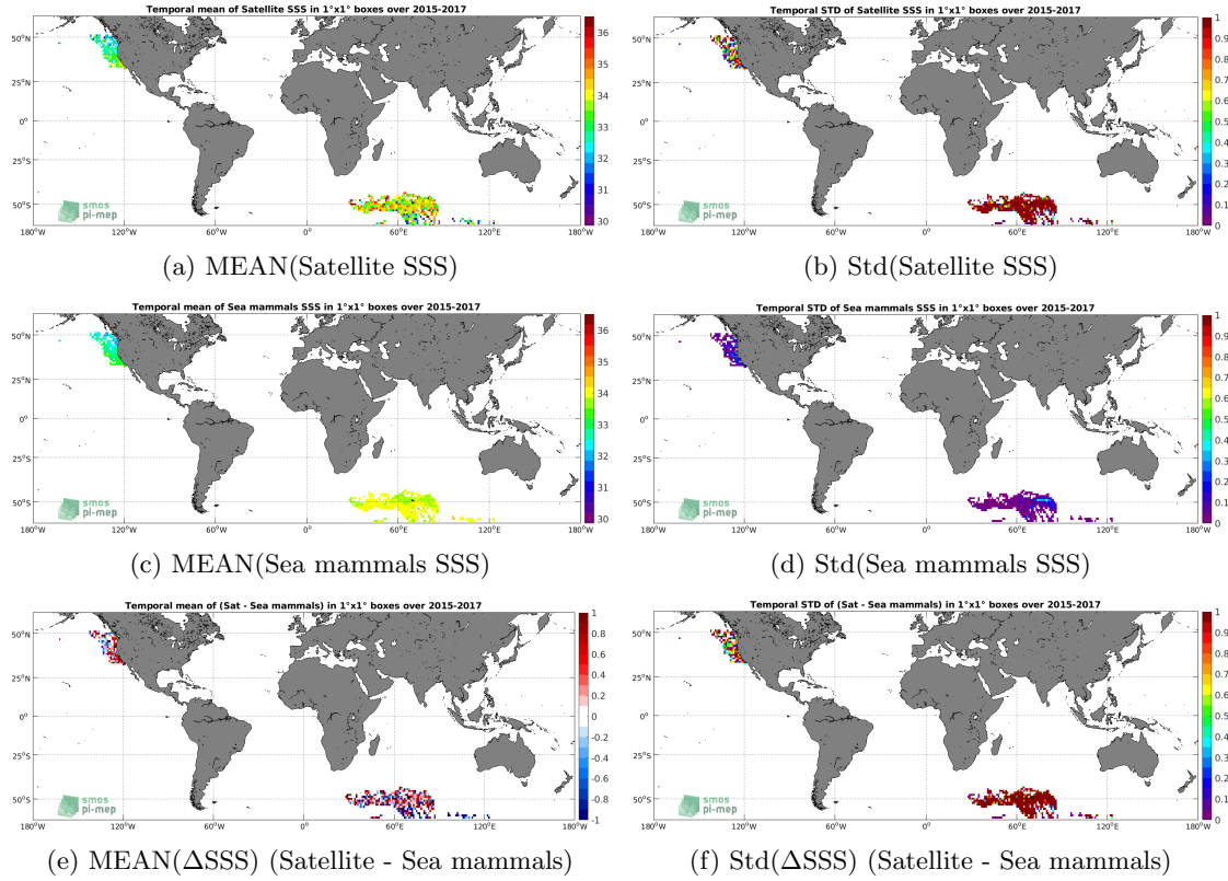
Figure 6: Temporal mean (left) and Std (right) of SSS from SMAP SSS L2 v5.0 (JPL) (top), Sea mammals (middle), and of \Delta SSS (Satellite - Sea mammals). Only match-up pairs are used to generate these maps.
