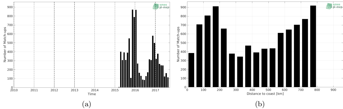
Figure 1: Number of match-ups between Sea mammals and SMAP SSS L2 v5.0 (JPL) SSS as a function of time (a) and as function of the distance to coast (b) over the SMOS coastal zone (<800km) 60N-60S Pi-MEP region and for the full satellite product period.
