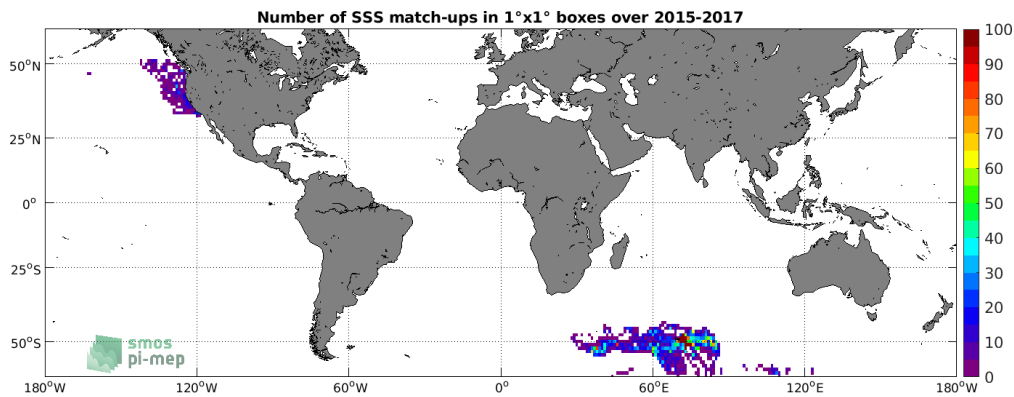
Figure 4: Number of SSS match-ups between Sea mammals SSS and the SMAP SSS L2 v5.0 (JPL) SSS product for the SMOS coastal zone (<800km) 60N-60S Pi-MEP region over 1°x1° boxes and for the full satellite product period.
