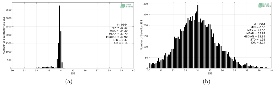
Figure 2: Histograms of SSS from Sea mammals (a) and SMAP SSS L2 v5.0 (JPL) (b) considering all match-up pairs per bins of 0.1 over the SMOS coastal zone (<800km) 60N-60S Pi-MEP region and for the full satellite product period.
