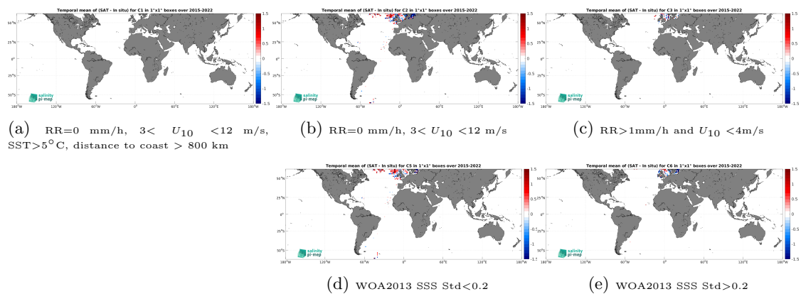
Figure 14: Temporal mean gridded over spatial boxes of size 1^\circ \times 1^\circ of \Delta\text{SSS} (SMAP SSS L2 v5.0 (JPL) - ICES) for 5 different subdatasets corresponding to: RR=0 mm/h, 3 < U_{10} < 12 m/s, SST > 5°C, distance to coast > 800 km (a), RR=0 mm/h, 3 < U_{10} < 12 m/s (b), RR > 1mm/h and U_{10} < 4 m/s (c), WOA2013 SSS Std < 0.2 (d), WOA2013 SSS Std > 0.2 (e).
