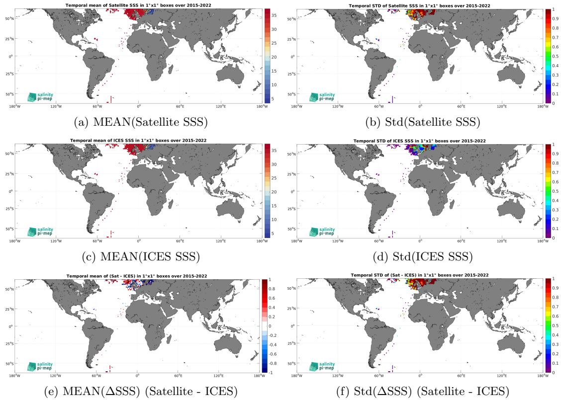
Figure 7: Temporal mean (left) and Std (right) of SSS from SMAP SSS L2 v5.0 (JPL) (top), ICES (middle), and of \Delta SSS (Satellite - ICES). Only match-up pairs are used to generate these maps.
