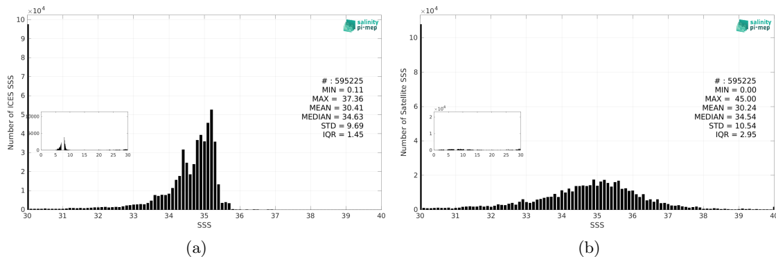
Figure 3: Histograms of SSS from ICES (a) and SMAP SSS L2 v5.0 (JPL) (b) considering all match-up pairs per bins of 0.1 over the SMOS coastal zone (<800km) 60N-60S Pi-MEP region and for the full satellite product period.
