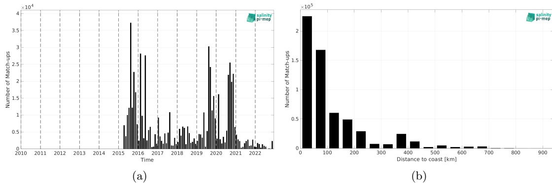
Figure 2: Number of match-ups between ICES and SMAP SSS L2 v5.0 (JPL) SSS as a function of time (a) and as function of the distance to coast (b) over the SMOS coastal zone (<800km) 60N-60S Pi-MEP region and for the full satellite product period.
