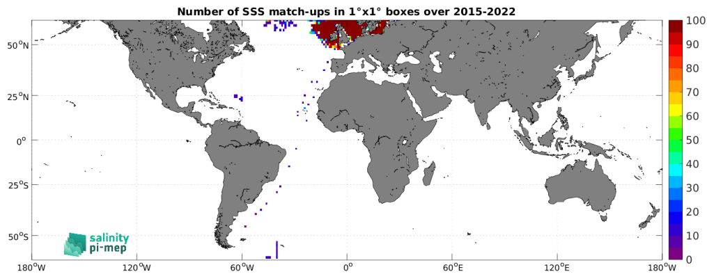
Figure 5: Number of SSS match-ups between ICES SSS and the SMAP SSS L2 v5.0 (JPL) SSS product for the SMOS coastal zone (<800km) 60N-60S Pi-MEP region over 1^\circ \times 1^\circ boxes and for the full satellite product period.
