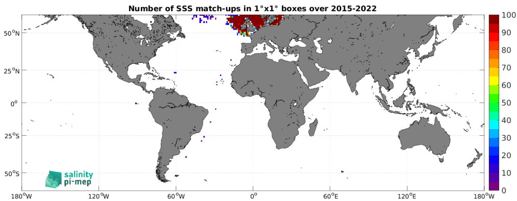
Figure 5: Number of SSS match-ups between ICES SSS and the SMAP SSS L2 v5.0 (JPL) SSS product for the SMOS coastal zone (<800km) 60N-60S Pi-MEP region over 1°×1° boxes and for the full satellite product period.
