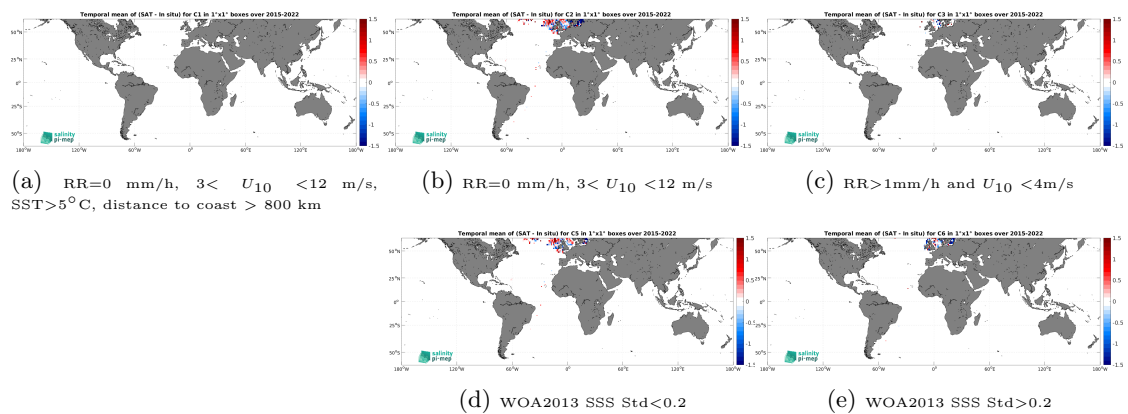
Figure 14: Temporal mean gridded over spatial boxes of size 1^\circ \times 1^\circ of \Delta SSS (SMAP SSS L2 v5.0 (JPL) - ICES) for 5 different subdatasets corresponding to:RR=0 mm/h, 3 < U_{10} < 12 m/s, SST >5^\circ C, distance to coast > 800 km (a), RR=0 mm/h, 3 < U_{10} < 12 m/s (b), RR >1 mm/h and U_{10} < 4 m/s (c), WOA2013 SSS Std <0.2 (d), WOA2013 SSS Std >0.2 (e).
