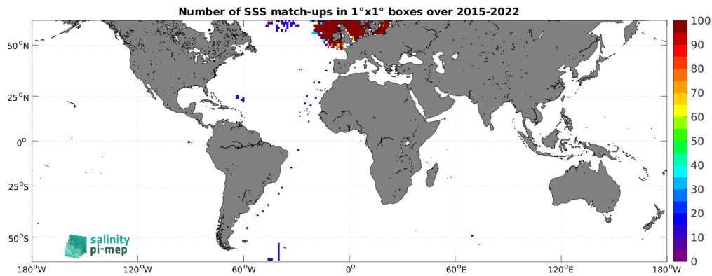
Figure 4: Number of SSS match-ups between ICES SSS and the SMAP SSS L2 v5.0 (JPL) SSS product for the SMOS coastal zone (<800km) 60N-60S Pi-MEP region over 1^\circ \times 1^\circ boxes and for the full satellite product period.
