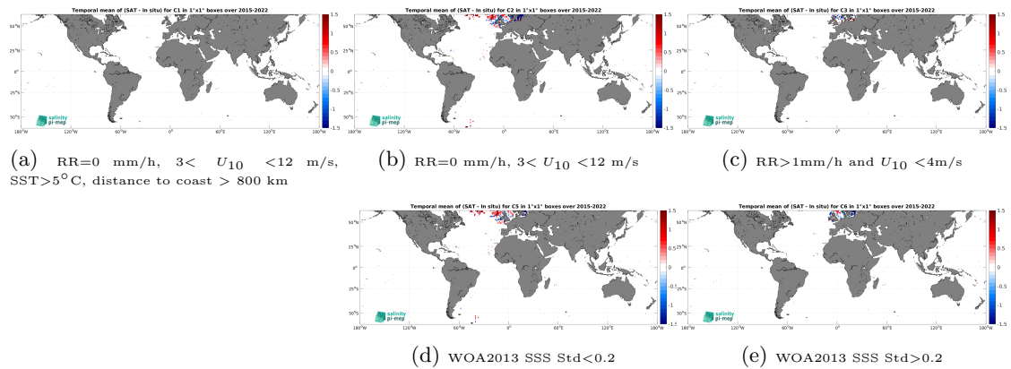
Figure 12: Temporal mean gridded over spatial boxes of size 1^\circ \times 1^\circ of \Delta SSS (SMAP SSS L2 v5.0 (JPL) - ICES) for 5 different subdatasets corresponding to: RR=0 mm/h, 3 < U_{10} < 12 m/s, SST > 5^\circ\text{C} , distance to coast > 800 km (a), RR=0 mm/h, 3 < U_{10} < 12 m/s (b), RR > 1 mm/h and U_{10} < 4 m/s (c), WOA2013 SSS Std < 0.2 (d), WOA2013 SSS Std > 0.2 (e).
