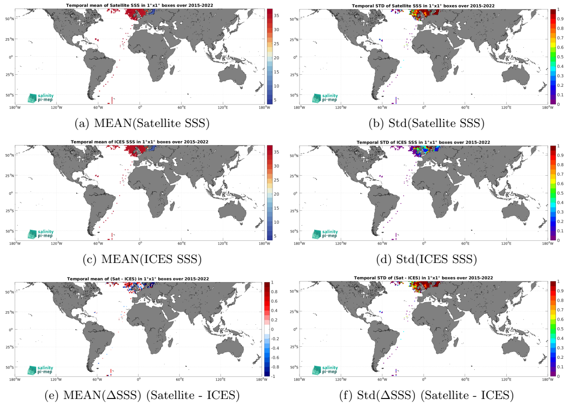
Figure 6: Temporal mean (left) and Std (right) of SSS from SMAP SSS L2 v5.0 (JPL) (top), ICES (middle), and of \Delta SSS (Satellite - ICES). Only match-up pairs are used to generate these maps.
