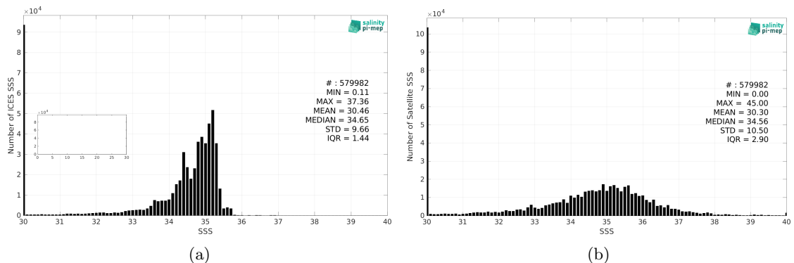
Figure 2: Histograms of SSS from ICES (a) and SMAP SSS L2 v5.0 (JPL) (b) considering all match-up pairs per bins of 0.1 over the SMOS coastal zone (<800km) 60N-60S Pi-MEP region and for the full satellite product period.
