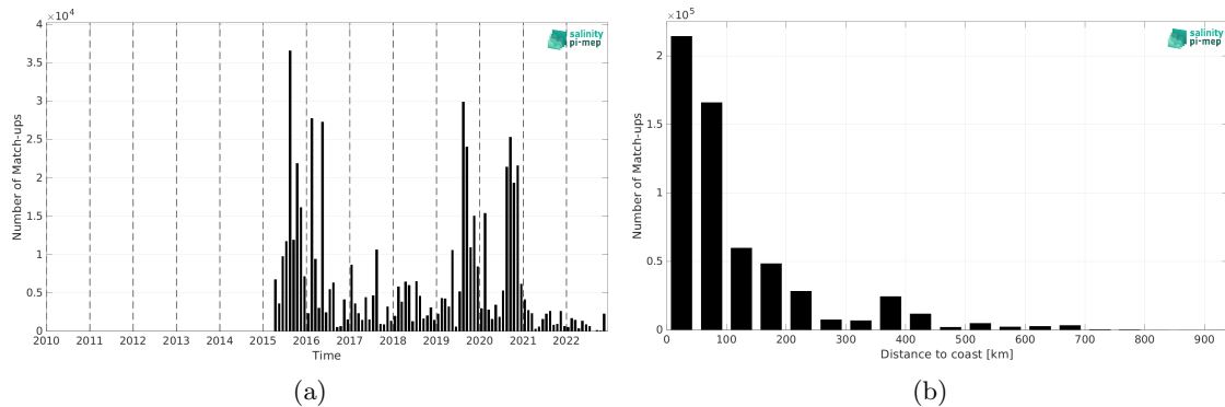
Figure 1: Number of match-ups between ICES and SMAP SSS L2 v5.0 (JPL) SSS as a function of time (a) and as function of the distance to coast (b) over the SMOS coastal zone (<800km) 60N-60S Pi-MEP region and for the full satellite product period.
