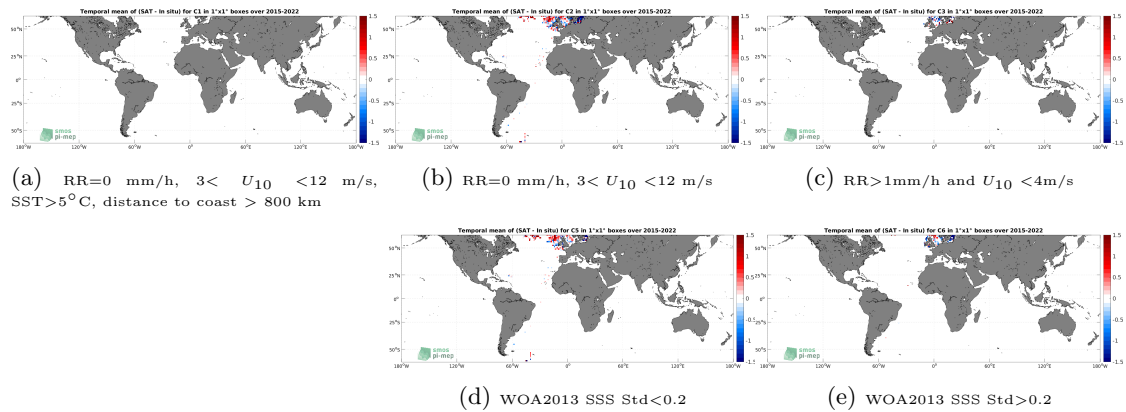
Figure 12: Temporal mean gridded over spatial boxes of size 1^\circ \times 1^\circ of \Delta\text{SSS} (SMAP SSS L2 v5.0 (JPL) - ICES) for 5 different subdatasets corresponding to:RR=0 mm/h, 3 < U_{10} < 12 m/s, SST >5^\circ\text{C} , distance to coast > 800 km (a), RR=0 mm/h, 3 < U_{10} < 12 m/s (b), RR >1 mm/h and U_{10} < 4 m/s (c), WOA2013 SSS Std <0.2 (d), WOA2013 SSS Std >0.2 (e).
