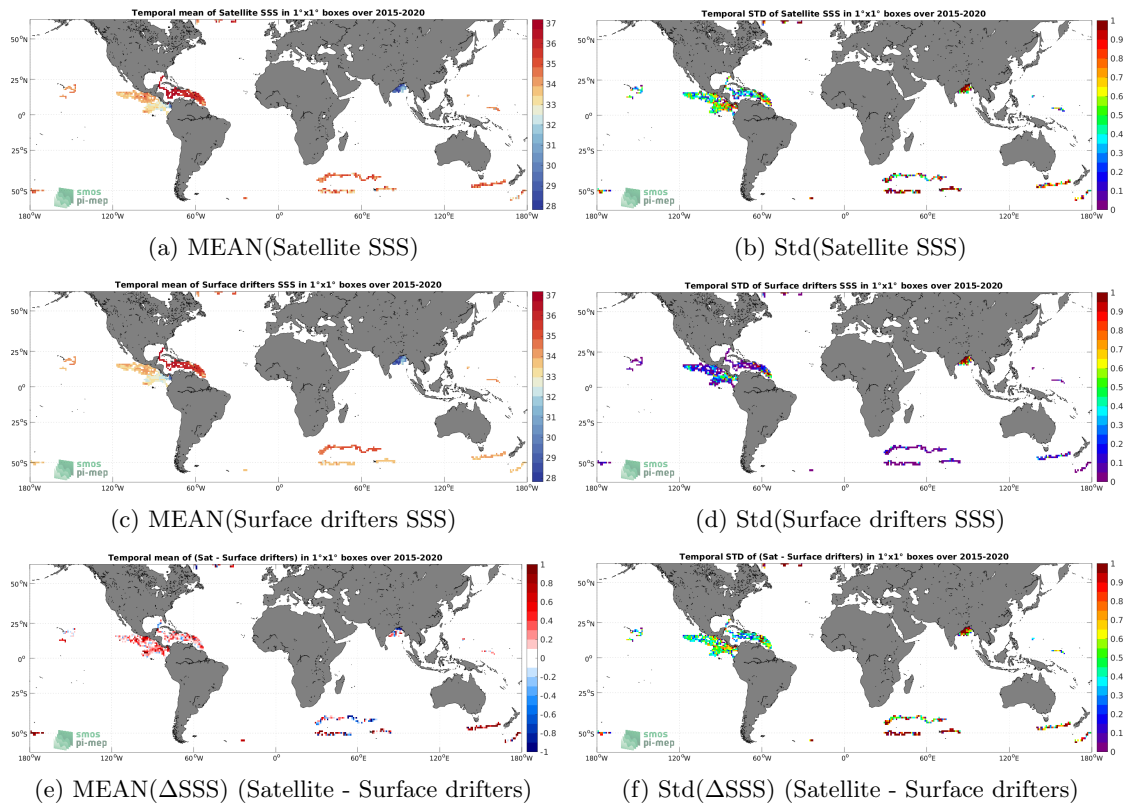
Figure 5: Temporal mean (left) and Std (right) of SSS from SMAP SSS L2 v5.0 (JPL) (top), Surface drifters (middle), and of \Delta SSS (Satellite - Surface drifters). Only match-up pairs are used to generate these maps.
