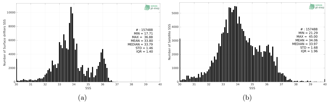
Figure 2: Histograms of SSS from Surface drifters (a) and SMAP SSS L2 v5.0 (JPL) (b) considering all match-up pairs per bins of 0.1 over the SMOS coastal zone (<800km) 60N-60S Pi-MEP region and for the full satellite product period.
