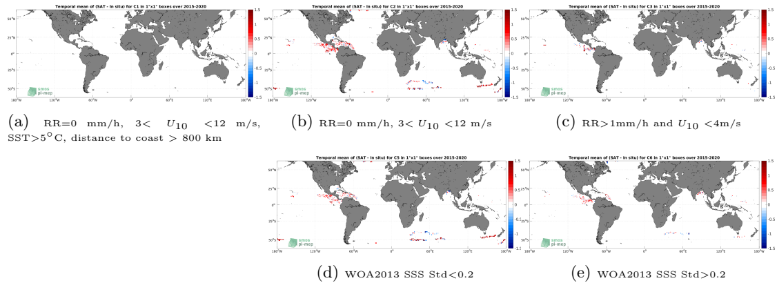
Figure 11: Temporal mean gridded over spatial boxes of size 1^\circ \times 1^\circ of \Delta SSS (SMAP SSS L2 v5.0 (JPL) - Surface drifters) for 5 different subdatasets corresponding to:RR=0 mm/h, 3 < U_{10} < 12 m/s, SST >5^\circ C, distance to coast > 800 km (a), RR=0 mm/h, 3 < U_{10} < 12 m/s (b), RR >1 mm/h and U_{10} < 4 m/s (c), WOA2013 SSS Std <0.2 (d), WOA2013 SSS Std >0.2 (e).
