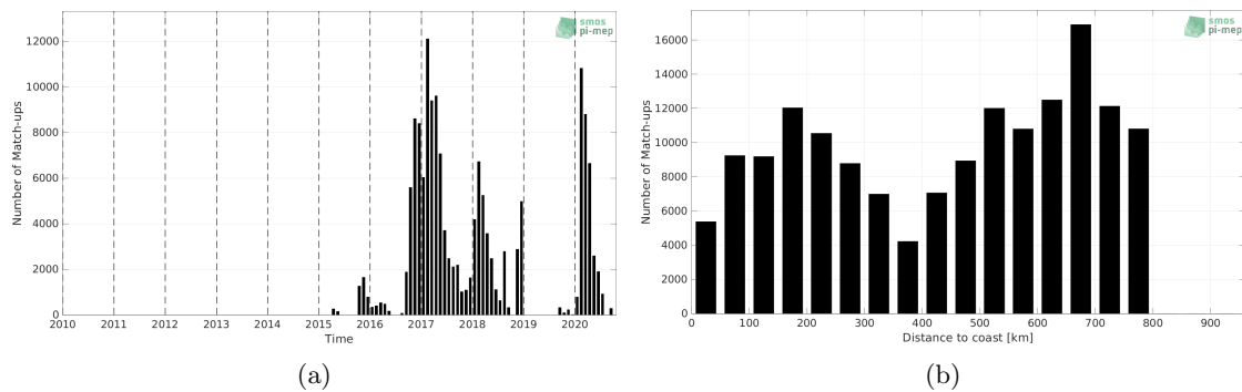
Figure 1: Number of match-ups between Surface drifters and SMAP SSS L2 v5.0 (JPL) SSS as a function of time (a) and as function of the distance to coast (b) over the SMOS coastal zone (<800km) 60N-60S Pi-MEP region and for the full satellite product period.
