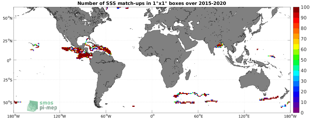
Figure 3: Number of SSS match-ups between Surface drifters SSS and the SMAP SSS L2 v5.0 (JPL) SSS product for the SMOS coastal zone (<800km) 60N-60S Pi-MEP region over 1^\circ \times 1^\circ boxes and for the full satellite product period.
