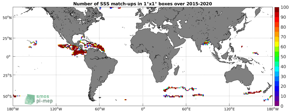
Figure 3: Number of SSS match-ups between Surface drifters SSS and the SMAP SSS L2 v5.0 (JPL) SSS product for the SMOS coastal zone (<800km) 60N-60S Pi-MEP region over 1°x1° boxes and for the full satellite product period.
