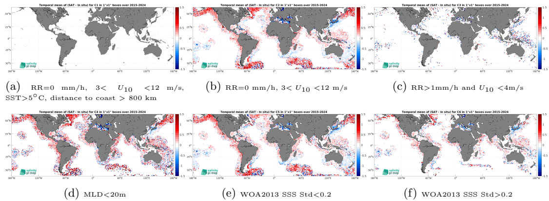
Figure 14: Temporal mean gridded over spatial boxes of size 1^\circ \times 1^\circ of \Delta SSS (SMAP SSS L2 v5.0 (JPL) - Argo) for 6 different subdatasets corresponding to:RR=0 mm/h, 3 < U_{10} < 12 m/s, SST > 5^\circ\text{C} , distance to coast > 800 km (a), RR=0 mm/h, 3 < U_{10} < 12 m/s (b), RR > 1 mm/h and U_{10} < 4 m/s (c),MLD < 20 m (d),WOA2013 SSS Std < 0.2 (e),WOA2013 SSS Std > 0.2 (f).
