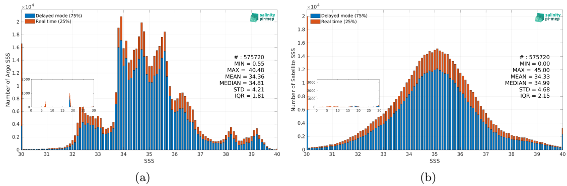
Figure 3: Histograms of SSS from Argo (a) and SMAP SSS L2 v5.0 (JPL) (b) considering all match-up pairs per bins of 0.1 over the SMOS coastal zone (<800km) 60N-60S Pi-MEP region and for the full satellite product period.
