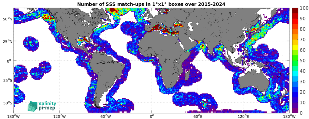
Figure 5: Number of SSS match-ups between Argo SSS and the SMAP SSS L2 v5.0 (JPL) SSS product for the SMOS coastal zone (<800km) 60N-60S Pi-MEP region over 1^\circ \times 1^\circ boxes and for the full satellite product period.
