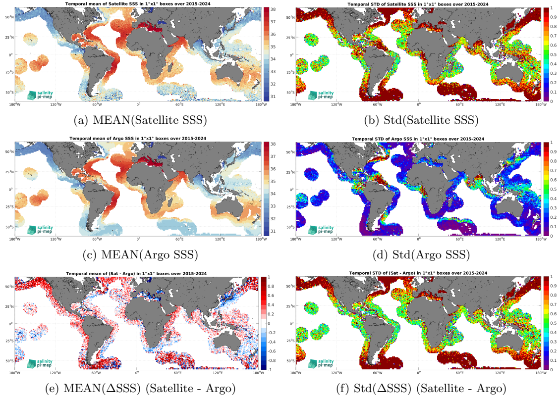
Figure 7: Temporal mean (left) and Std (right) of SSS from SMAP SSS L2 v5.0 (JPL) (top), Argo (middle), and of \Delta SSS (Satellite - Argo). Only match-up pairs are used to generate these maps.
