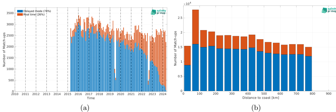
Figure 2: Number of match-ups between Argo and SMAP SSS L2 v5.0 (JPL) SSS as a function of time (a) and as function of the distance to coast (b) over the SMOS coastal zone (<800km) 60N-60S Pi-MEP region and for the full satellite product period.
