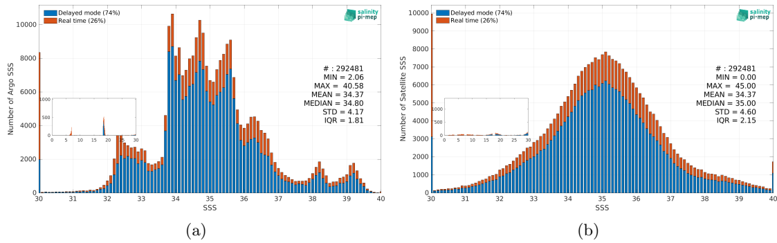
Figure 3: Histograms of SSS from Argo (a) and SMAP SSS L2 v5.0 (JPL) (b) considering all match-up pairs per bins of 0.1 over the SMOS coastal zone (<800km) 60N-60S Pi-MEP region and for the full satellite product period.
