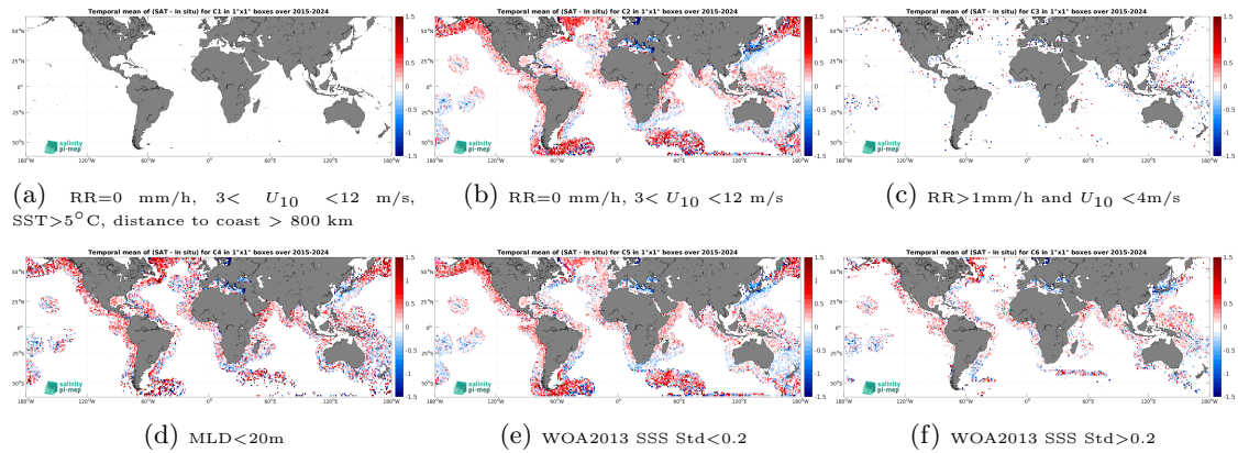
Figure 14: Temporal mean gridded over spatial boxes of size 1^\circ \times 1^\circ of \Delta SSS (SMAP SSS L2 v5.0 (JPL) - Argo) for 6 different subdatasets corresponding to: RR=0 mm/h, 3 < U_{10} < 12 m/s, SST > 5°C, distance to coast > 800 km (a), RR=0 mm/h, 3 < U_{10} < 12 m/s (b), RR > 1mm/h and U_{10} < 4 m/s (c), MLD < 20m (d), WOA2013 SSS Std < 0.2 (e), WOA2013 SSS Std > 0.2 (f).
