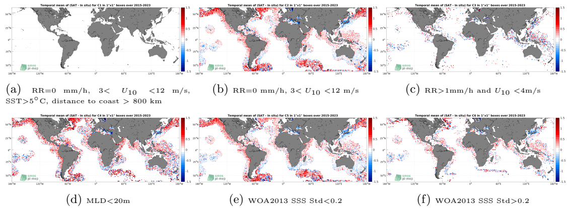
Figure 12: Temporal mean gridded over spatial boxes of size 1^\circ \times 1^\circ of \Delta SSS (SMAP SSS L2 v5.0 (JPL) - Argo) for 6 different subdatasets corresponding to: RR=0 mm/h, 3 < U_{10} < 12 m/s, SST > 5^\circ\text{C} , distance to coast > 800 km (a), RR=0 mm/h, 3 < U_{10} < 12 m/s (b), RR > 1 mm/h and U_{10} < 4 m/s (c), MLD < 20 m (d), WOA2013 SSS Std < 0.2 (e), WOA2013 SSS Std > 0.2 (f).
