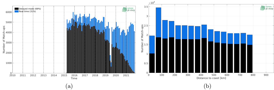
Figure 1: Number of match-ups between Argo and SMAP SSS L2 v5.0 (JPL) SSS as a function of time (a) and as function of the distance to coast (b) over the SMOS coastal zone (<800km) 60N-60S Pi-MEP region and for the full satellite product period.
