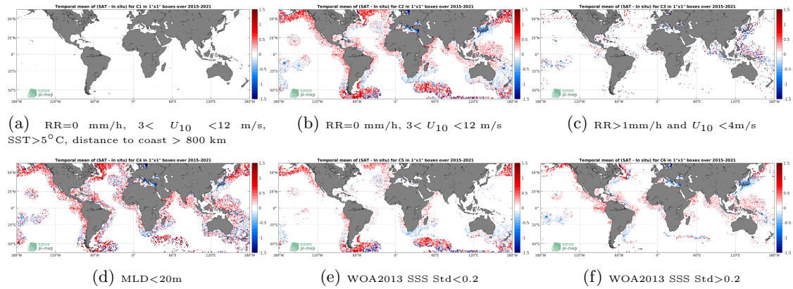
Figure 12: Temporal mean gridded over spatial boxes of size 1^\circ \times 1^\circ of \Delta SSS (SMAP SSS L2 v5.0 (JPL) - Argo) for 6 different subdatasets corresponding to:RR=0 mm/h, 3 < U_{10} < 12 m/s, SST > 5°C, distance to coast > 800 km (a), RR=0 mm/h, 3 < U_{10} < 12 m/s (b), RR > 1mm/h and U_{10} < 4 m/s (c),MLD < 20m (d),WOA2013 SSS Std < 0.2 (e),WOA2013 SSS Std > 0.2 (f).
