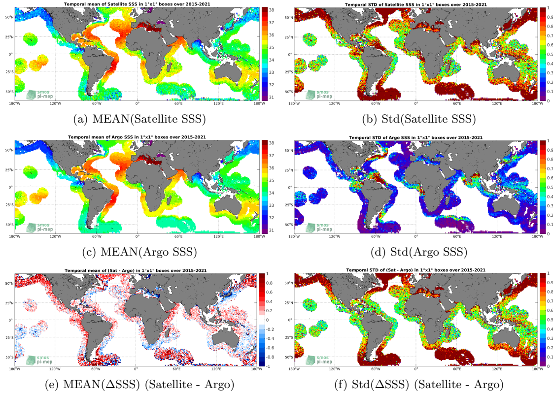
Figure 6: Temporal mean (left) and Std (right) of SSS from SMAP SSS L2 v5.0 (JPL) (top), Argo (middle), and of \Delta SSS (Satellite - Argo). Only match-up pairs are used to generate these maps.
