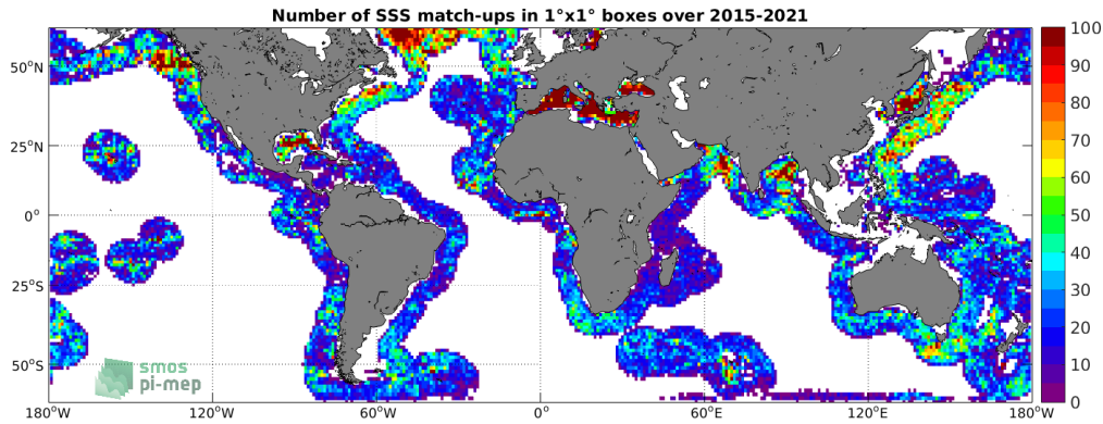
Figure 4: Number of SSS match-ups between Argo SSS and the SMAP SSS L2 v5.0 (JPL) SSS product for the SMOS coastal zone (<800km) 60N-60S Pi-MEP region over 1^\circ \times 1^\circ boxes and for the full satellite product period.
