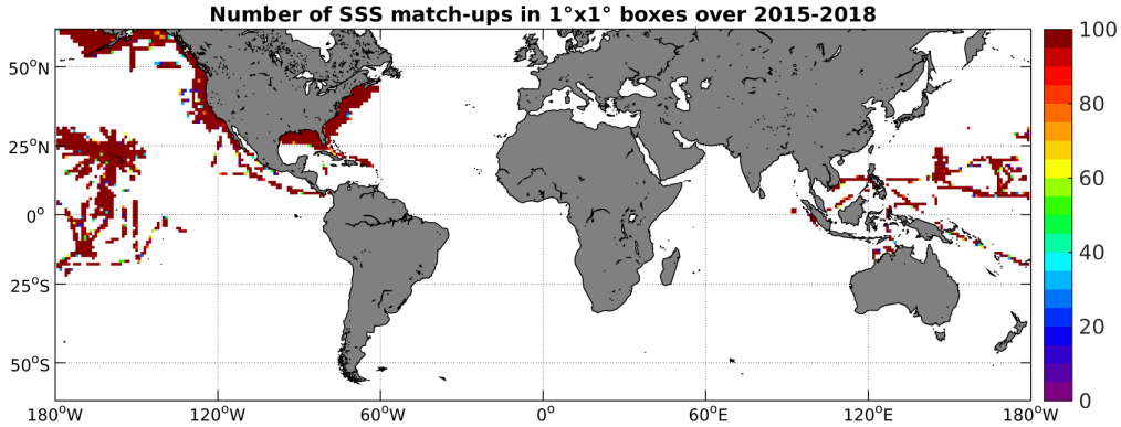
Figure 4: Number of SSS match-ups between TSG-SAMOS SSS and the SMAP-L2-JPL-V4 SSS product for the SMOS coastal zone ( \geq 800\text{km} ) 60N-60S Pi-MEP region over 1^\circ \times 1^\circ boxes and for the full satellite product period.
