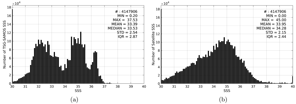
Figure 2: Histograms of SSS from TSG-SAMOS (a) and SMAP-L2-JPL-V4 (b) considering all match-up pairs per bins of 0.1 over the SMOS coastal zone ( \pm 800\text{km} ) 60N-60S Pi-MEP region and for the full satellite product period.
