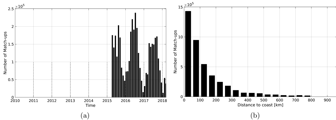
Figure 1: Number of match-ups between TSG-SAMOS and SMAP-L2-JPL-V4 SSS as a function of time (a) and as function of the distance to coast (b) over the SMOS coastal zone ( \pm 800 km) 60N-60S Pi-MEP region and for the full satellite product period.
