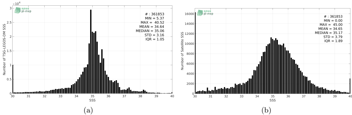
Figure 2: Histograms of SSS from TSG-LEGOS-DM (a) and SMAP-L2-JPL-V4 (b) considering all match-up pairs per bins of 0.1 over the SMOS coastal zone ( \pm 800\text{km} ) 60N-60S Pi-MEP region and for the full satellite product period.
