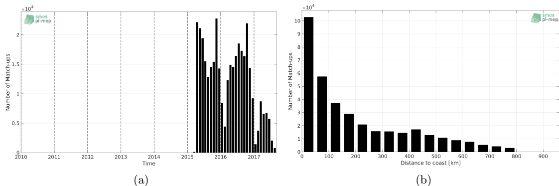
Figure 1: Number of match-ups between TSG-LEGOS-DM and SMAP-L2-JPL-V4 SSS as a function of time (a) and as function of the distance to coast (b) over the SMOS coastal zone ( \pm 800 km) 60N-60S Pi-MEP region and for the full satellite product period.
