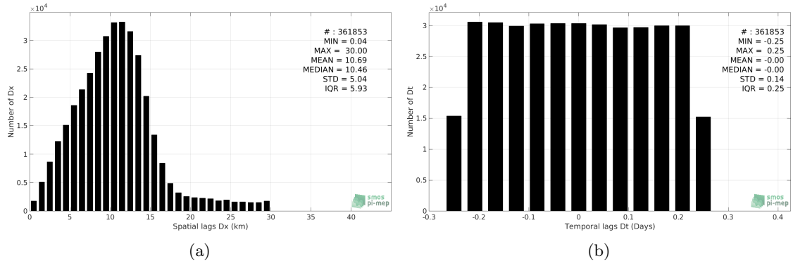
Figure 5: Histograms of the spatial (a) and temporal (b) lags between the time of the TSG-LEGOS-DM measurements and the date of the corresponding SMAP-L2-JPL-V4 SSS product.
