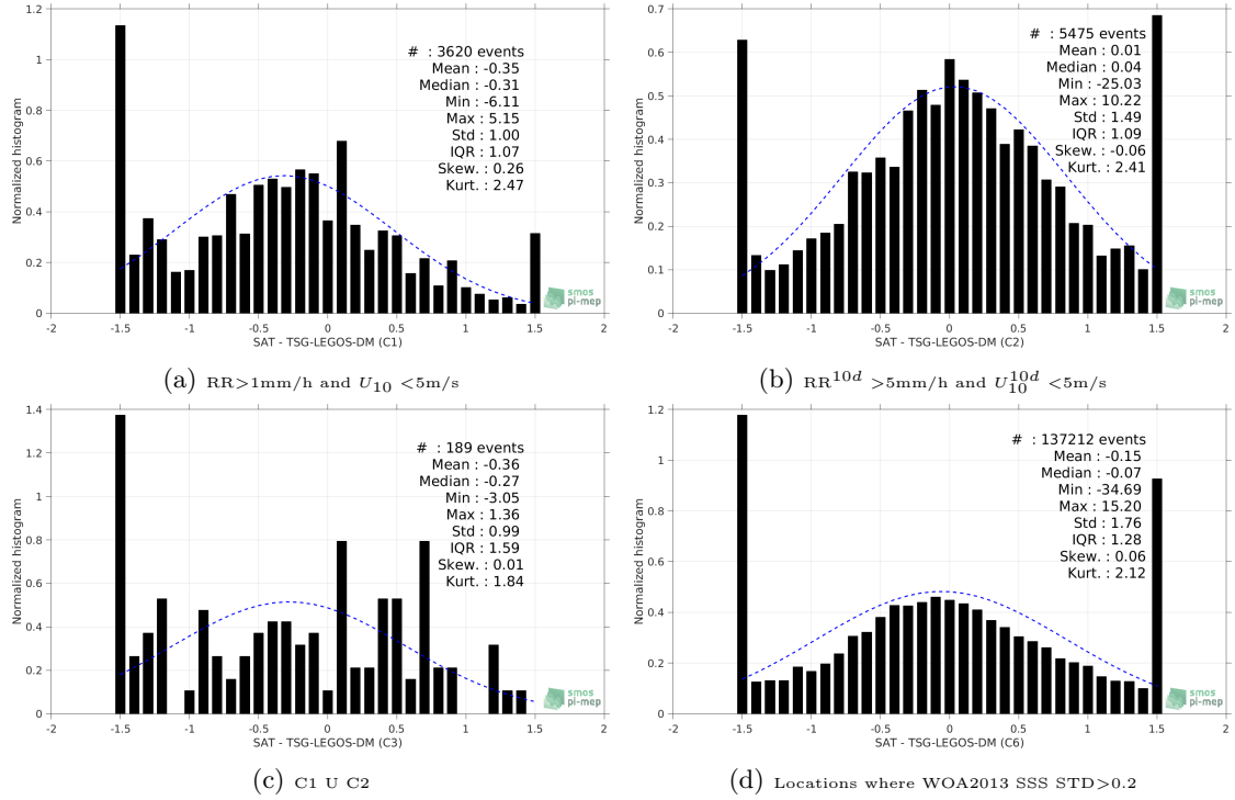
Figure 13: Normalized histogram of \Delta SSS (SMAP-L2-JPL-V4 - TSG-LEGOS-DM) for 6 different subdatasets corresponding to: RR > 1\text{mm/h} and U_{10} < 5\text{m/s} (a), RR^{10d} > 5\text{mm/h} and U_{10}^{10d} < 5\text{m/s} (b), C1 U C2 (c), Locations where WOA2013 SSS STD > 0.2 (d).
