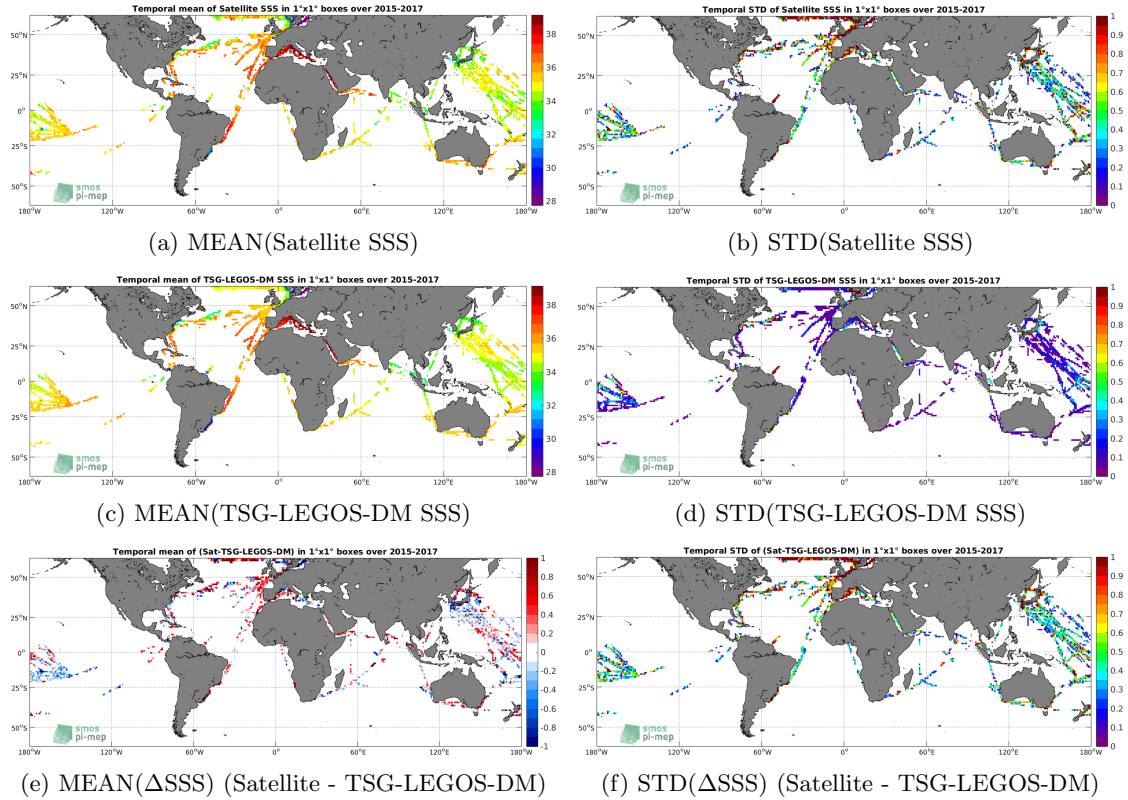
Figure 6: Temporal mean (left) and STD (right) of SSS from SMAP-L2-JPL-V4 (top), TSG-LEGOS-DM (middle), and of \Delta SSS (Satellite - TSG-LEGOS-DM). Only match-up pairs are used to generate these maps.
