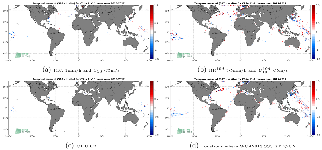
Figure 12: Temporal mean gridded over spatial boxes of size 1^\circ \times 1^\circ of \Delta SSS (SMAP-L2-JPL-V4 - TSG-LEGOS-DM) for 4 different subdatasets corresponding to: RR > 1mm/h and U_{10} < 5\text{m/s} (a), RR^{10d} > 5\text{mm/h} and U_{10}^{10d} < 5\text{m/s} (b), C1 U C2 (c), Locations where WOA2013 SSS STD > 0.2 (d).
