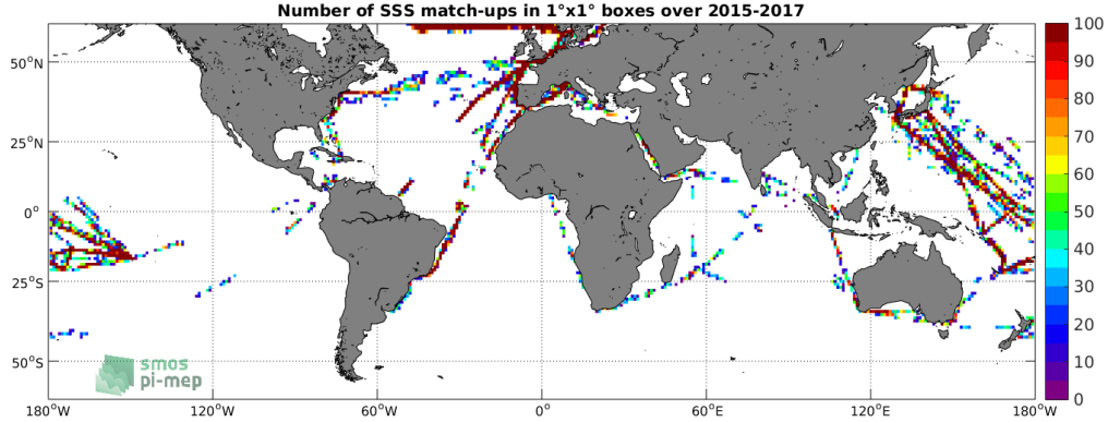
Figure 4: Number of SSS match-ups between TSG-LEGOS-DM SSS and the SMAP-L2-JPL-V4 SSS product for the SMOS coastal zone ( \leq 800\text{km} ) 60N-60S Pi-MEP region over 1^\circ \times 1^\circ boxes and for the full satellite product period.
