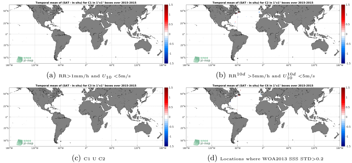
Figure 12: Temporal mean gridded over spatial boxes of size 1^\circ \times 1^\circ of \Delta SSS (SMAP-L2-JPL-V4 - TSG-GOSUD-Sailing-ship) for 4 different subdatasets corresponding to: RR > 1\text{mm/h} and U_{10} < 5\text{m/s} (a), RR^{10d} > 5\text{mm/h} and U_{10}^{10d} < 5\text{m/s} (b), C1 U C2 (c), Locations where WOA2013 SSS STD > 0.2 (d).
