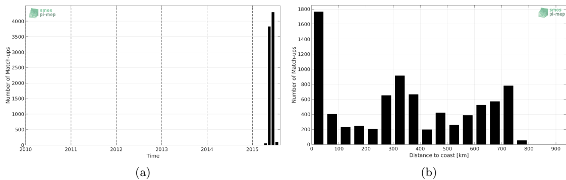
Figure 1: Number of match-ups between TSG-GOSUD-Sailing-ship and SMAP-L2-JPL-V4 SSS as a function of time (a) and as function of the distance to coast (b) over the SMOS coastal zone ( \pm 800 km) 60N-60S Pi-MEP region and for the full satellite product period.
