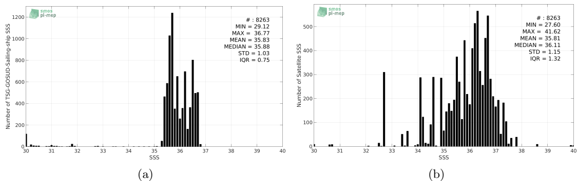
Figure 2: Histograms of SSS from TSG-GOSUD-Sailing-ship (a) and SMAP-L2-JPL-V4 (b) considering all match-up pairs per bins of 0.1 over the SMOS coastal zone ( \pm 800\text{km} ) 60N-60S Pi-MEP region and for the full satellite product period.
