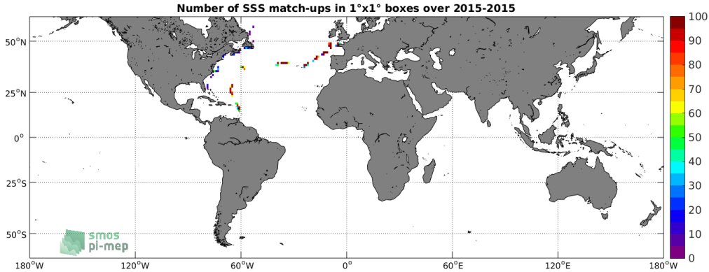
Figure 4: Number of SSS match-ups between TSG-GOSUD-Sailing-ship SSS and the SMAP-L2-JPL-V4 SSS product for the SMOS coastal zone ( \approx 800\text{km} ) 60\text{N} - 60\text{S} Pi-MEP region over 1^\circ \times 1^\circ boxes and for the full satellite product period.
