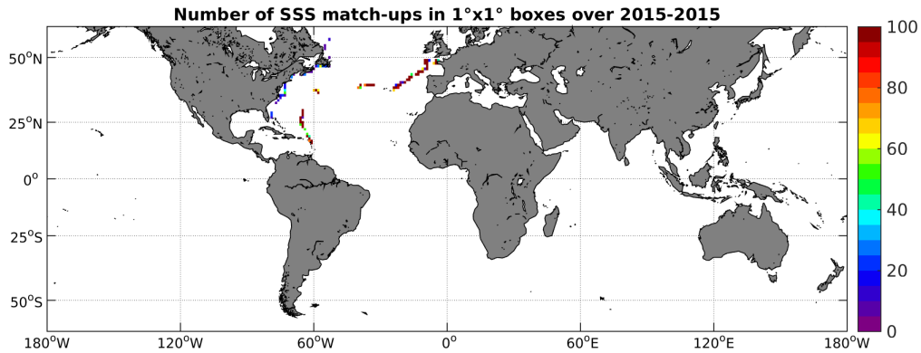
Figure 4: Number of SSS match-ups between TSG-GOSUD-Sailing-ship SSS and the SMAP-L2-JPL-V4 SSS product for the SMOS coastal zone ( \approx 800\text{km} ) 60N-60S Pi-MEP region over 1^\circ \times 1^\circ boxes and for the full satellite product period.
