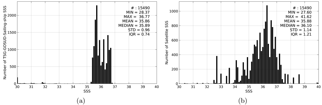
Figure 2: Histograms of SSS from TSG-GOSUD-Sailing-ship (a) and SMAP-L2-JPL-V4 (b) considering all match-up pairs per bins of 0.1 over the SMOS coastal zone ( \approx 800\text{km} ) 60N-60S Pi-MEP region and for the full satellite product period.
