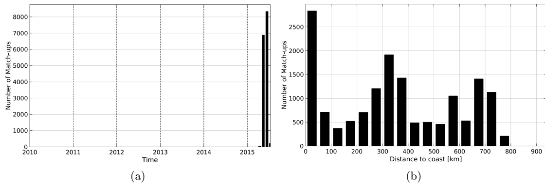
Figure 1: Number of match-ups between TSG-GOSUD-Sailing-ship and SMAP-L2-JPL-V4 SSS as a function of time (a) and as function of the distance to coast (b) over the SMOS coastal zone ( \pm 800\text{km} ) 60N-60S Pi-MEP region and for the full satellite product period.
