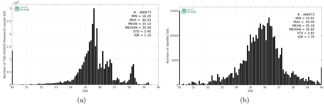
Figure 2: Histograms of SSS from TSG-GOSUD-Research-vessel (a) and SMAP-L2-JPL-V4 (b) considering all match-up pairs per bins of 0.1 over the SMOS coastal zone ( \approx 800\text{km} ) 60^\circ\text{N} - 60^\circ\text{S} Pi-MEP region and for the full satellite product period.
