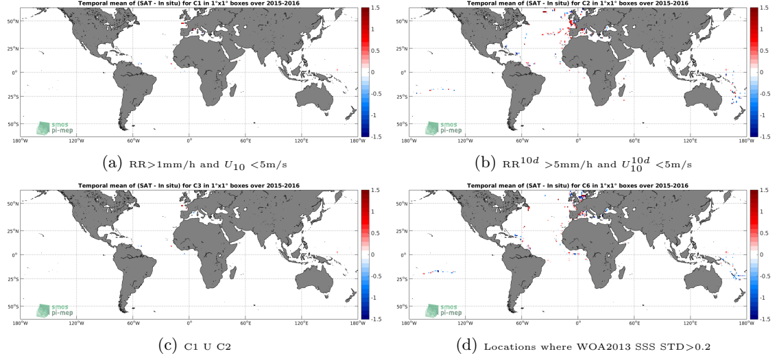
Figure 12: Temporal mean gridded over spatial boxes of size 1^\circ \times 1^\circ of \Delta SSS (SMAP-L2-JPL-V4 - TSG-GOSUD-Research-vessel) for 4 different subdatasets corresponding to: RR > 1\text{mm/h} and U_{10} < 5\text{m/s} (a), RR^{10d} > 5\text{mm/h} and U_{10}^{10d} < 5\text{m/s} (b), C1 U C2 (c), Locations where WOA2013 SSS STD > 0.2 (d).
