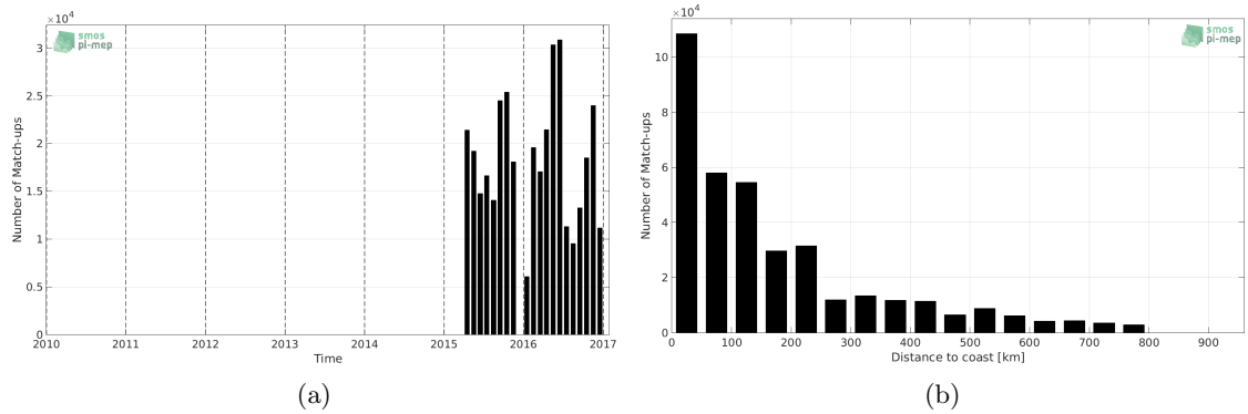
Figure 1: Number of match-ups between TSG-GOSUD-Research-vessel and SMAP-L2-JPL-V4 SSS as a function of time (a) and as function of the distance to coast (b) over the SMOS coastal zone ( \pm 800 km) 60N-60S Pi-MEP region and for the full satellite product period.
