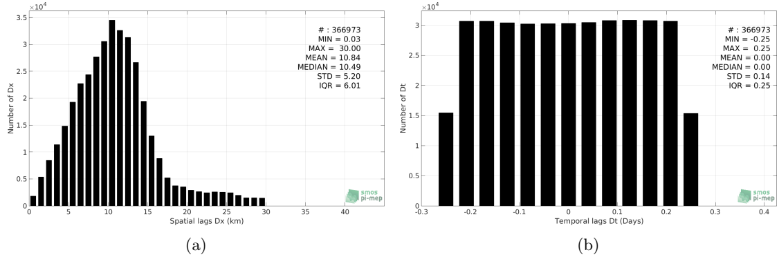
Figure 5: Histograms of the spatial (a) and temporal (b) lags between the time of the TSG-GOSUD-Research-vessel measurements and the date of the corresponding SMAP-L2-JPL-V4 SSS product.
