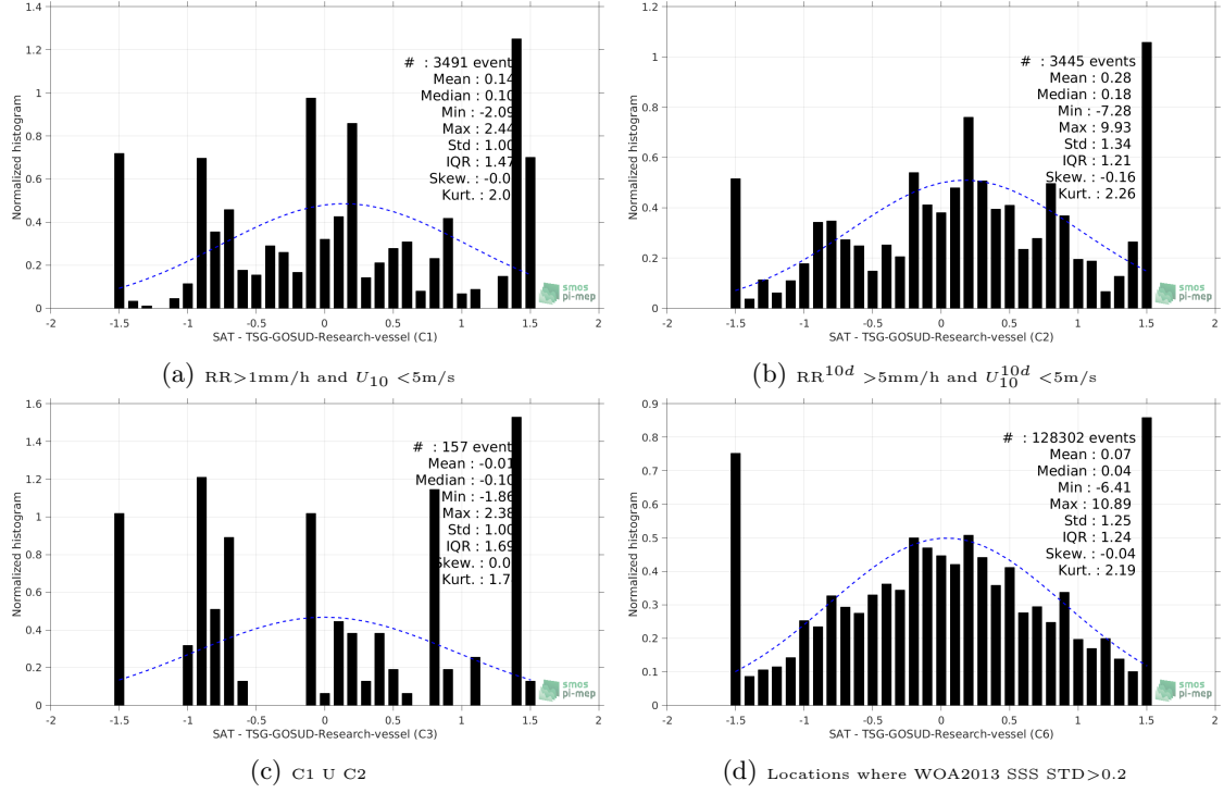
Figure 13: Normalized histogram of \Delta SSS (SMAP-L2-JPL-V4 - TSG-GOSUD-Research-vessel) for 6 different subdatasets corresponding to: RR > 1\text{mm/h} and U_{10} < 5\text{m/s} (a), RR^{10d} > 5\text{mm/h} and U_{10}^{10d} < 5\text{m/s} (b), C1 U C2 (c), Locations where WOA2013 SSS STD > 0.2 (d).
