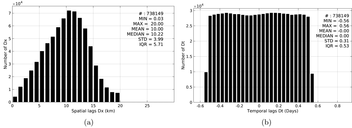
Figure 5: Histograms of the spatial (a) and temporal (b) lags between the time of the TSG-GOSUD-Research-vessel measurements and the date of the corresponding SMAP-L2-JPL-V4 SSS product.
