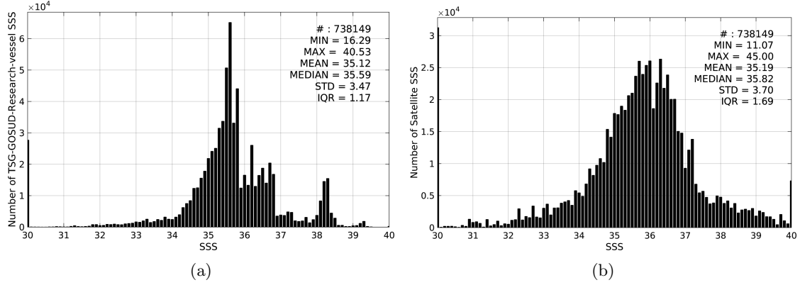
Figure 2: Histograms of SSS from TSG-GOSUD-Research-vessel (a) and SMAP-L2-JPL-V4 (b) considering all match-up pairs per bins of 0.1 over the SMOS coastal zone ( \pm 800\text{km} ) 60^\circ\text{N} - 60^\circ\text{S} Pi-MEP region and for the full satellite product period.
