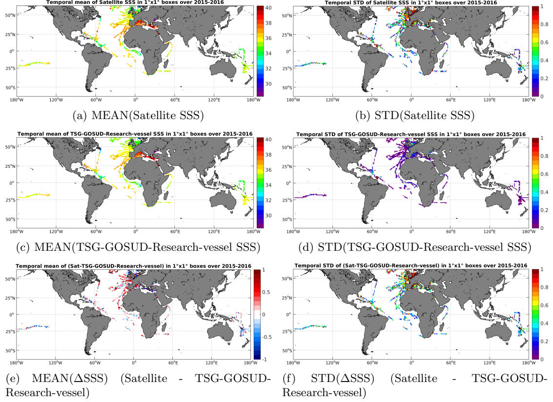
Figure 6: Temporal mean (left) and STD (right) of SSS from SMAP-L2-JPL-V4 (top), TSG-GOSUD-Research-vessel (middle), and of \Delta SSS (Satellite - TSG-GOSUD-Research-vessel). Only match-up pairs are used to generate these maps.
