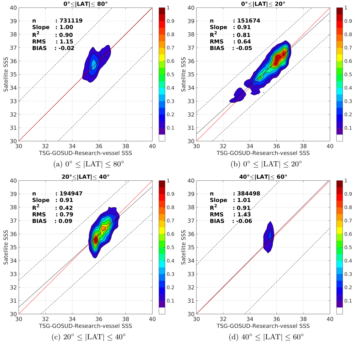
Figure 9: Contour maps of the concentration of SMAP-L2-JPL-V4 SSS (y-axis) versus TSG-GOSUD-Research-vessel SSS (x-axis) at match-up pairs for different latitude bands. For each plot, the red line shows x=y . The black thin and dashed lines indicate a linear fit through the data cloud and the \pm 95\% confidence levels, respectively. The number match-up pairs n , the slope and R^2 coefficient of the linear fit, the root mean square (RMS) and the mean bias between satellite and in situ data are indicated for each latitude band in each plots.
