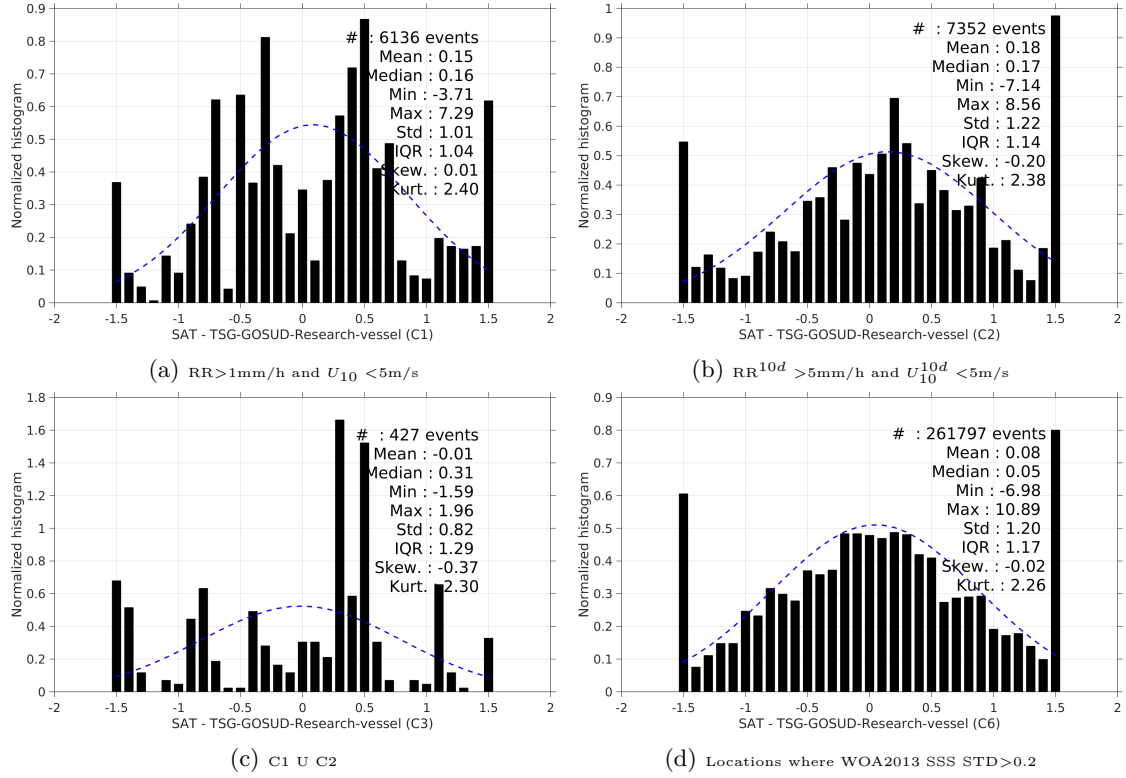
Figure 13: Normalized histogram of \Delta SSS (SMAP-L2-JPL-V4 - TSG-GOSUD-Research-vessel) for 6 different subdatasets corresponding to: RR > 1\text{mm/h} and U_{10} < 5\text{m/s} (a), RR^{10d} > 5\text{mm/h} and U_{10}^{10d} < 5\text{m/s} (b), C1 U C2 (c), Locations where WOA2013 SSS STD > 0.2 (d).
