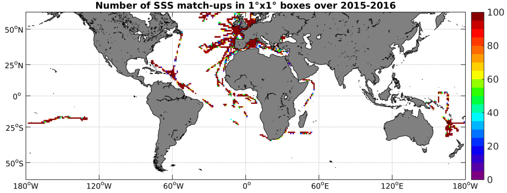
Figure 4: Number of SSS match-ups between TSG-GOSUD-Research-vessel SSS and the SMAP-L2-JPL-V4 SSS product for the SMOS coastal zone ( \leq 800\text{km} ) 60N-60S Pi-MEP region over 1^\circ \times 1^\circ boxes and for the full satellite product period.
