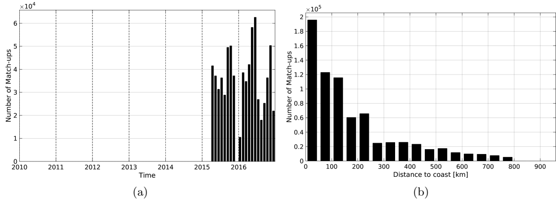
Figure 1: Number of match-ups between TSG-GOSUD-Research-vessel and SMAP-L2-JPL-V4 SSS as a function of time (a) and as function of the distance to coast (b) over the SMOS coastal zone ( \pm 800 km) 60N-60S Pi-MEP region and for the full satellite product period.
