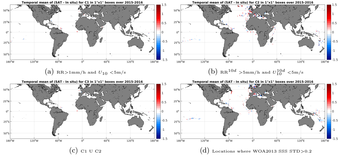
Figure 12: Temporal mean gridded over spatial boxes of size 1^\circ \times 1^\circ of \Delta SSS (SMAP-L2-JPL-V4 - TSG-GOSUD-Research-vessel) for 4 different subdatasets corresponding to: RR > 1mm/h and U_{10} < 5 m/s (a), RR^{10d} > 5 mm/h and U_{10}^{10d} < 5 m/s (b), C1 U C2 (c), Locations where WOA2013 SSS STD > 0.2 (d).
