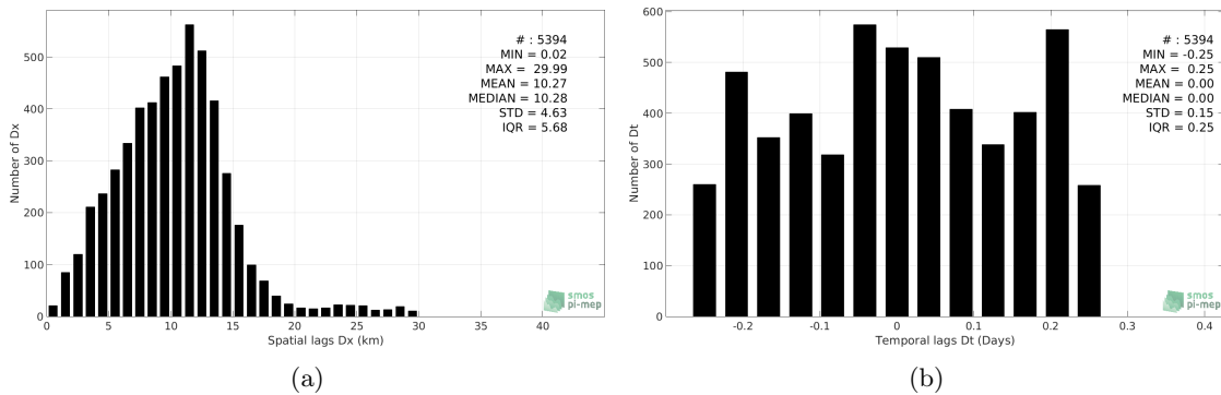
Figure 5: Histograms of the spatial (a) and temporal (b) lags between the time of the Sea mammals measurements and the date of the corresponding SMAP-L2-JPL-V4 SSS product.
