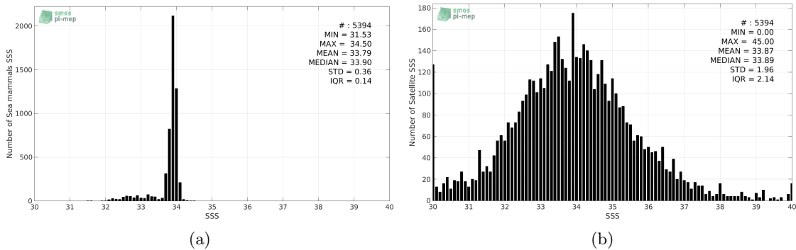
Figure 2: Histograms of SSS from Sea mammals (a) and SMAP-L2-JPL-V4 (b) considering all match-up pairs per bins of 0.1 over the SMOS coastal zone ( \pm 800\text{km} ) 60N-60S Pi-MEP region and for the full satellite product period.
