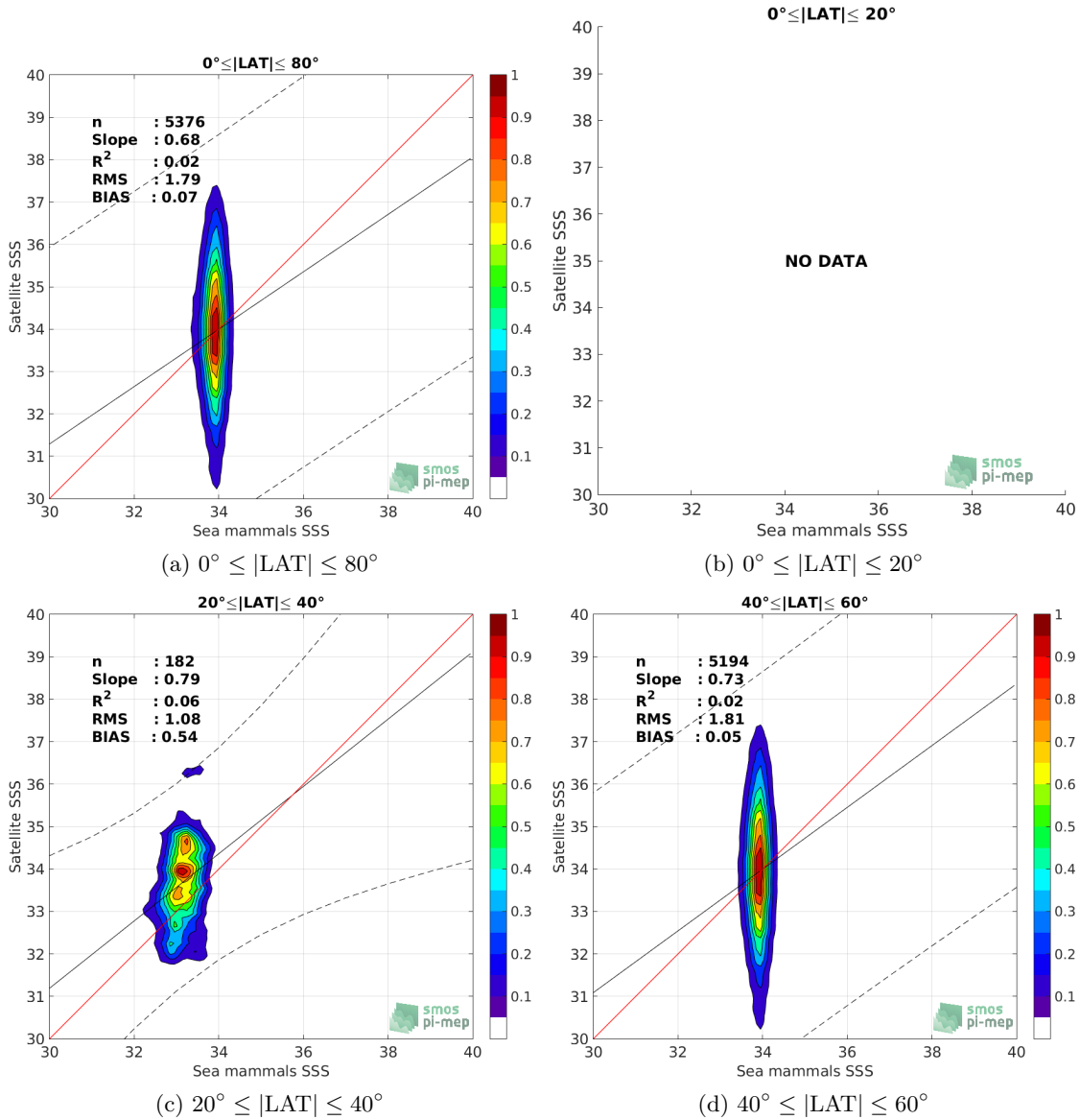
Figure 9: Contour maps of the concentration of SMAP-L2-JPL-V4 SSS (y-axis) versus Sea mammals SSS (x-axis) at match-up pairs for different latitude bands. For each plot, the red line shows x=y . The black thin and dashed lines indicate a linear fit through the data cloud and the \pm 95\% confidence levels, respectively. The number match-up pairs n , the slope and R^2 coefficient of the linear fit, the root mean square (RMS) and the mean bias between satellite and in situ data are indicated for each latitude band in each plots.
