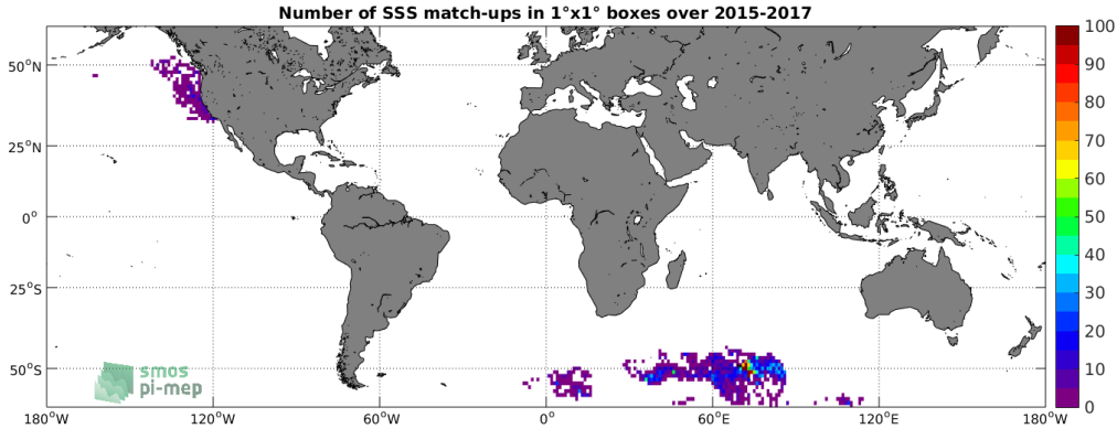
Figure 4: Number of SSS match-ups between Sea mammals SSS and the SMAP-L2-JPL-V4 SSS product for the SMOS coastal zone ( \approx 800\text{km} ) 60N-60S Pi-MEP region over 1^\circ \times 1^\circ boxes and for the full satellite product period.
