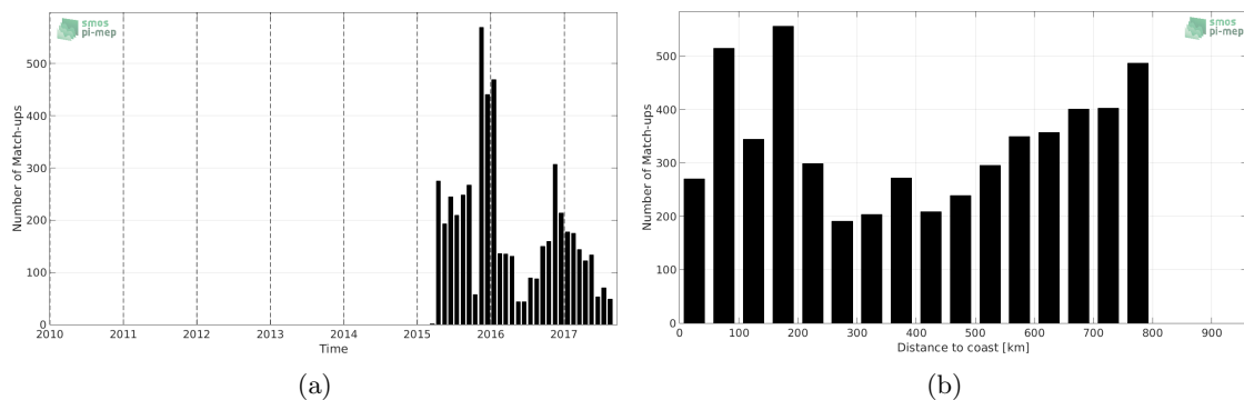
Figure 1: Number of match-ups between Sea mammals and SMAP-L2-JPL-V4 SSS as a function of time (a) and as function of the distance to coast (b) over the SMOS coastal zone ( \pm 800 km) 60N-60S Pi-MEP region and for the full satellite product period.
