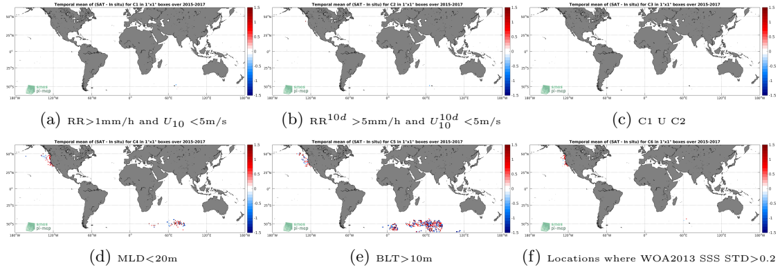
Figure 12: Temporal mean gridded over spatial boxes of size 1^\circ \times 1^\circ of \Delta SSS (SMAP-L2-JPL-V4 - Sea mammals) for 6 different subdatasets corresponding to: RR > 1\text{mm/h} and U_{10} < 5\text{m/s} (a), RR^{10d} > 5\text{mm/h} and U_{10}^{10d} < 5\text{m/s} (b), C1 U C2 (c), MLD < 20\text{m} (d), BLT > 10\text{m} (e), Locations where WOA2013 SSS STD > 0.2 (f).
