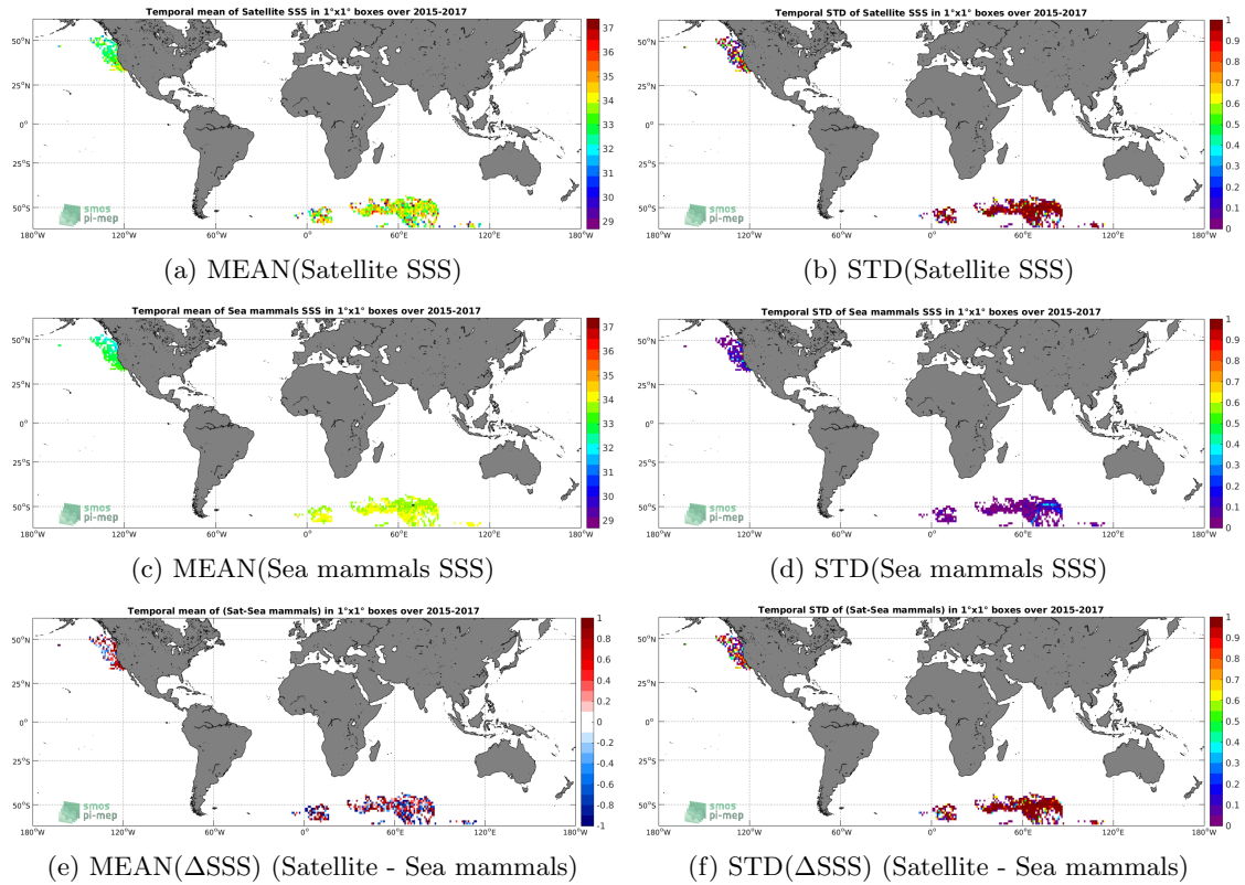
Figure 6: Temporal mean (left) and STD (right) of SSS from SMAP-L2-JPL-V4 (top), Sea mammals (middle), and of \Delta SSS (Satellite - Sea mammals). Only match-up pairs are used to generate these maps.
