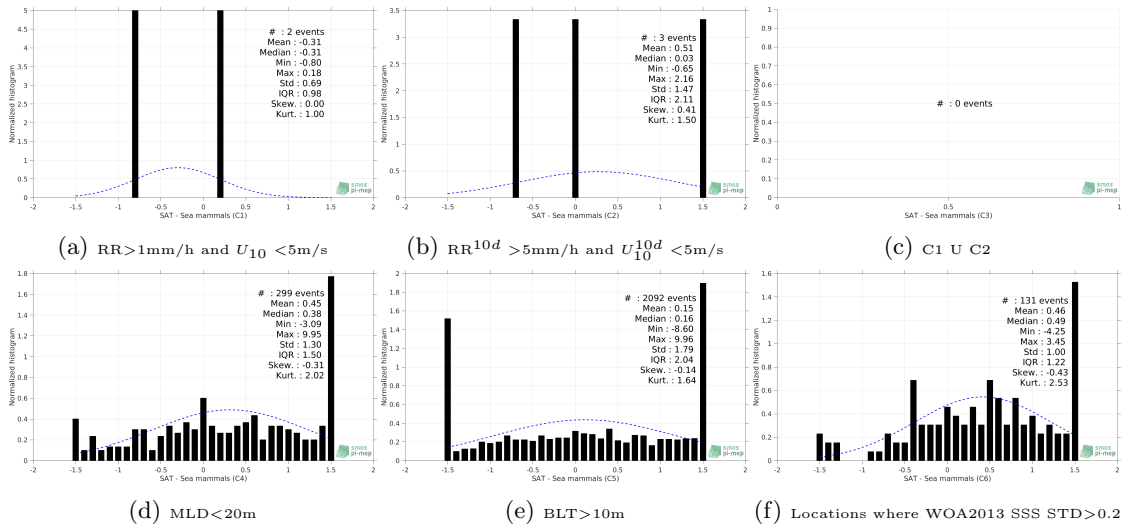
Figure 13: Normalized histogram of \Delta SSS (SMAP-L2-JPL-V4 - Sea mammals) for 6 different subdatasets corresponding to: RR > 1\text{mm/h} and U_{10} < 5\text{m/s} (a), RR^{10d} > 5\text{mm/h} and U_{10}^{10d} < 5\text{m/s} (b), C1 U C2 (c), MLD < 20\text{m} (d), BLT > 10\text{m} (e), Locations where WOA2013 SSS STD > 0.2 (f).
