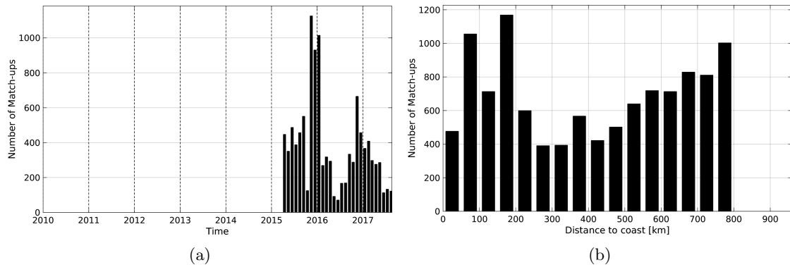
Figure 1: Number of match-ups between Sea mammals and SMAP-L2-JPL-V4 SSS as a function of time (a) and as function of the distance to coast (b) over the SMOS coastal zone ( \pm 800 km) 60N-60S Pi-MEP region and for the full satellite product period.
