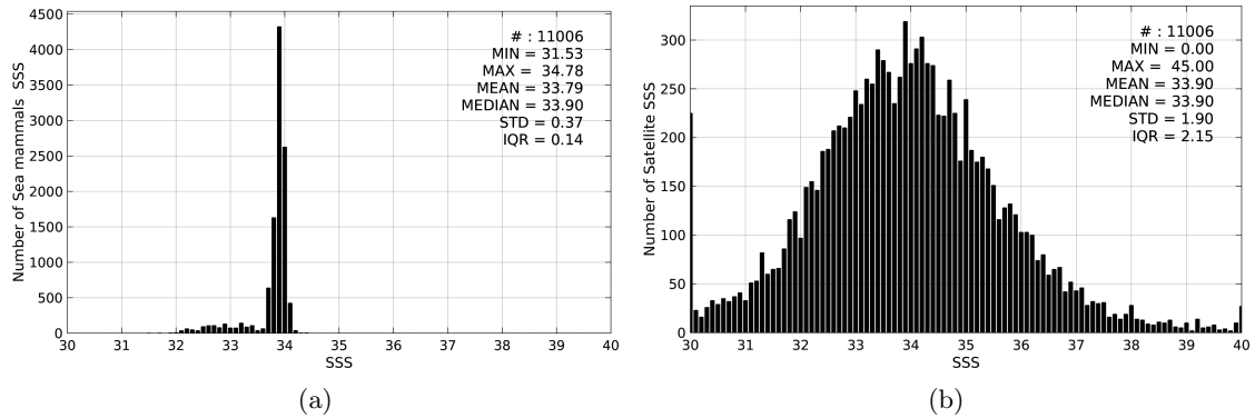
Figure 2: Histograms of SSS from Sea mammals (a) and SMAP-L2-JPL-V4 (b) considering all match-up pairs per bins of 0.1 over the SMOS coastal zone ( \approx 800\text{km} ) 60N-60S Pi-MEP region and for the full satellite product period.
