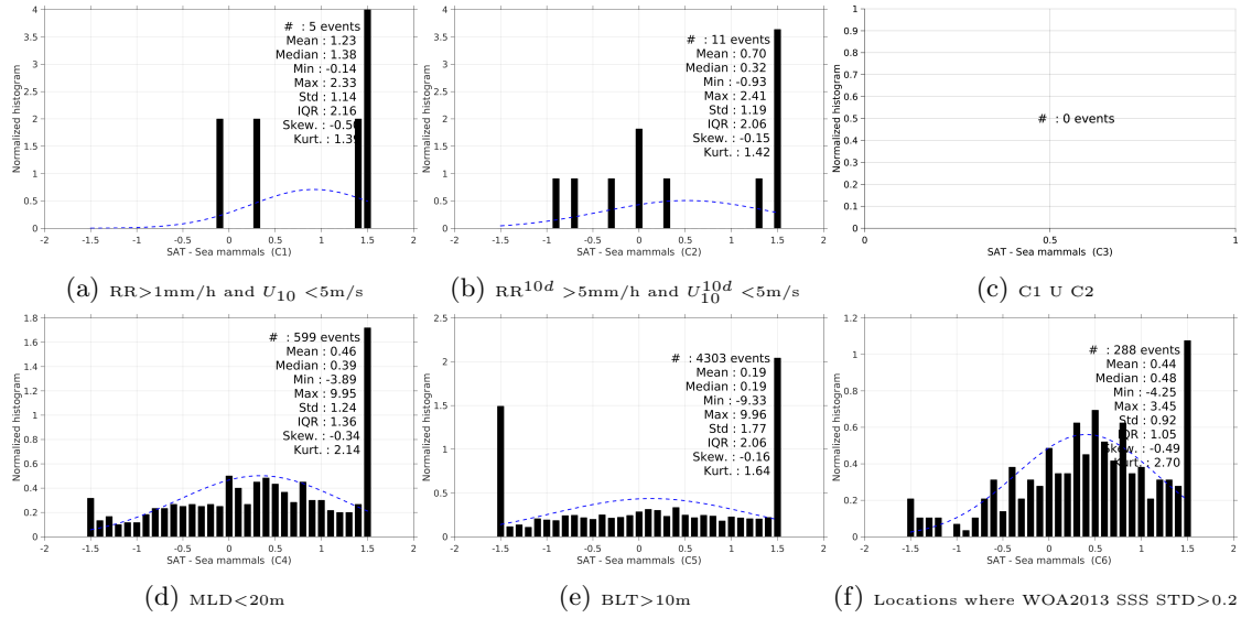
Figure 13: Normalized histogram of \Delta SSS (SMAP-L2-JPL-V4 - Sea mammals) for 6 different sub-datasets corresponding to: RR>1mm/h and U_{10} < 5\text{m/s} (a), RR^{10d} > 5\text{mm/h} and U_{10}^{10d} < 5\text{m/s} (b), C1 U C2 (c),MLD<20m (d),BLT>10m (e),Locations where WOA2013 SSS STD>0.2 (f).
