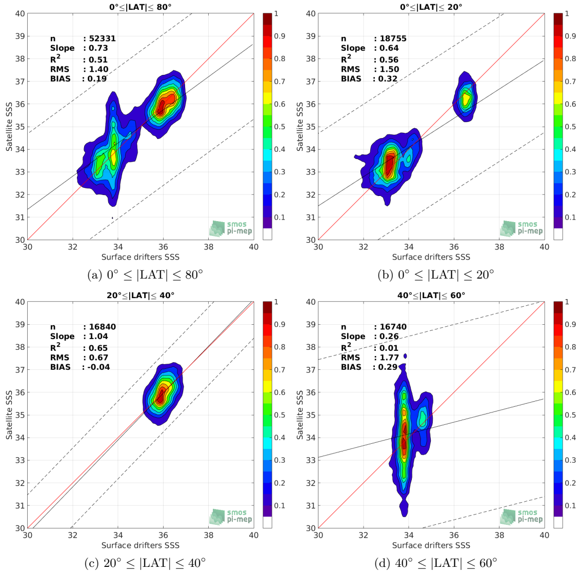
Figure 8: Contour maps of the concentration of SMAP-L2-JPL-V4 SSS (y-axis) versus Surface drifters SSS (x-axis) at match-up pairs for different latitude bands. For each plot, the red line shows x=y . The black thin and dashed lines indicate a linear fit through the data cloud and the \pm 95\% confidence levels, respectively. The number match-up pairs n , the slope and R^2 coefficient of the linear fit, the root mean square (RMS) and the mean bias between satellite and in situ data are indicated for each latitude band in each plots.
