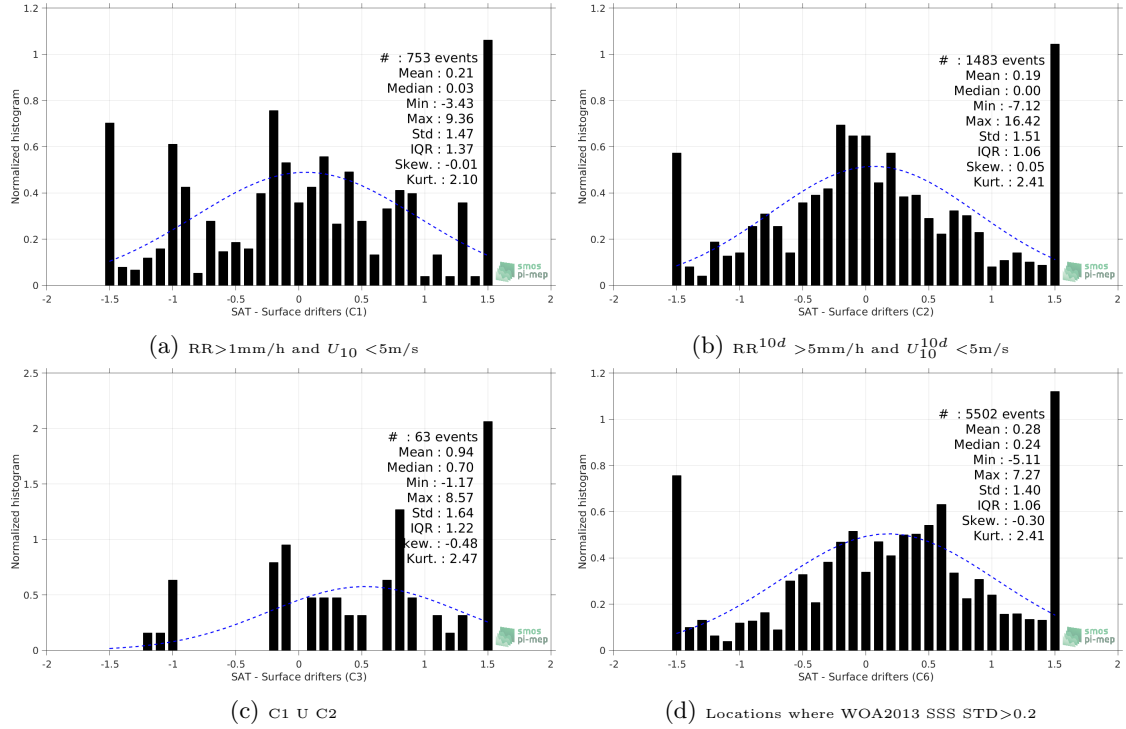
Figure 12: Normalized histogram of \Delta SSS (SMAP-L2-JPL-V4 - Surface drifters) for 6 different subdatasets corresponding to: RR > 1\text{mm/h} and U_{10} < 5\text{m/s} (a), RR^{10d} > 5\text{mm/h} and U_{10}^{10d} < 5\text{m/s} (b), C1 \cup C2 (c), Locations where WOA2013 SSS STD > 0.2 (d).
