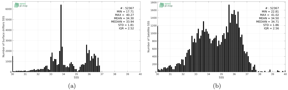
Figure 2: Histograms of SSS from Surface drifters (a) and SMAP-L2-JPL-V4 (b) considering all match-up pairs per bins of 0.1 over the SMOS coastal zone ( \approx 800\text{km} ) 60N-60S Pi-MEP region and for the full satellite product period.
