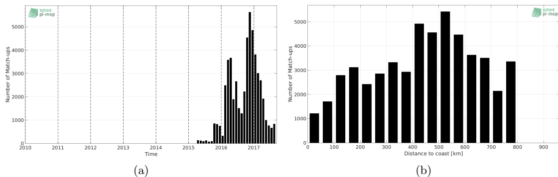
Figure 1: Number of match-ups between Surface drifters and SMAP-L2-JPL-V4 SSS as a function of time (a) and as function of the distance to coast (b) over the SMOS coastal zone ( \pm 800 km) 60N-60S Pi-MEP region and for the full satellite product period.
