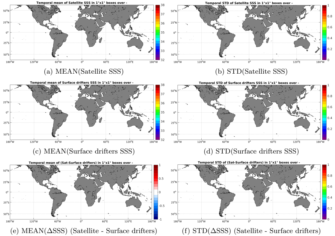
Figure 5: Temporal mean (left) and STD (right) of SSS from SMAP-L2-JPL-V4 (top), Surface drifters (middle), and of \Delta SSS (Satellite - Surface drifters). Only match-up pairs are used to generate these maps.
