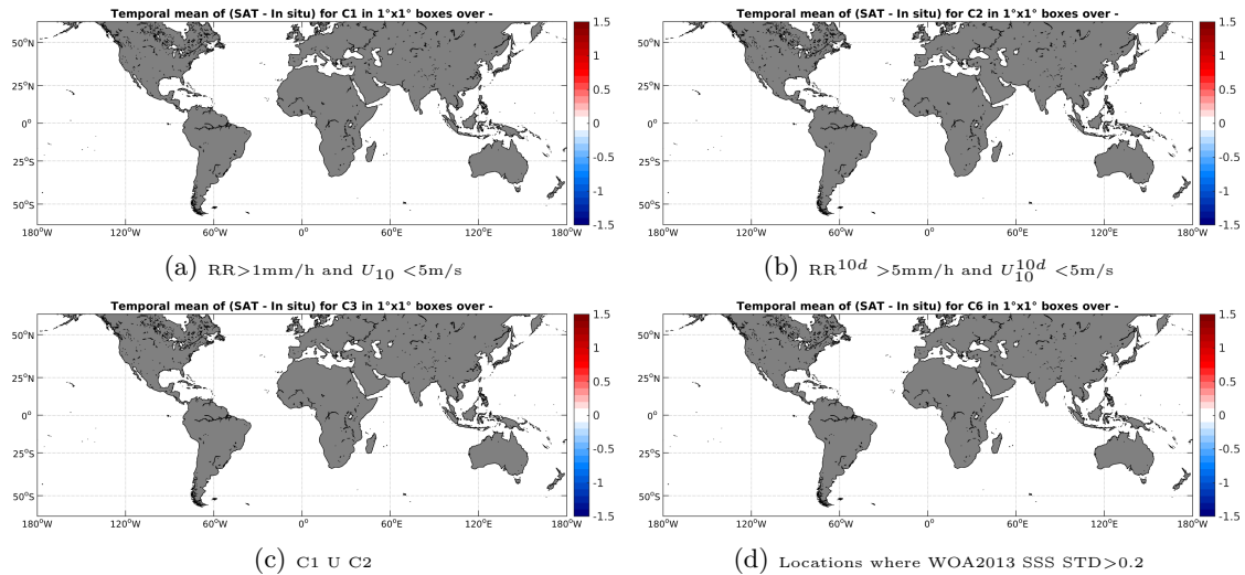
Figure 11: Temporal mean gridded over spatial boxes of size 1^\circ \times 1^\circ of \Delta SSS (SMAP-L2-JPL-V4 - Surface drifters) for 4 different subdatasets corresponding to: RR > 1 mm/h and U_{10} < 5 m/s (a), RR ^{10d} > 5 mm/h and U_{10}^{10d} < 5 m/s (b), C1 U C2 (c), Locations where WOA2013 SSS STD > 0.2 (d).
