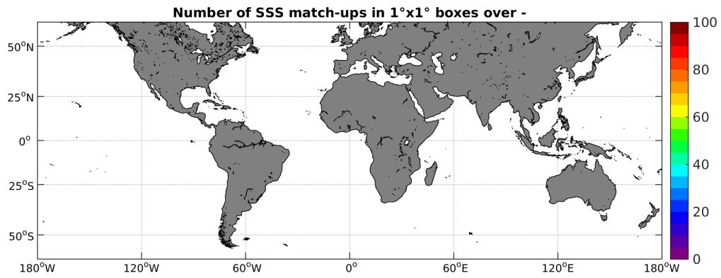
Figure 3: Number of SSS match-ups between Surface drifters SSS and the SMAP-L2-JPL-V4 SSS product for the SMOS coastal zone ( \approx 800\text{km} ) 60N-60S Pi-MEP region over 1^\circ \times 1^\circ boxes and for the full satellite product period.
