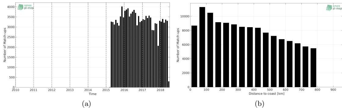
Figure 1: Number of match-ups between Argo and SMAP-L2-JPL-V4 SSS as a function of time (a) and as function of the distance to coast (b) over the SMOS coastal zone ( \pm 800 km) 60N-60S Pi-MEP region and for the full satellite product period.
