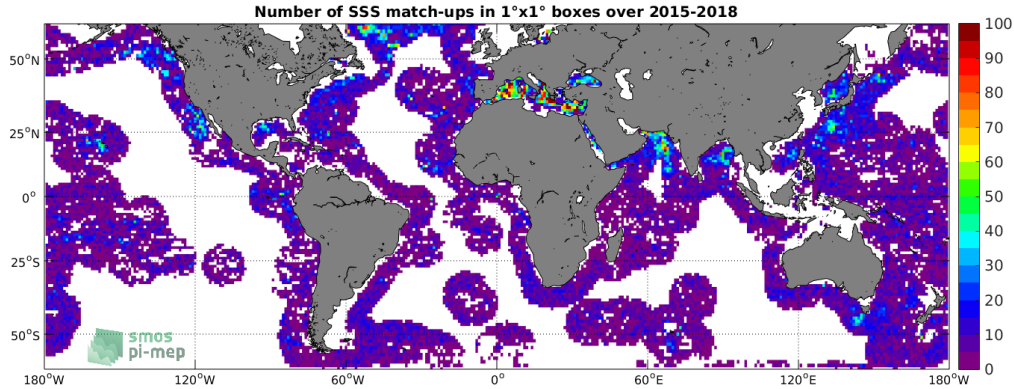
Figure 4: Number of SSS match-ups between Argo SSS and the SMAP-L2-JPL-V4 SSS product for the SMOS coastal zone ( \approx 800\text{km} ) 60N-60S Pi-MEP region over 1^\circ \times 1^\circ boxes and for the full satellite product period.
