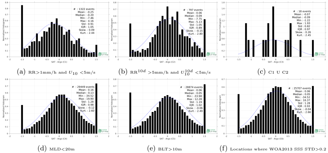
Figure 13: Normalized histogram of \Delta SSS (SMAP-L2-JPL-V4 - Argo) for 6 different subdatasets corresponding to: RR>1mm/h and U_{10} <5m/s (a), RR^{10d} >5mm/h and U_{10}^{10d} <5m/s (b), C1 U C2 (c),MLD<20m (d),BLT>10m (e),Locations where WOA2013 SSS STD>0.2 (f).
