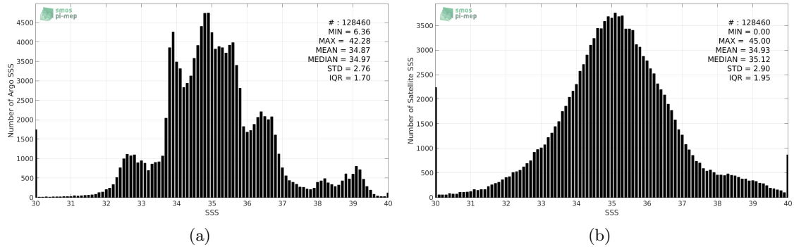
Figure 2: Histograms of SSS from Argo (a) and SMAP-L2-JPL-V4 (b) considering all match-up pairs per bins of 0.1 over the SMOS coastal zone ( \geq 800\text{km} ) 60N-60S Pi-MEP region and for the full satellite product period.
