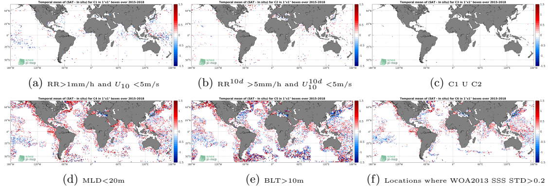
Figure 12: Temporal mean gridded over spatial boxes of size 1°x1° of \Delta SSS (SMAP-L2-JPL-V4 - Argo) for 6 different subdatasets corresponding to:RR>1mm/h and U_{10} <5m/s (a), RR^{10d} >5mm/h and U_{10}^{10d} <5m/s (b), C1 U C2 (c),MLD<20m (d),BLT>10m (e),Locations where WOA2013 SSS STD>0.2 (f).
