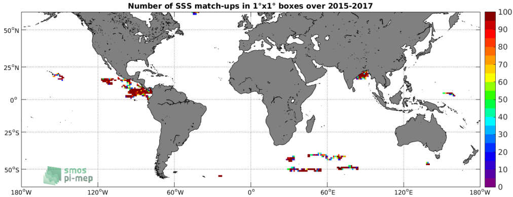
Figure 3: Number of SSS match-ups between Surface drifters SSS and the SMAP-L2-JPL-V4.2 SSS product for the SMOS coastal zone ( \geq 800\text{km} ) 60N-60S Pi-MEP region over 1^\circ \times 1^\circ boxes and for the full satellite product period.
