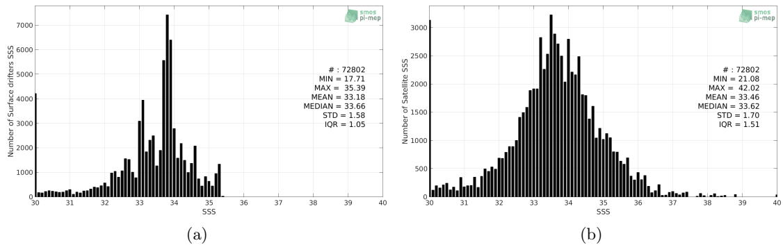
Figure 2: Histograms of SSS from Surface drifters (a) and SMAP-L2-JPL-V4.2 (b) considering all match-up pairs per bins of 0.1 over the SMOS coastal zone ( \pm 800 km) 60N-60S Pi-MEP region and for the full satellite product period.
