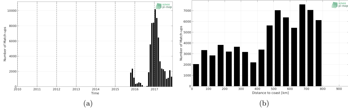
Figure 1: Number of match-ups between Surface drifters and SMAP-L2-JPL-V4.2 SSS as a function of time (a) and as function of the distance to coast (b) over the SMOS coastal zone ( \pm 800 km) 60N-60S Pi-MEP region and for the full satellite product period.
