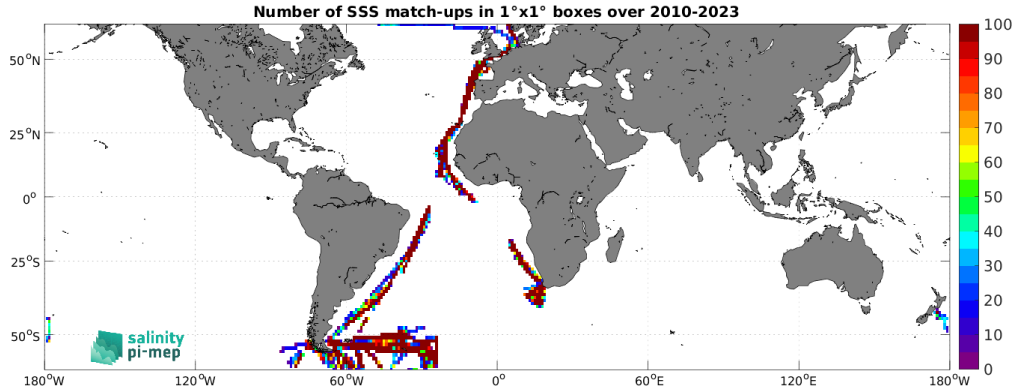
Figure 5: Number of SSS match-ups between TSG (Polarstern) SSS and the ISAS v7 - Monthly (Ifremer-LOPS-CMEMS) SSS product for the SMOS coastal zone (<800km) 60N-60S Pi-MEP region over 1^{\circ} \times 1^{\circ} boxes and for the full satellite product period.
