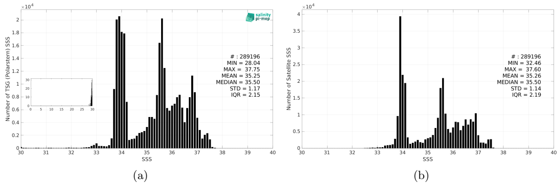
Figure 3: Histograms of SSS from TSG (Polarstern) (a) and ISAS v7 - Monthly (Ifremer-LOPS-CMEMS) (b) considering all match-up pairs per bins of 0.1 over the SMOS coastal zone (<800km) 60N-60S Pi-MEP region and for the full satellite product period.
