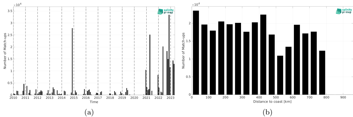
Figure 2: Number of match-ups between TSG (Polarstern) and ISAS v7 - Monthly (Ifremer-LOPS-CMEMS) SSS as a function of time (a) and as function of the distance to coast (b) over the SMOS coastal zone (<800km) 60N-60S Pi-MEP region and for the full satellite product period.
