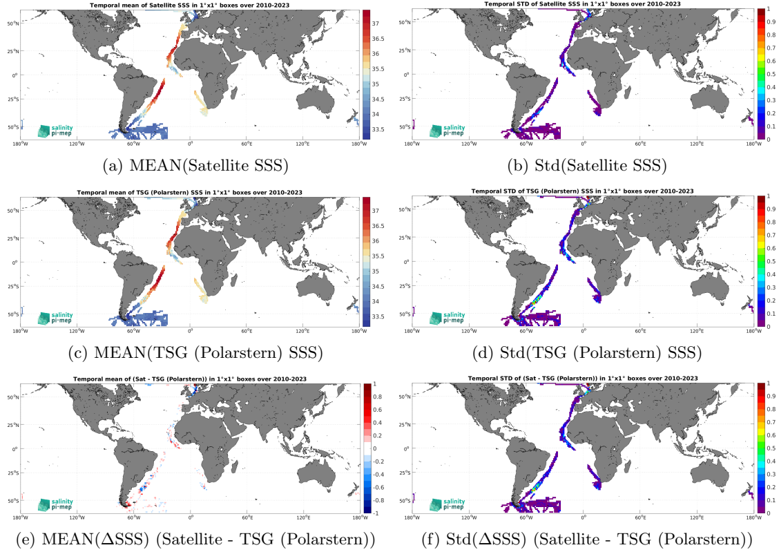
Figure 7: Temporal mean (left) and Std (right) of SSS from ISAS v7 - Monthly (Ifremer-LOPS-CMEMS) (top), TSG (Polarstern) (middle), and of \Delta SSS (Satellite - TSG (Polarstern)). Only match-up pairs are used to generate these maps.
