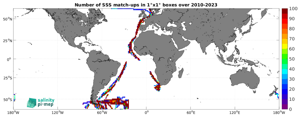
Figure 5: Number of SSS match-ups between TSG (Polarstern) SSS and the ISAS SSS product for the SMOS coastal zone (<800km) 60N-60S Pi-MEP region over 1^\circ \times 1^\circ boxes and for the full satellite product period.
