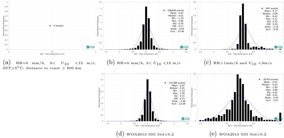
Figure 15: Normalized histogram of \Delta SSS (ISAS - TSG (Polarstern)) for 5 different subdatasets corresponding to: RR=0 mm/h, 3 < U_{10} < 12 m/s, SST > 5°C, distance to coast > 800 km (a), RR=0 mm/h, 3 < U_{10} < 12 m/s (b), RR > 1mm/h and U_{10} < 4 m/s (c), WOA2013 SSS Std < 0.2 (d), WOA2013 SSS Std > 0.2 (e).
