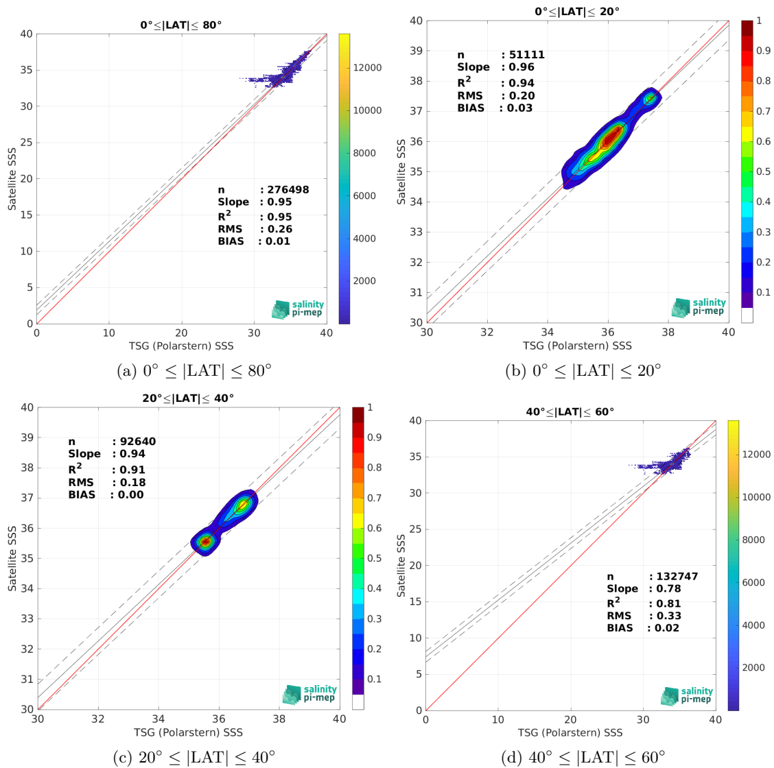
Figure 10: Contour maps of the concentration of ISAS SSS (y-axis) versus TSG (Polarstern) SSS (x-axis) at match-up pairs for different latitude bands. For each plot, the red line shows x=y . The black thin and dashed lines indicate a linear fit through the data cloud and the \pm 95\% confidence levels, respectively. The number match-up pairs n , the slope and R^2 coefficient of the linear fit, the root mean square (RMS) and the mean bias between satellite and in situ data are indicated for each latitude band in each plots.
