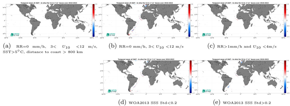
Figure 14: Temporal mean gridded over spatial boxes of size 1^\circ \times 1^\circ of \Delta SSS (ISAS - TSG (Polarstern)) for 5 different subdatasets corresponding to:RR=0 mm/h, 3 < U_{10} < 12 m/s, SST >5^\circ C, distance to coast > 800 km (a), RR=0 mm/h, 3 < U_{10} < 12 m/s (b), RR >1 mm/h and U_{10} < 4 m/s (c), WOA2013 SSS Std <0.2 (d), WOA2013 SSS Std >0.2 (e).
