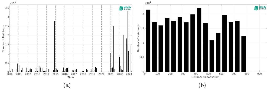
Figure 2: Number of match-ups between TSG (Polarstern) and ISAS SSS as a function of time (a) and as function of the distance to coast (b) over the SMOS coastal zone (<800km) 60N-60S Pi-MEP region and for the full satellite product period.
