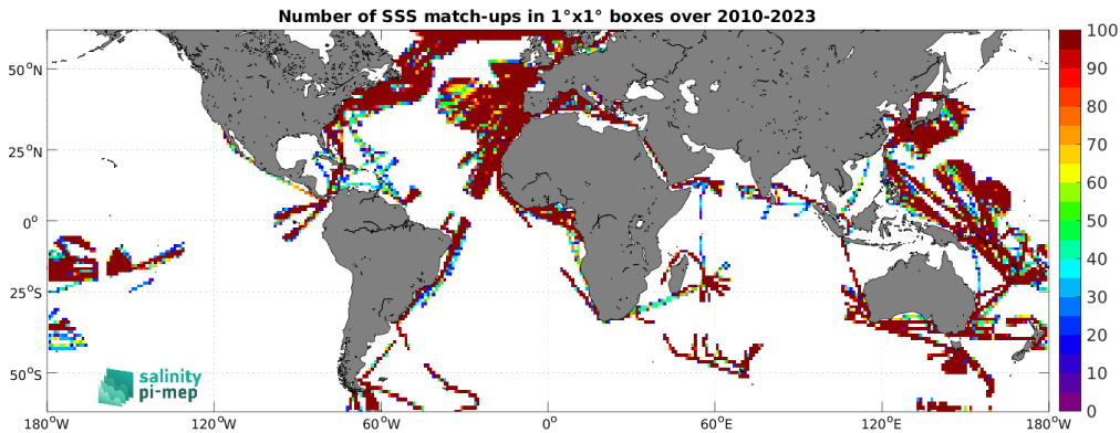
Figure 5: Number of SSS match-ups between TSG (LEGOS-DM) SSS and the ISAS SSS product for the SMOS coastal zone (<800km) 60N-60S Pi-MEP region over 1°×1° boxes and for the full satellite product period.
