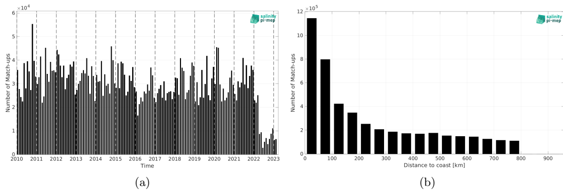
Figure 2: Number of match-ups between TSG (LEGOS-DM) and ISAS SSS as a function of time (a) and as function of the distance to coast (b) over the SMOS coastal zone (<800km) 60N-60S Pi-MEP region and for the full satellite product period.
