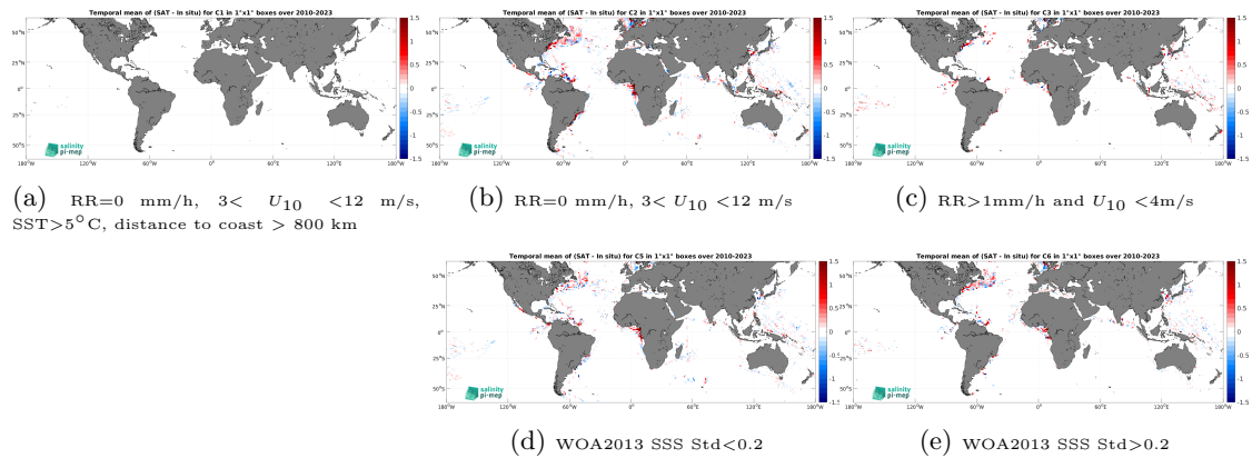
Figure 14: Temporal mean gridded over spatial boxes of size 1^\circ \times 1^\circ of \Delta SSS (ISAS - TSG (LEGOS-DM)) for 5 different subdatasets corresponding to:RR=0 mm/h, 3 < U_{10} < 12 m/s, SST >5^\circ\text{C} , distance to coast > 800 km (a), RR=0 mm/h, 3 < U_{10} < 12 m/s (b), RR >1 mm/h and U_{10} < 4 m/s (c), WOA2013 SSS Std <0.2 (d), WOA2013 SSS Std >0.2 (e).
