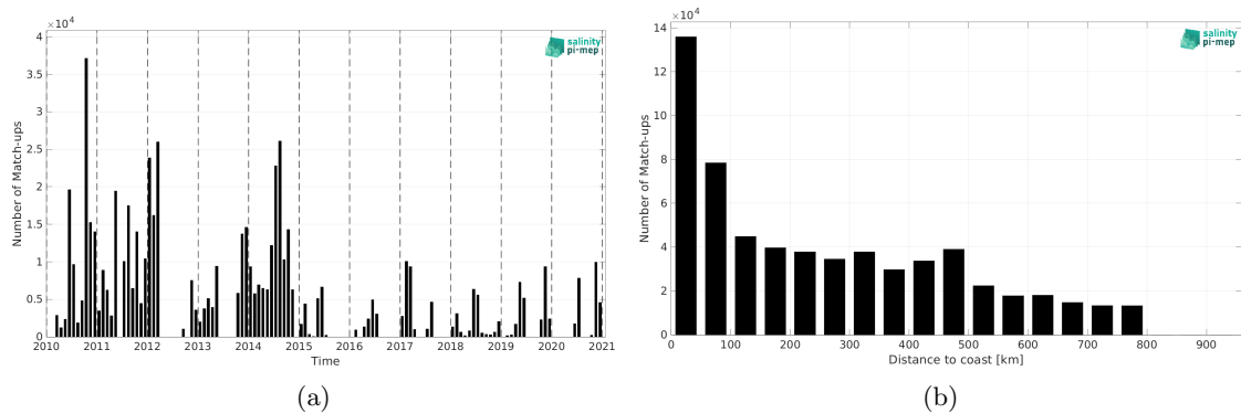
Figure 2: Number of match-ups between TSG (GOSUD-Sailing-ship) and ISAS SSS as a function of time (a) and as function of the distance to coast (b) over the SMOS coastal zone (<800km) 60N-60S Pi-MEP region and for the full satellite product period.
