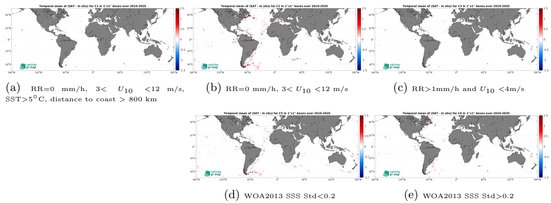
Figure 14: Temporal mean gridded over spatial boxes of size 1^\circ \times 1^\circ of \Delta SSS (ISAS - TSG (GOSUD-Sailing-ship)) for 5 different subdatasets corresponding to:RR=0 mm/h, 3 < U_{10} < 12 m/s, SST > 5°C, distance to coast > 800 km (a), RR=0 mm/h, 3 < U_{10} < 12 m/s (b), RR > 1mm/h and U_{10} < 4 m/s (c), WOA2013 SSS Std < 0.2 (d), WOA2013 SSS Std > 0.2 (e).
