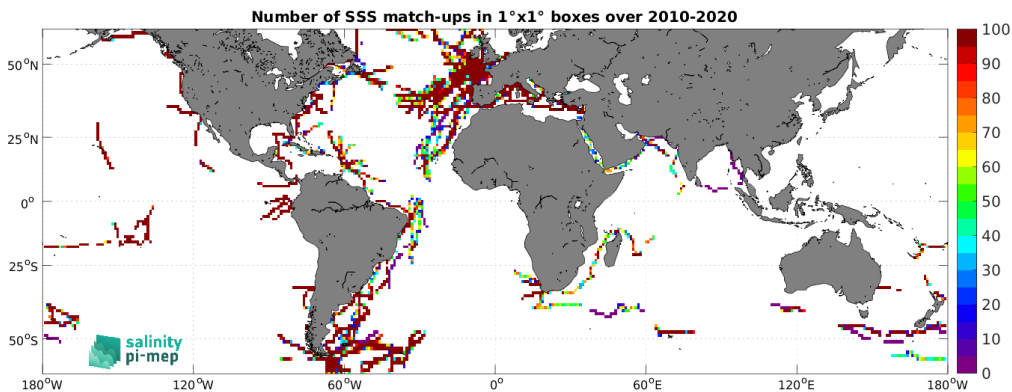
Figure 5: Number of SSS match-ups between TSG (GOSUD-Sailing-ship) SSS and the ISAS SSS product for the SMOS coastal zone (<800km) 60N-60S Pi-MEP region over 1^\circ \times 1^\circ boxes and for the full satellite product period.
