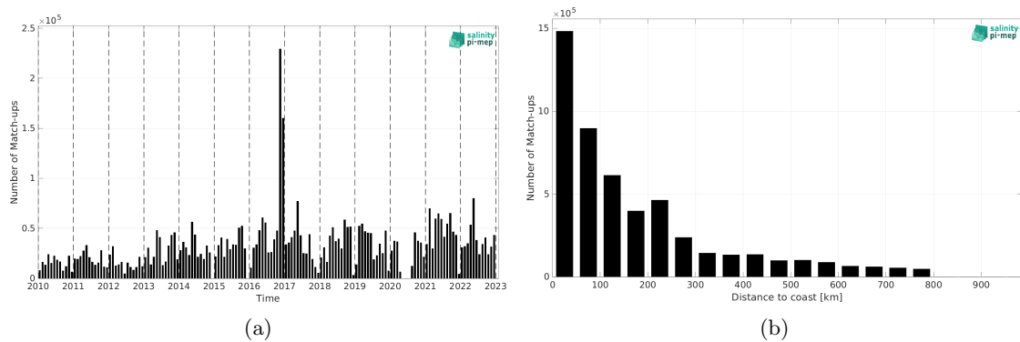
Figure 2: Number of match-ups between TSG (GOSUD-Research-vessel) and ISAS v7 - Monthly (Ifremer-LOPS-CMEMS) SSS as a function of time (a) and as function of the distance to coast (b) over the SMOS coastal zone (<800km) 60N-60S Pi-MEP region and for the full satellite product period.
