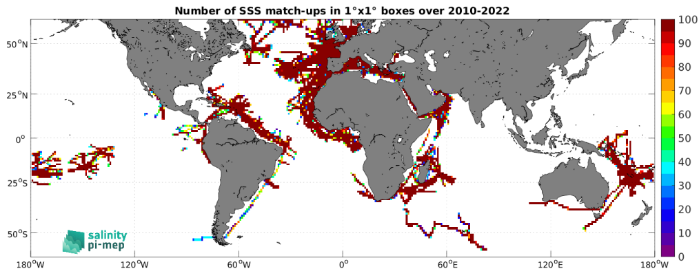
Figure 5: Number of SSS match-ups between TSG (GOSUD-Research-vessel) SSS and the ISAS v7 - Monthly (Ifremer-LOPS-CMEMS) SSS product for the SMOS coastal zone (<800km) 60N-60S Pi-MEP region over 1^\circ \times 1^\circ boxes and for the full satellite product period.
