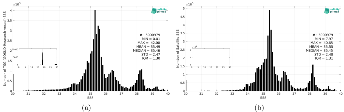
Figure 3: Histograms of SSS from TSG (GOSUD-Research-vessel) (a) and ISAS v7 - Monthly (Ifremer-LOPS-CMEMS) (b) considering all match-up pairs per bins of 0.1 over the SMOS coastal zone (<800km) 60N-60S Pi-MEP region and for the full satellite product period.
