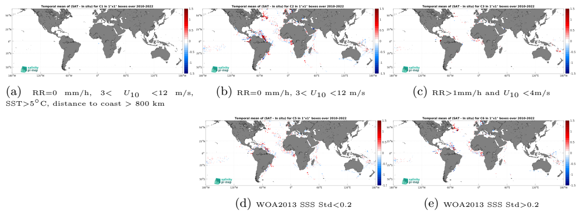
Figure 14: Temporal mean gridded over spatial boxes of size 1^\circ \times 1^\circ of \Delta SSS (ISAS v7 - Monthly (Ifremer-LOPS-CMEMS) - TSG (GOSUD-Research-vessel)) for 5 different subdatasets corresponding to:RR=0 mm/h, 3 < U_{10} < 12 m/s, SST >5^\circ\text{C} , distance to coast > 800 km (a), RR=0 mm/h, 3 < U_{10} < 12 m/s (b), RR >1 mm/h and U_{10} < 4 m/s (c), WOA2013 SSS Std <0.2 (d), WOA2013 SSS Std >0.2 (e).
