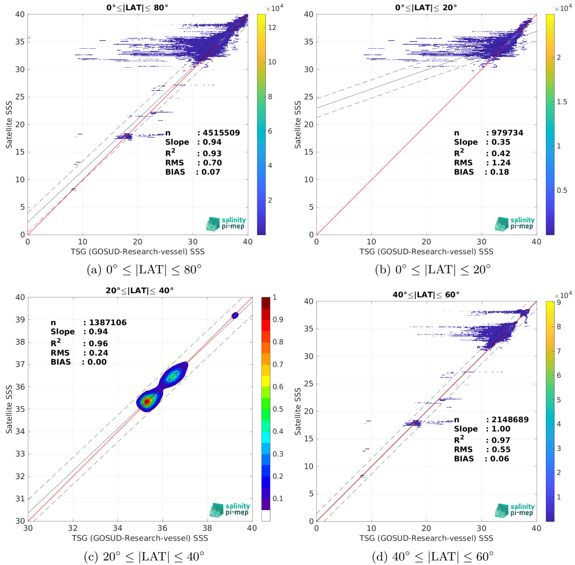
Figure 10: Contour maps of the concentration of ISAS SSS (y-axis) versus TSG (GOSUD-Research-vessel) SSS (x-axis) at match-up pairs for different latitude bands. For each plot, the red line shows x=y . The black thin and dashed lines indicate a linear fit through the data cloud and the \pm 95\% confidence levels, respectively. The number match-up pairs n , the slope and R^2 coefficient of the linear fit, the root mean square (RMS) and the mean bias between satellite and in situ data are indicated for each latitude band in each plots.
