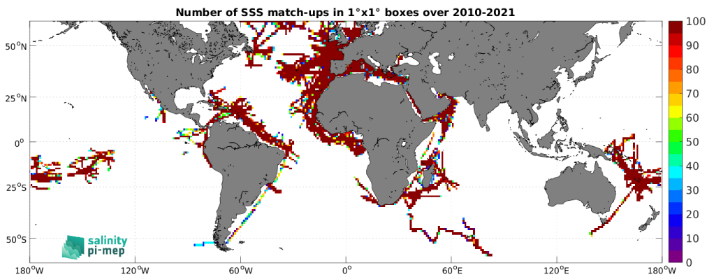
Figure 5: Number of SSS match-ups between TSG (GOSUD-Research-vessel) SSS and the ISAS SSS product for the SMOS coastal zone (<800km) 60N-60S Pi-MEP region over 1^\circ \times 1^\circ boxes and for the full satellite product period.
