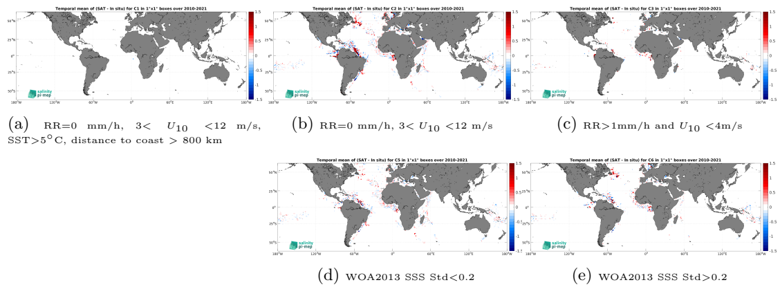
Figure 14: Temporal mean gridded over spatial boxes of size 1^\circ \times 1^\circ of \Delta SSS (ISAS - TSG (GOSUD-Research-vessel)) for 5 different subdatasets corresponding to:RR=0 mm/h, 3 < U_{10} < 12 m/s, SST>5°C, distance to coast > 800 km (a), RR=0 mm/h, 3 < U_{10} < 12 m/s (b), RR>1mm/h and U_{10} < 4 m/s (c), WOA2013 SSS Std<0.2 (d), WOA2013 SSS Std>0.2 (e).
