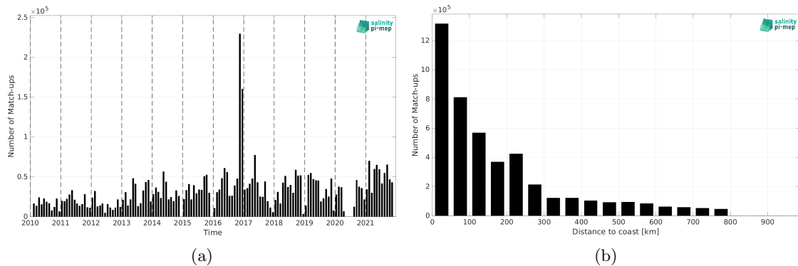
Figure 2: Number of match-ups between TSG (GOSUD-Research-vessel) and ISAS SSS as a function of time (a) and as function of the distance to coast (b) over the SMOS coastal zone (<800km) 60N-60S Pi-MEP region and for the full satellite product period.
