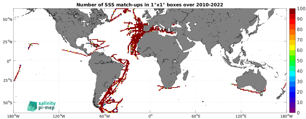
Figure 5: Number of SSS match-ups between TSG (CSIC-UTM) SSS and the ISAS SSS product for the SMOS coastal zone (<800km) 60N-60S Pi-MEP region over 1^\circ \times 1^\circ boxes and for the full satellite product period.
