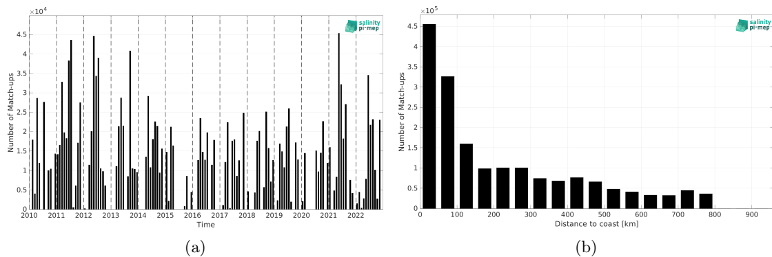
Figure 2: Number of match-ups between TSG (CSIC-UTM) and ISAS SSS as a function of time (a) and as function of the distance to coast (b) over the SMOS coastal zone (<800km) 60N-60S Pi-MEP region and for the full satellite product period.
