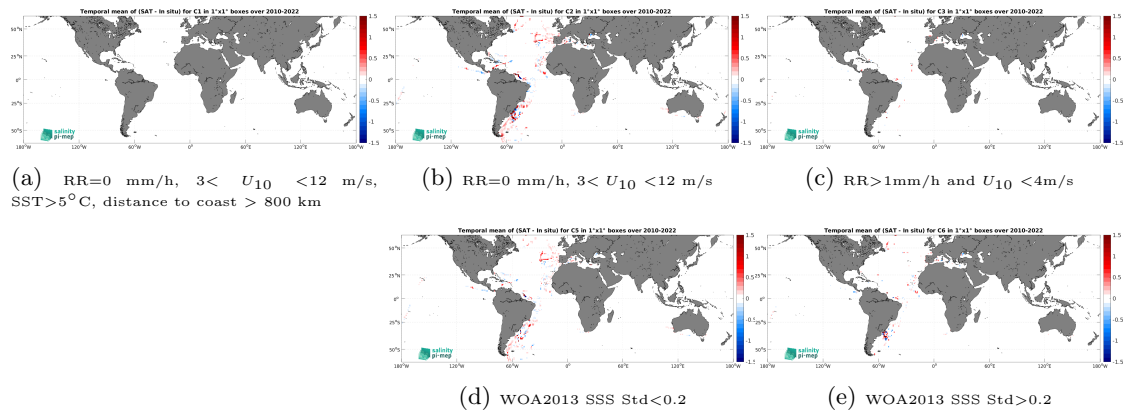
Figure 14: Temporal mean gridded over spatial boxes of size 1^\circ \times 1^\circ of \Delta SSS (ISAS - TSG (CSIC-UTM)) for 5 different subdatasets corresponding to:RR=0 mm/h, 3 < U_{10} < 12 m/s, SST >5^\circ C, distance to coast > 800 km (a), RR=0 mm/h, 3 < U_{10} < 12 m/s (b), RR >1 mm/h and U_{10} < 4 m/s (c), WOA2013 SSS Std <0.2 (d), WOA2013 SSS Std >0.2 (e).
