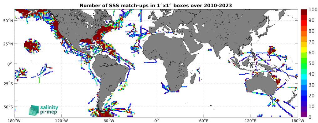
Figure 5: Number of SSS match-ups between TSG (SAMOS) SSS and the CCI SSS L4 Merged-OI v5.5 - 7-day running (ESA) SSS product for the SMOS coastal zone (<800km) 60N-60S Pi-MEP region over 1^\circ \times 1^\circ boxes and for the full satellite product period.
