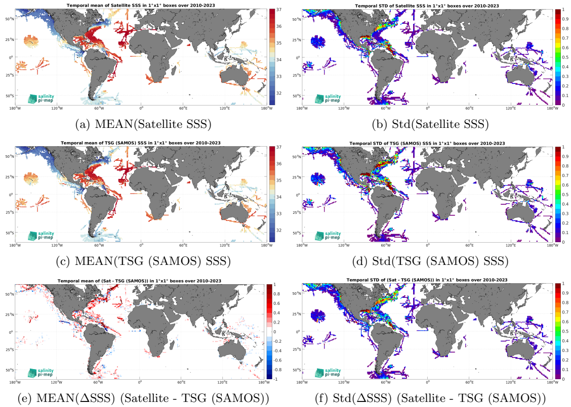
Figure 7: Temporal mean (left) and Std (right) of SSS from CCI SSS L4 Merged-OI v5.5 - 7-day running (ESA) (top), TSG (SAMOS) (middle), and of \Delta SSS (Satellite - TSG (SAMOS)). Only match-up pairs are used to generate these maps.
