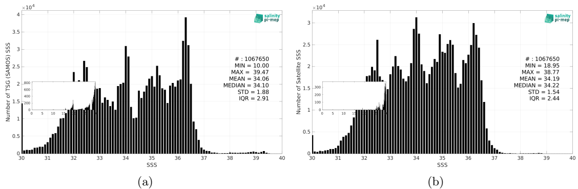
Figure 3: Histograms of SSS from TSG (SAMOS) (a) and CCI SSS L4 Merged-OI v5.5 - 7-day running (ESA) (b) considering all match-up pairs per bins of 0.1 over the SMOS coastal zone (<800km) 60N-60S Pi-MEP region and for the full satellite product period.
