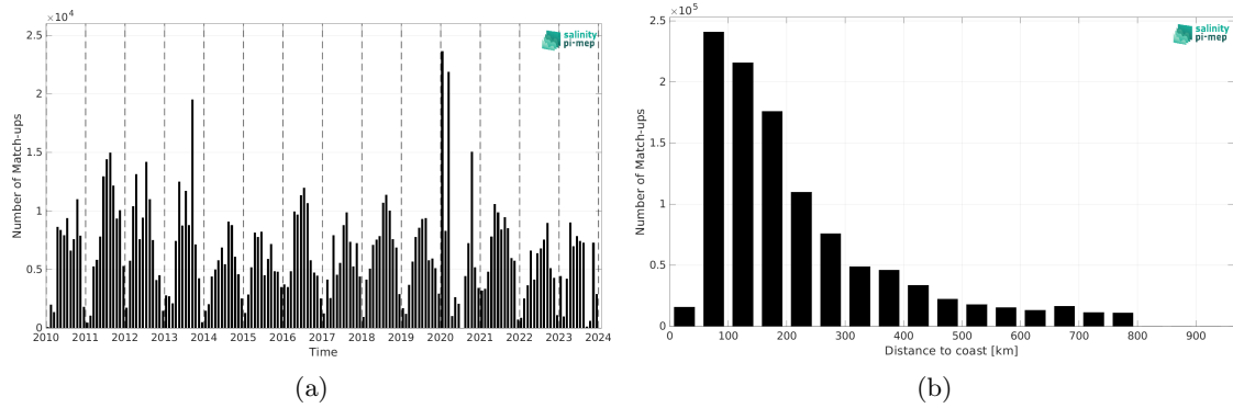
Figure 2: Number of match-ups between TSG (SAMOS) and CCI SSS L4 Merged-OI v5.5 - 7-day running (ESA) SSS as a function of time (a) and as function of the distance to coast (b) over the SMOS coastal zone (<800km) 60N-60S Pi-MEP region and for the full satellite product period.
