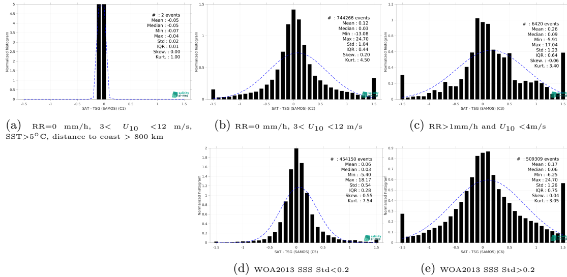
Figure 15: Normalized histogram of \Delta SSS (CCI SSS L4 Merged-OI v5.5 - 7-day running (ESA) - TSG (SAMOS)) for 5 different subdatasets corresponding to: RR=0 mm/h, 3 < U_{10} < 12 m/s, SST > 5°C, distance to coast > 800 km (a), RR=0 mm/h, 3 < U_{10} < 12 m/s (b), RR > 1mm/h and U_{10} < 4 m/s (c), WOA2013 SSS Std < 0.2 (d), WOA2013 SSS Std > 0.2 (e).
