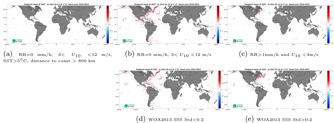
Figure 14: Temporal mean gridded over spatial boxes of size 1^\circ \times 1^\circ of \Delta\text{SSS} (CCI SSS L4 Merged-OI v5.5 - 7-day running (ESA) - TSG (SAMOS)) for 5 different subdatasets corresponding to:RR=0 mm/h, 3 < U_{10} < 12 m/s, SST >5^\circ\text{C} , distance to coast > 800 km (a), RR=0 mm/h, 3 < U_{10} < 12 m/s (b), RR >1 mm/h and U_{10} < 4 m/s (c), WOA2013 SSS Std <0.2 (d), WOA2013 SSS Std >0.2 (e).
