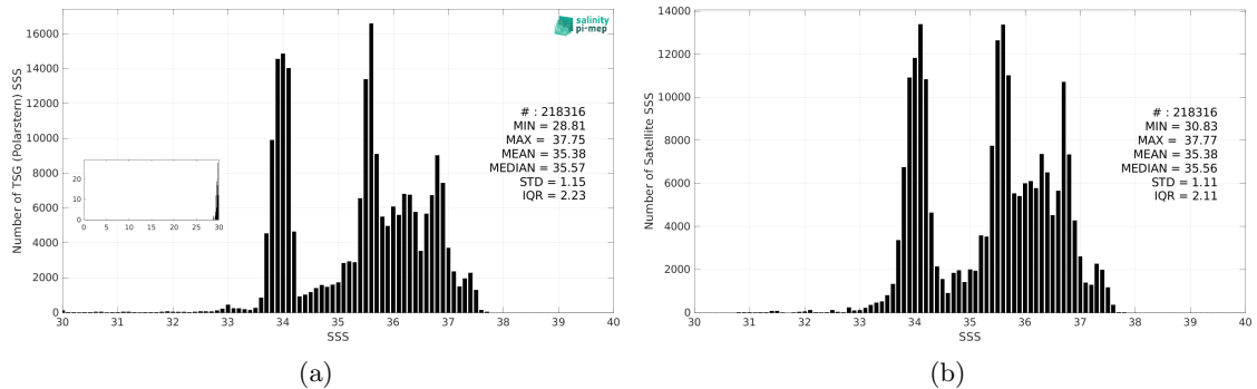
Figure 3: Histograms of SSS from TSG (Polarstern) (a) and CCI SSS L4 Merged-OI v5.5 - 7-day running (ESA) (b) considering all match-up pairs per bins of 0.1 over the SMOS coastal zone (<800km) 60N-60S Pi-MEP region and for the full satellite product period.
