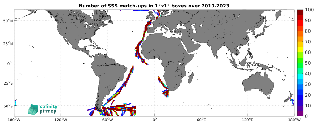
Figure 5: Number of SSS match-ups between TSG (Polarstern) SSS and the CCI SSS L4 Merged-OI v5.5 - 7-day running (ESA) SSS product for the SMOS coastal zone ( <800\text{km} ) 60N-60S Pi-MEP region over 1^\circ \times 1^\circ boxes and for the full satellite product period.
