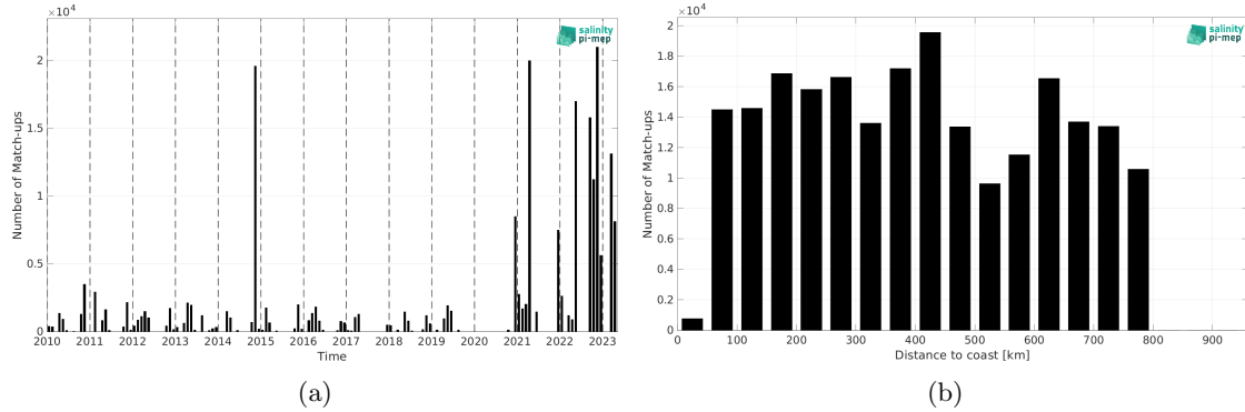
Figure 2: Number of match-ups between TSG (Polarstern) and CCI SSS L4 Merged-OI v5.5 - 7-day running (ESA) SSS as a function of time (a) and as function of the distance to coast (b) over the SMOS coastal zone (<800km) 60N-60S Pi-MEP region and for the full satellite product period.
