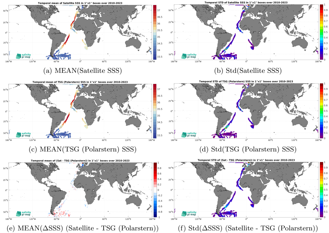
Figure 7: Temporal mean (left) and Std (right) of SSS from CCI SSS L4 Merged-OI v5.5 - 7-day running (ESA) (top), TSG (Polarstern) (middle), and of \Delta SSS (Satellite - TSG (Polarstern)). Only match-up pairs are used to generate these maps.
