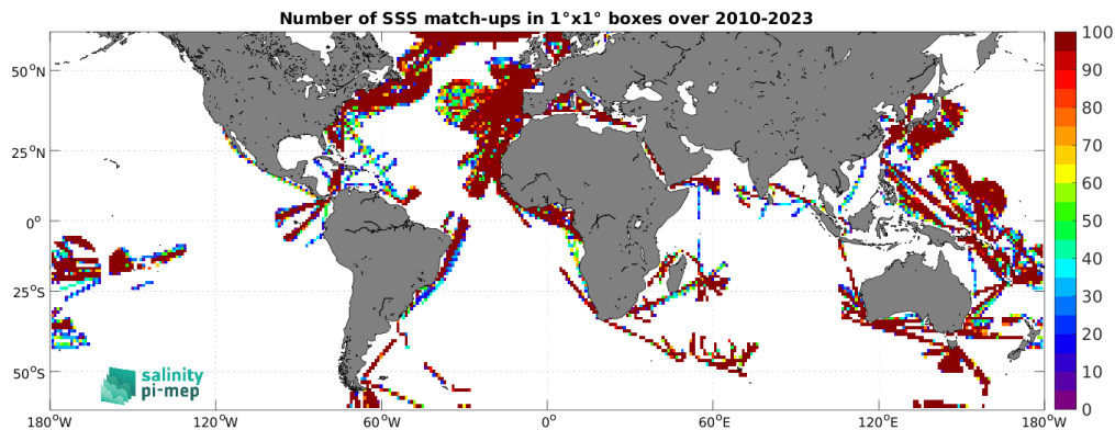
Figure 5: Number of SSS match-ups between TSG (LEGOS-DM) SSS and the CCI SSS L4 Merged-OI v5.5 - 7-day running (ESA) SSS product for the SMOS coastal zone ( <800\text{km} ) 60\text{N} - 60\text{S} Pi-MEP region over 1^\circ \times 1^\circ boxes and for the full satellite product period.
