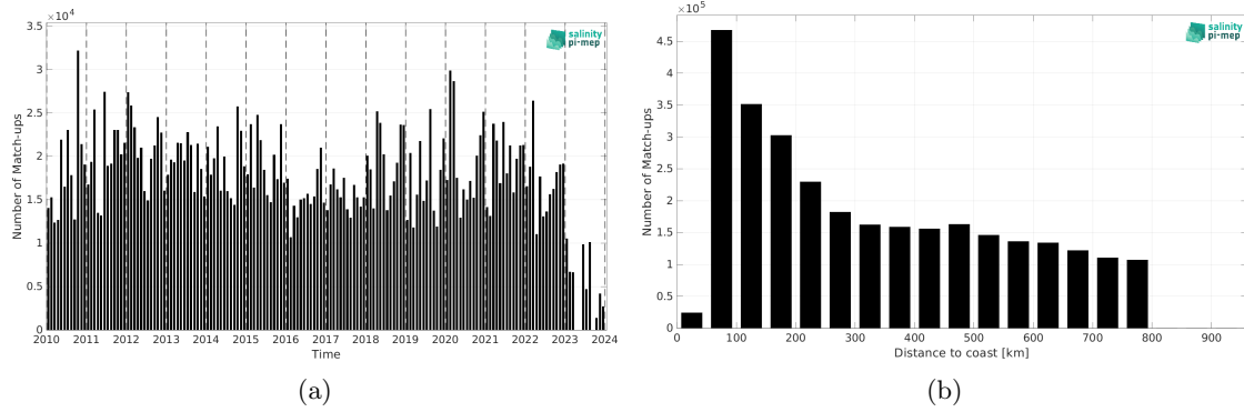
Figure 2: Number of match-ups between TSG (LEGOS-DM) and CCI SSS L4 Merged-OI v5.5 - 7-day running (ESA) SSS as a function of time (a) and as function of the distance to coast (b) over the SMOS coastal zone (<800km) 60N-60S Pi-MEP region and for the full satellite product period.
