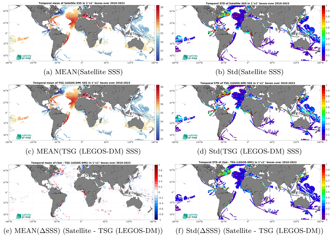
Figure 7: Temporal mean (left) and Std (right) of SSS from CCI SSS L4 Merged-OI v5.5 - 7-day running (ESA) (top), TSG (LEGOS-DM) (middle), and of \Delta SSS (Satellite - TSG (LEGOS-DM)). Only match-up pairs are used to generate these maps.
