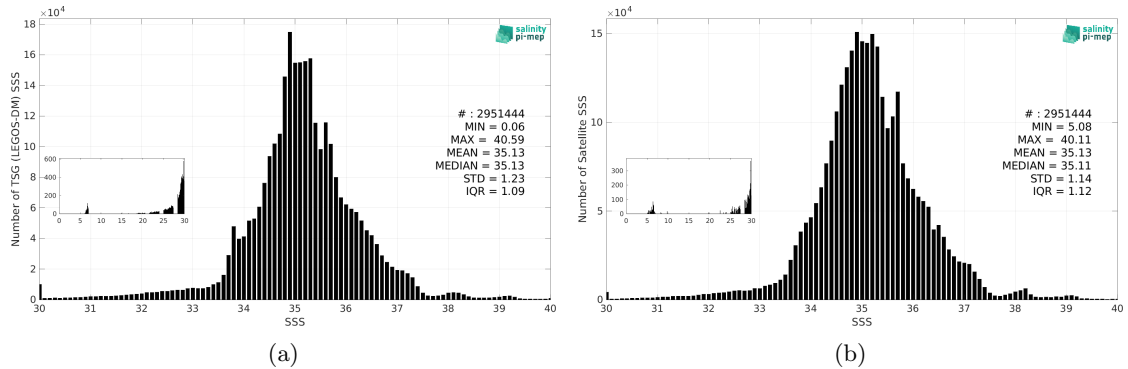
Figure 3: Histograms of SSS from TSG (LEGOS-DM) (a) and CCI SSS L4 Merged-OI v5.5 - 7-day running (ESA) (b) considering all match-up pairs per bins of 0.1 over the SMOS coastal zone (<800km) 60N-60S Pi-MEP region and for the full satellite product period.
