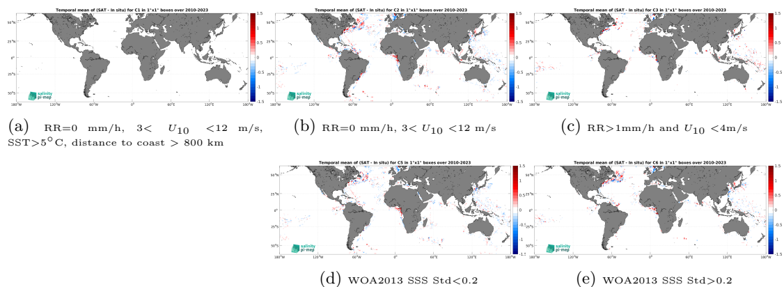
Figure 14: Temporal mean gridded over spatial boxes of size 1^\circ \times 1^\circ of \Delta\text{SSS} (CCI SSS L4 Merged-OI v5.5 - 7-day running (ESA) - TSG (LEGOS-DM)) for 5 different subdatasets corresponding to:RR=0 mm/h, 3 < U_{10} < 12 m/s, SST >5^\circ\text{C} , distance to coast > 800 km (a), RR=0 mm/h, 3 < U_{10} < 12 m/s (b), RR >1 mm/h and U_{10} < 4 m/s (c), WOA2013 SSS Std <0.2 (d), WOA2013 SSS Std >0.2 (e).
