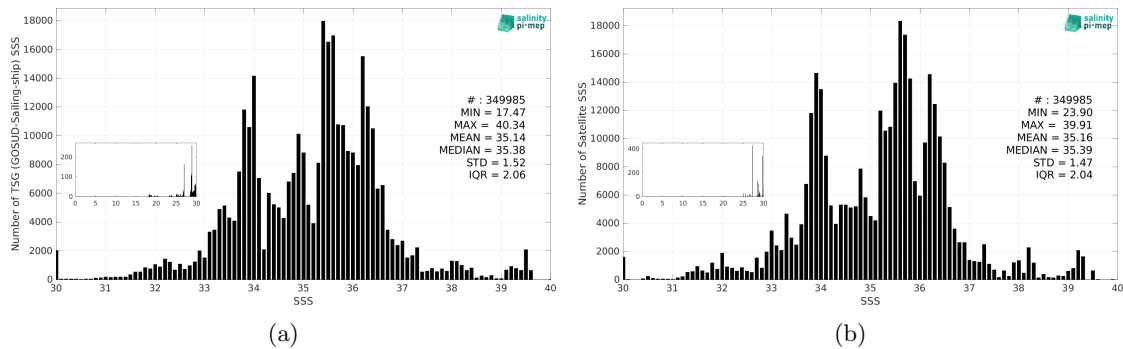
Figure 3: Histograms of SSS from TSG (GOSUD-Sailing-ship) (a) and CCI SSS L4 Merged-OI v5.5 - 7-day running (ESA) (b) considering all match-up pairs per bins of 0.1 over the SMOS coastal zone (<800km) 60N-60S Pi-MEP region and for the full satellite product period.
