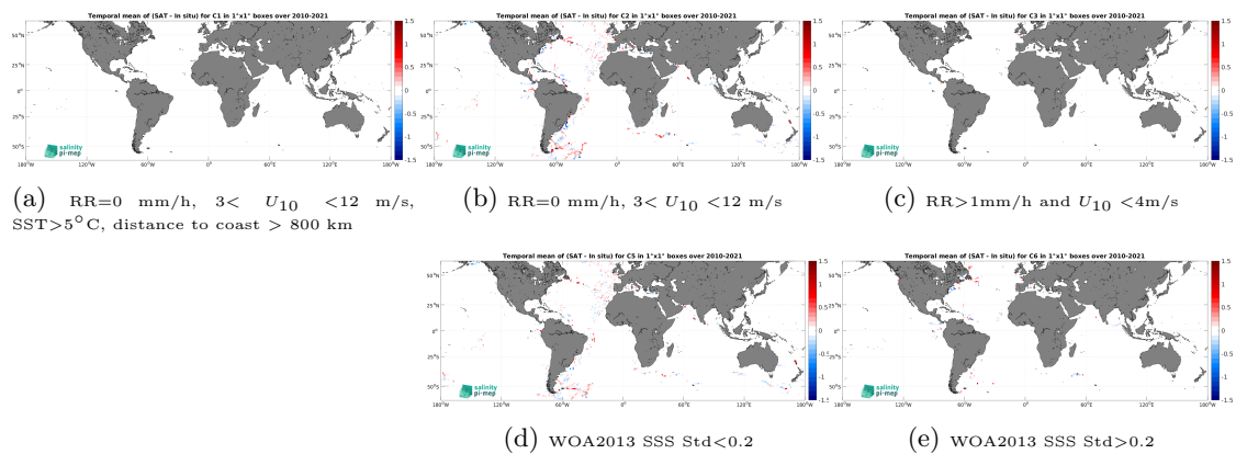
Figure 14: Temporal mean gridded over spatial boxes of size 1^\circ \times 1^\circ of \Delta\text{SSS} (CCI SSS L4 Merged-OI v5.5 - 7-day running (ESA) - TSG (GOSUD-Sailing-ship)) for 5 different subdatasets corresponding to: RR=0 mm/h, 3 < U_{10} < 12 m/s, SST > 5°C, distance to coast > 800 km (a), RR=0 mm/h, 3 < U_{10} < 12 m/s (b), RR > 1mm/h and U_{10} < 4 m/s (c), WOA2013 SSS Std < 0.2 (d), WOA2013 SSS Std > 0.2 (e).
