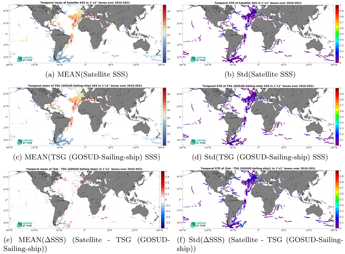
Figure 7: Temporal mean (left) and Std (right) of SSS from CCI SSS L4 Merged-OI v5.5 - 7-day running (ESA) (top), TSG (GOSUD-Sailing-ship) (middle), and of \Delta SSS (Satellite - TSG (GOSUD-Sailing-ship)). Only match-up pairs are used to generate these maps.
