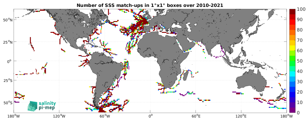
Figure 5: Number of SSS match-ups between TSG (GOSUD-Sailing-ship) SSS and the CCI SSS L4 Merged-OI v5.5 - 7-day running (ESA) SSS product for the SMOS coastal zone (<800km) 60N-60S Pi-MEP region over 1^\circ \times 1^\circ boxes and for the full satellite product period.
