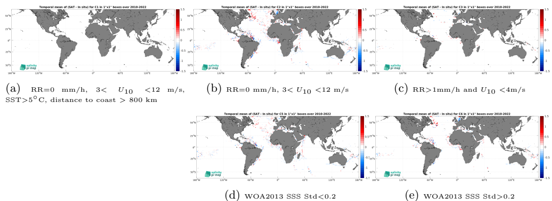
Figure 14: Temporal mean gridded over spatial boxes of size 1^\circ \times 1^\circ of \Delta\text{SSS} (CCI SSS L4 Merged-OI v5.5 - 7-day running (ESA) - TSG (GOSUD-Research-vessel)) for 5 different subdatasets corresponding to:RR=0 mm/h, 3 < U_{10} < 12 m/s, SST>5°C, distance to coast > 800 km (a), RR=0 mm/h, 3 < U_{10} < 12 m/s (b), RR>1mm/h and U_{10} < 4 m/s (c), WOA2013 SSS Std<0.2 (d), WOA2013 SSS Std>0.2 (e).
