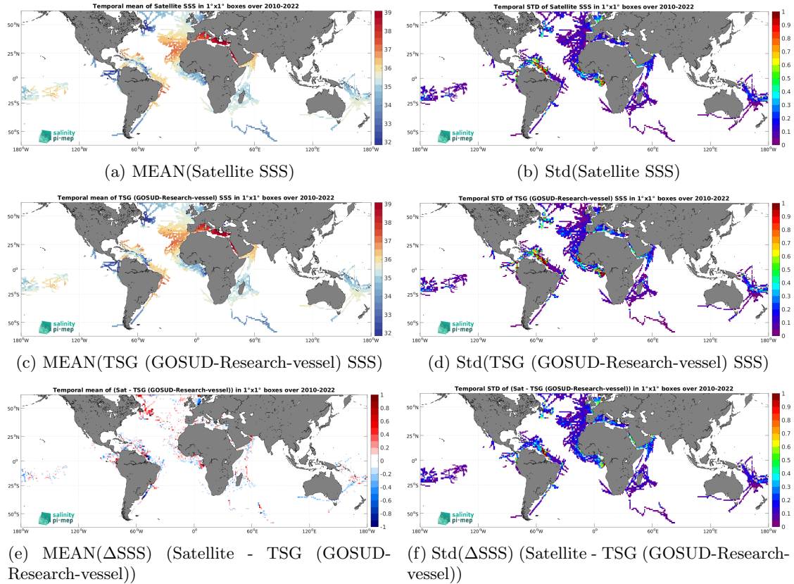
Figure 7: Temporal mean (left) and Std (right) of SSS from CCI SSS L4 Merged-OI v5.5 - 7-day running (ESA) (top), TSG (GOSUD-Research-vessel) (middle), and of \Delta SSS (Satellite - TSG (GOSUD-Research-vessel)). Only match-up pairs are used to generate these maps.
