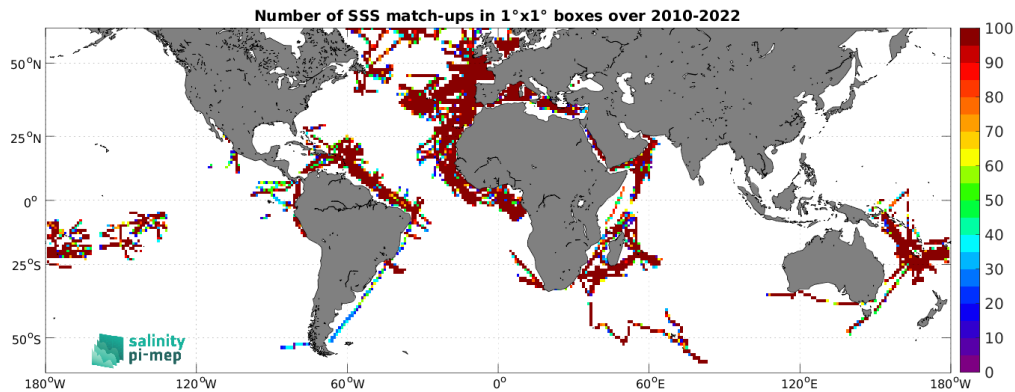
Figure 5: Number of SSS match-ups between TSG (GOSUD-Research-vessel) SSS and the CCI SSS L4 Merged-OI v5.5 - 7-day running (ESA) SSS product for the SMOS coastal zone (<800km) 60N-60S Pi-MEP region over 1^\circ \times 1^\circ boxes and for the full satellite product period.
