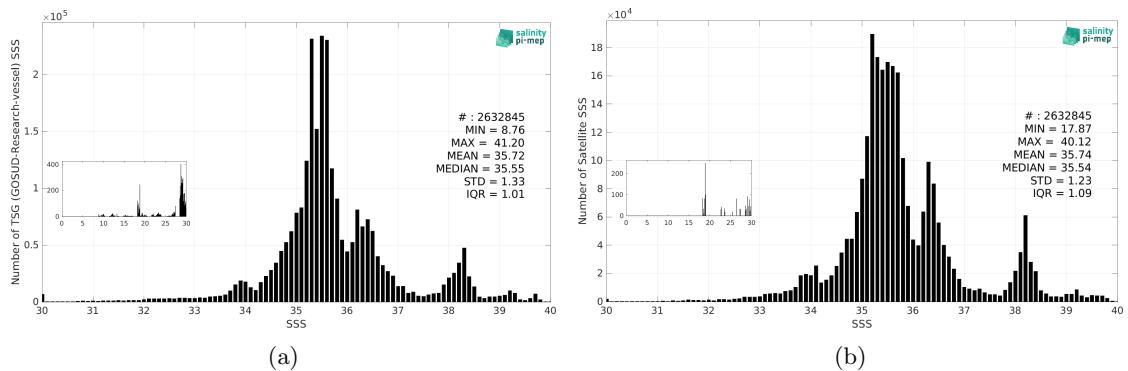
Figure 3: Histograms of SSS from TSG (GOSUD-Research-vessel) (a) and CCI SSS L4 Merged-OI v5.5 - 7-day running (ESA) (b) considering all match-up pairs per bins of 0.1 over the SMOS coastal zone (<800km) 60N-60S Pi-MEP region and for the full satellite product period.
