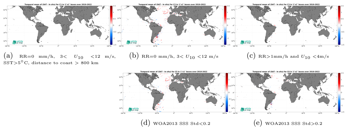
Figure 14: Temporal mean gridded over spatial boxes of size 1^\circ \times 1^\circ of \Delta\text{SSS} (CCI SSS L4 Merged-OI v5.5 - 7-day running (ESA) - TSG (CSIC-UTM)) for 5 different subdatasets corresponding to:RR=0 mm/h, 3 < U_{10} < 12 m/s, SST>5°C, distance to coast > 800 km (a), RR=0 mm/h, 3 < U_{10} < 12 m/s (b), RR>1mm/h and U_{10} < 4 m/s (c), WOA2013 SSS Std<0.2 (d), WOA2013 SSS Std>0.2 (e).
