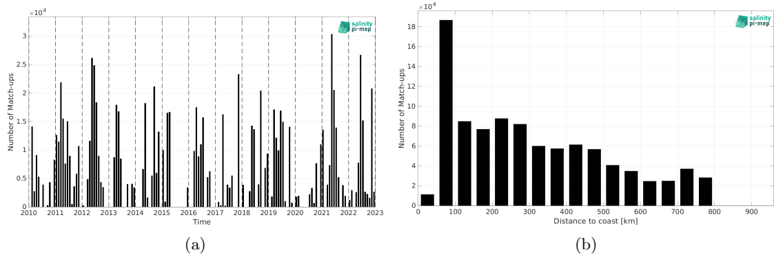
Figure 2: Number of match-ups between TSG (CSIC-UTM) and CCI SSS L4 Merged-OI v5.5 - 7-day running (ESA) SSS as a function of time (a) and as function of the distance to coast (b) over the SMOS coastal zone (<800km) 60N-60S Pi-MEP region and for the full satellite product period.
