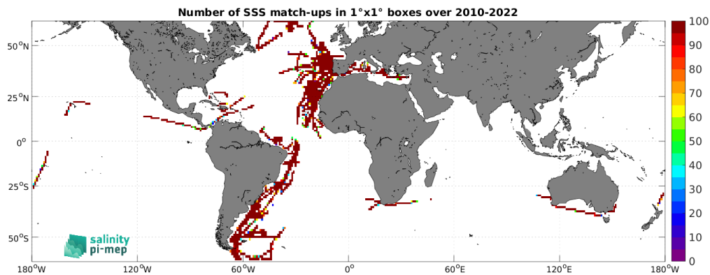
Figure 5: Number of SSS match-ups between TSG (CSIC-UTM) SSS and the CCI SSS L4 Merged-OI v5.5 - 7-day running (ESA) SSS product for the SMOS coastal zone (<800km) 60N-60S Pi-MEP region over 1^\circ \times 1^\circ boxes and for the full satellite product period.
