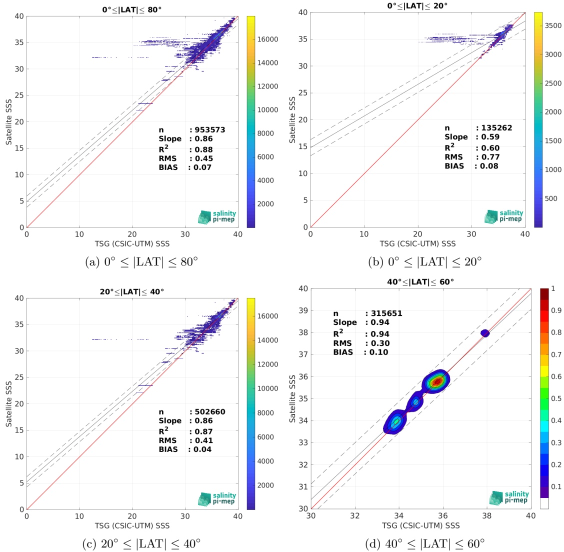
Figure 10: Contour maps of the concentration of CCI SSS L4 Merged-OI v5.5 - 7-day running (ESA) SSS (y-axis) versus TSG (CSIC-UTM) SSS (x-axis) at match-up pairs for different latitude bands. For each plot, the red line shows x=y . The black thin and dashed lines indicate a linear fit through the data cloud and the \pm 95\% confidence levels, respectively. The number match-up pairs n , the slope and R^2 coefficient of the linear fit, the root mean square (RMS) and the mean bias between satellite and in situ data are indicated for each latitude band in each plots.
