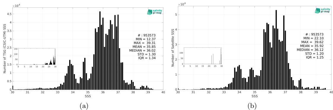
Figure 3: Histograms of SSS from TSG (CSIC-UTM) (a) and CCI SSS L4 Merged-OI v5.5 - 7-day running (ESA) (b) considering all match-up pairs per bins of 0.1 over the SMOS coastal zone (<800km) 60N-60S Pi-MEP region and for the full satellite product period.
