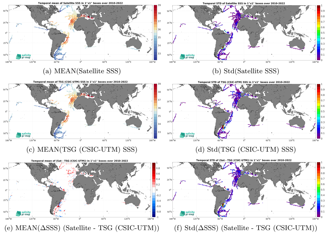
Figure 7: Temporal mean (left) and Std (right) of SSS from CCI SSS L4 Merged-OI v5.5 - 7-day running (ESA) (top), TSG (CSIC-UTM) (middle), and of \Delta SSS (Satellite - TSG (CSIC-UTM)). Only match-up pairs are used to generate these maps.
