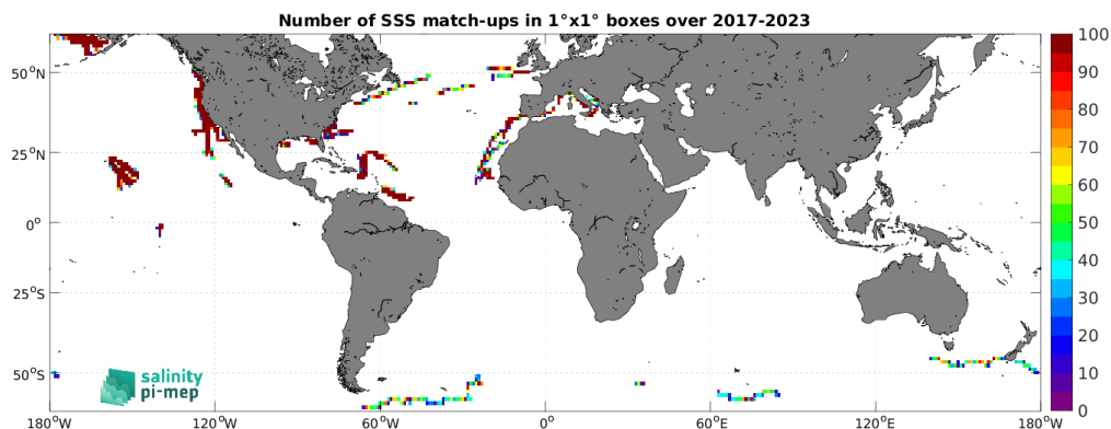
Figure 5: Number of SSS match-ups between Saildrone SSS and the CCI SSS L4 Merged-OI v5.5 - 7-day running (ESA) SSS product for the SMOS coastal zone (<800km) 60N-60S Pi-MEP region over 1^\circ \times 1^\circ boxes and for the full satellite product period.
