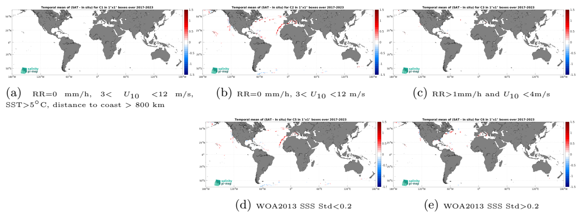
Figure 14: Temporal mean gridded over spatial boxes of size 1^\circ \times 1^\circ of \Delta SSS (CCI SSS L4 Merged-OI v5.5 - 7-day running (ESA) - Saildrone) for 5 different subdatasets corresponding to:RR=0 mm/h, 3 < U_{10} < 12 m/s, SST >5^\circ\text{C} , distance to coast > 800 km (a), RR=0 mm/h, 3 < U_{10} < 12 m/s (b), RR >1 mm/h and U_{10} < 4 m/s (c), WOA2013 SSS Std <0.2 (d), WOA2013 SSS Std >0.2 (e).
