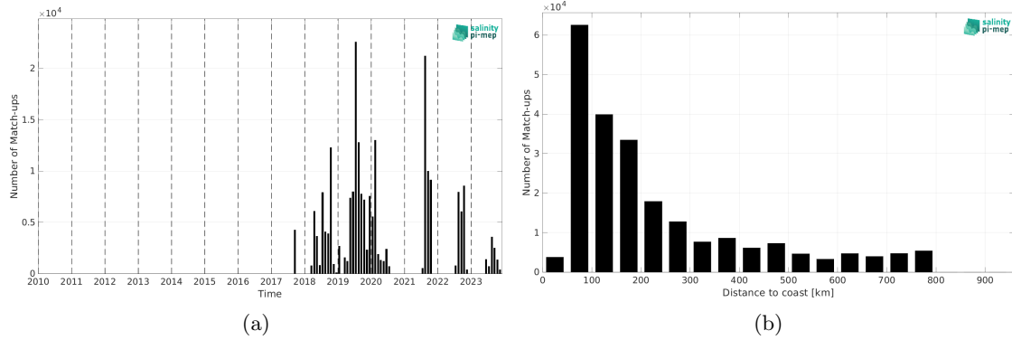
Figure 2: Number of match-ups between Saildrone and CCI SSS L4 Merged-OI v5.5 - 7-day running (ESA) SSS as a function of time (a) and as function of the distance to coast (b) over the SMOS coastal zone (<800km) 60N-60S Pi-MEP region and for the full satellite product period.
