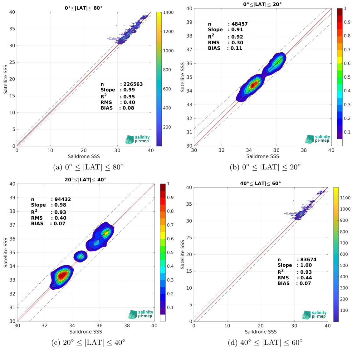
Figure 10: Contour maps of the concentration of CCI SSS L4 Merged-OI v5.5 - 7-day running (ESA) SSS (y-axis) versus Saitdrone SSS (x-axis) at match-up pairs for different latitude bands. For each plot, the red line shows x=y . The black thin and dashed lines indicate a linear fit through the data cloud and the \pm 95\% confidence levels, respectively. The number match-up pairs n , the slope and R^2 coefficient of the linear fit, the root mean square (RMS) and the mean bias between satellite and in situ data are indicated for each latitude band in each plots.
