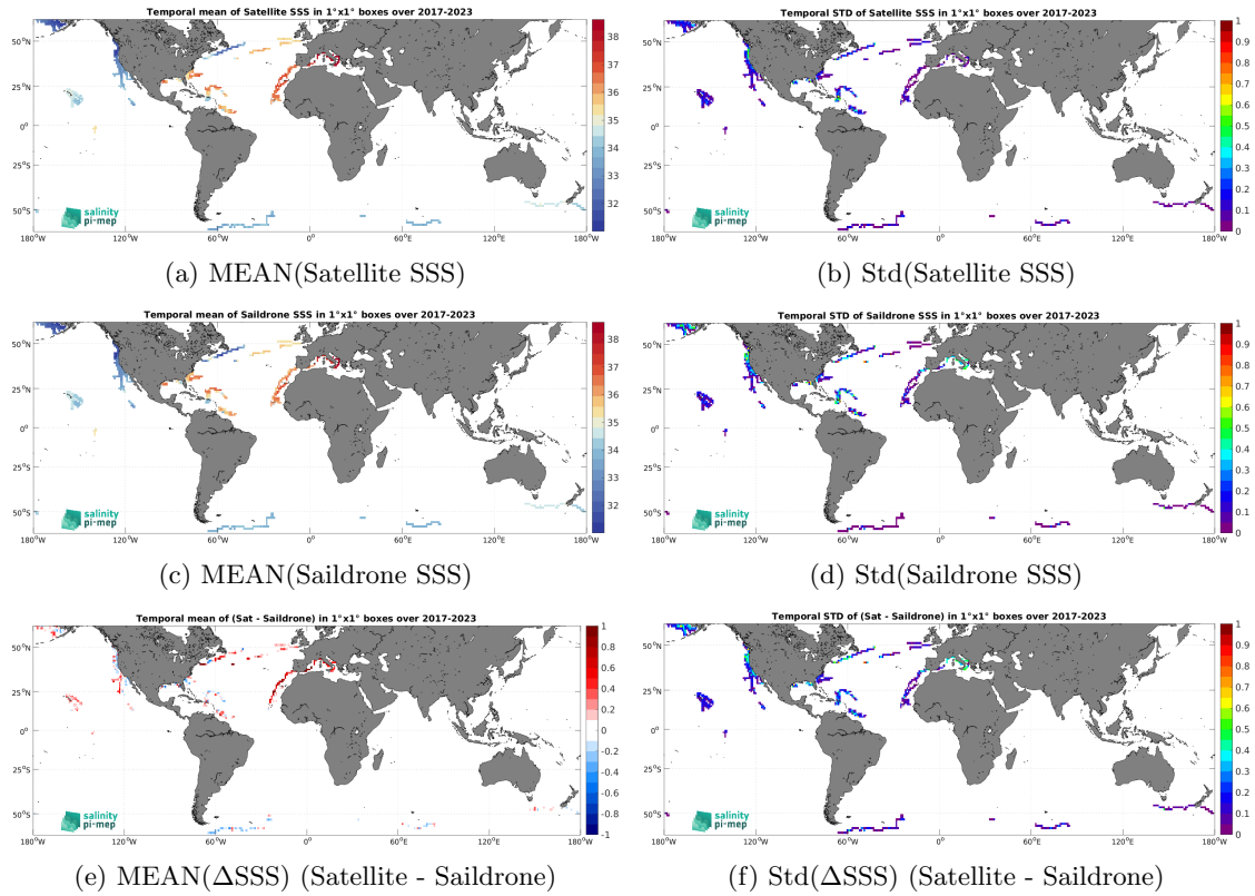
Figure 7: Temporal mean (left) and Std (right) of SSS from CCI SSS L4 Merged-OI v5.5 - 7-day running (ESA) (top), Saildrone (middle), and of \Delta SSS (Satellite - Saildrone). Only match-up pairs are used to generate these maps.
