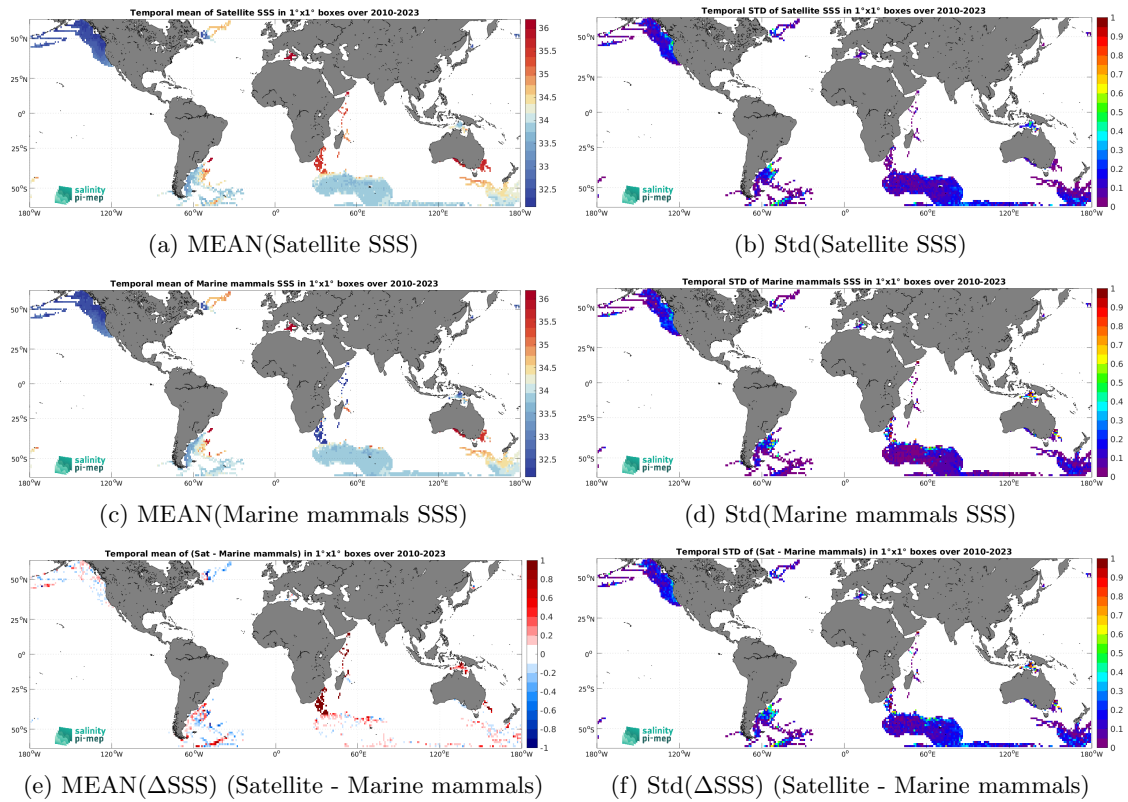
Figure 7: Temporal mean (left) and Std (right) of SSS from CCI SSS L4 Merged-OI v5.5 - 7-day running (ESA) (top), Marine mammals (middle), and of \Delta SSS (Satellite - Marine mammals). Only match-up pairs are used to generate these maps.
