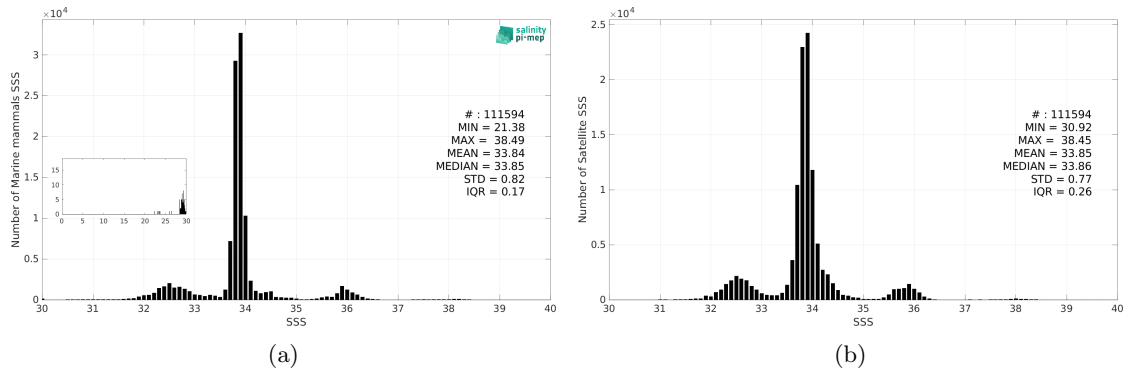
Figure 3: Histograms of SSS from Marine mammals (a) and CCI SSS L4 Merged-OI v5.5 - 7-day running (ESA) (b) considering all match-up pairs per bins of 0.1 over the SMOS coastal zone (<800km) 60N-60S Pi-MEP region and for the full satellite product period.
