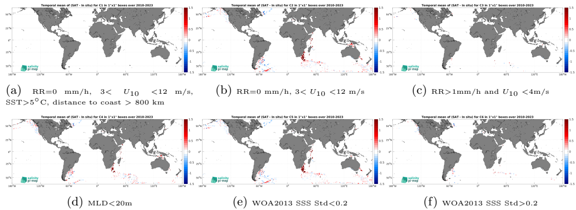
Figure 14: Temporal mean gridded over spatial boxes of size 1^\circ \times 1^\circ of \Delta SSS (CCI SSS L4 Merged-OI v5.5 - 7-day running (ESA) - Marine mammals) for 6 different subdatasets corresponding to:RR=0 mm/h, 3 < U_{10} < 12 m/s, SST >5^\circ C, distance to coast > 800 km (a), RR=0 mm/h, 3 < U_{10} < 12 m/s (b), RR >1 mm/h and U_{10} < 4 m/s (c),MLD <20 m (d),WOA2013 SSS Std <0.2 (e),WOA2013 SSS Std >0.2 (f).
