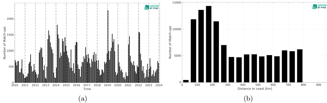
Figure 2: Number of match-ups between Marine mammals and CCI SSS L4 Merged-OI v5.5 - 7-day running (ESA) SSS as a function of time (a) and as function of the distance to coast (b) over the SMOS coastal zone (<800km) 60N-60S Pi-MEP region and for the full satellite product period.
