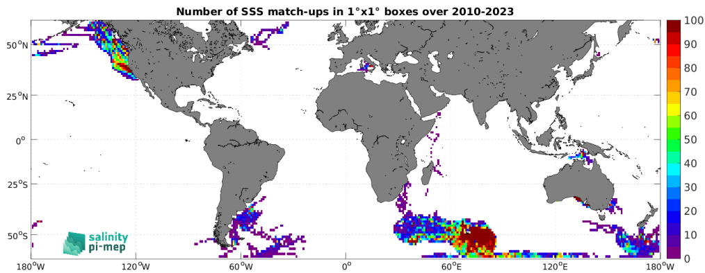
Figure 5: Number of SSS match-ups between Marine mammals SSS and the CCI SSS L4 Merged-OI v5.5 - 7-day running (ESA) SSS product for the SMOS coastal zone (<800km) 60N-60S Pi-MEP region over 1^\circ \times 1^\circ boxes and for the full satellite product period.
